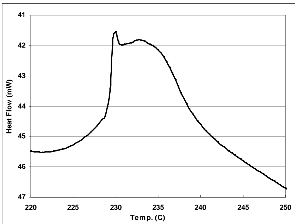
Figure 5. High temperature DSC scan of damp, spherical RF resin after contact with 3 M HNO 3 acid at 25 °C for 24 hours (scan rate: 10 °C/ min).
