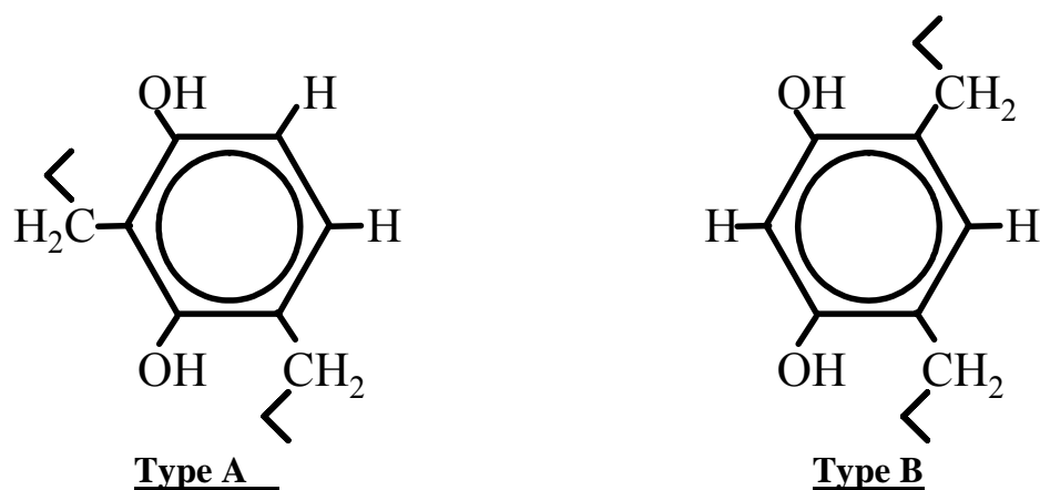
Figure 1. Primary structural types within resorcinol formaldehyde polymer.
