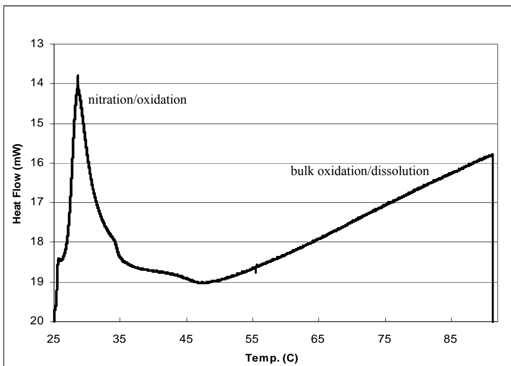
Figure 2. Differential scanning calorimetry data for spherical RF resin in 3 M nitric acid (scan rate: 0.1 °C/min).
