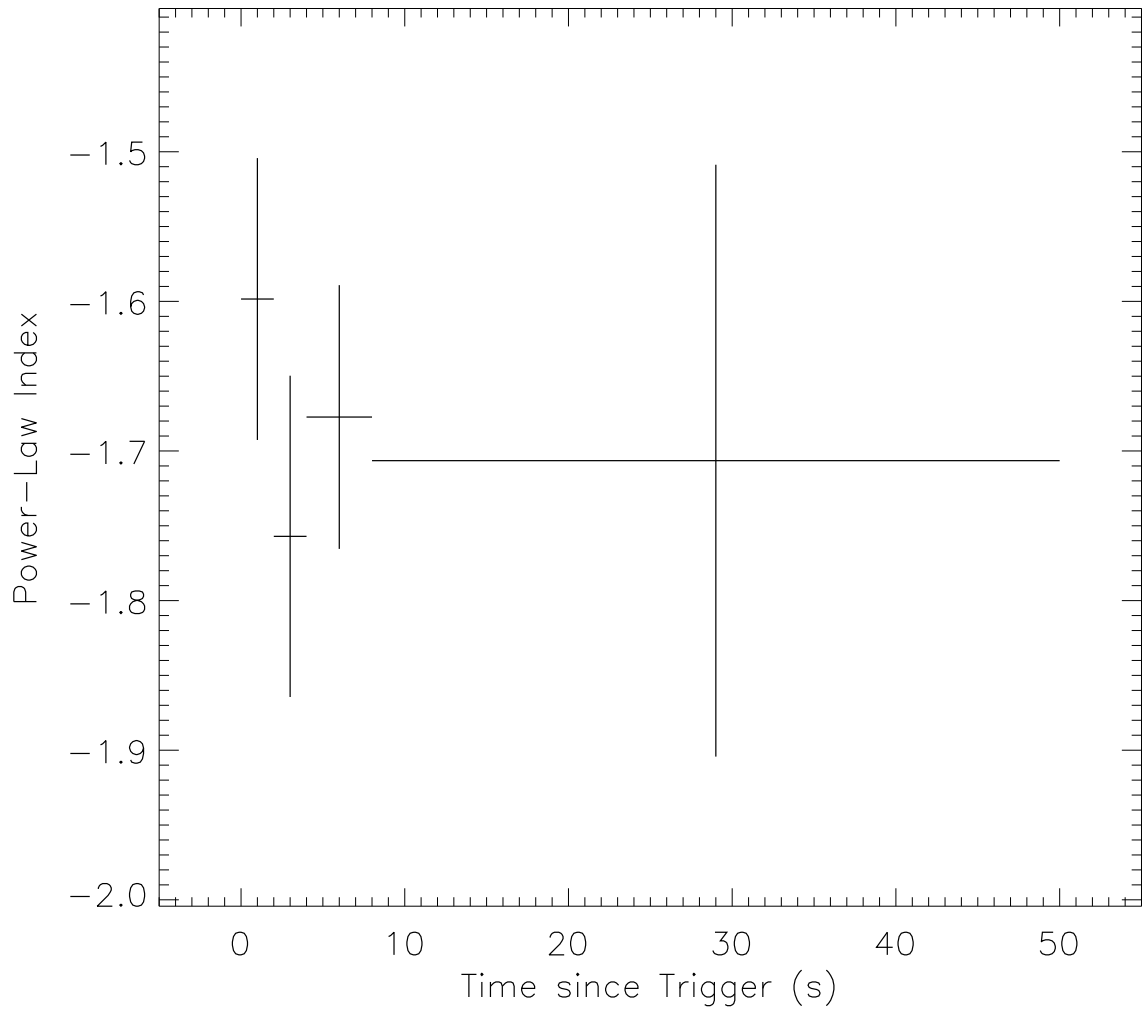
Fig. 5.— Single power law spectral index evolution of GRB031203; the data points correspond to the intervals indicated in Figure 4.
