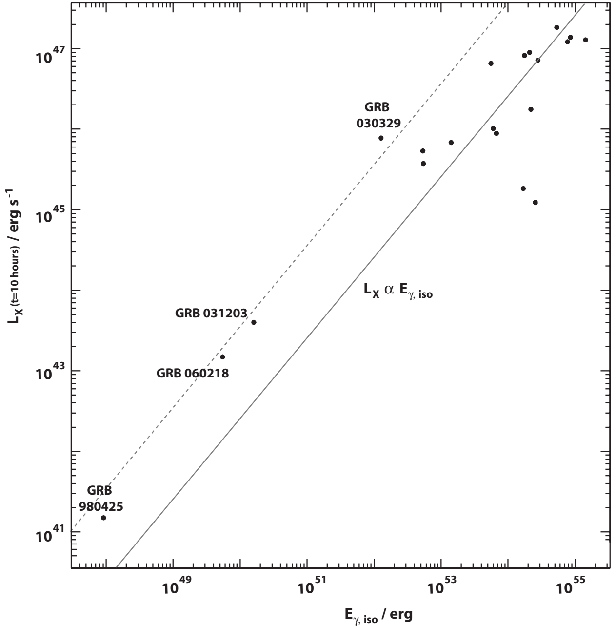
Fig. 20.— Isotropic-equivalent luminosity of SN-GRB X-ray afterglows scaled to t = 10 hr (source frame) after the burst trigger as a function of their isotropic \gamma -ray energy release (adopted from Kouveliotou et al. 2004).
