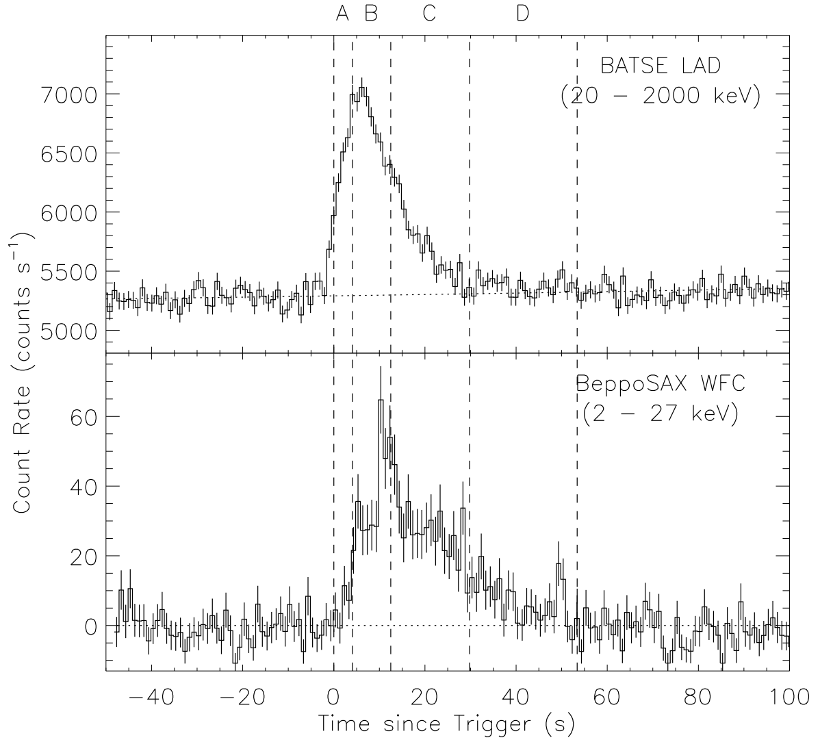
Fig. 1.— Lightcurves of GRB 980425 detected with the brightest BATSE LAD (20–2000 keV; top ) and with the BeppoSAX WFC (2–27 keV; bottom ) plotted with 1-s resolution. The four time intervals used in the current analysis are labeled with A, B, C, and D. The dotted lines indicate background levels.
