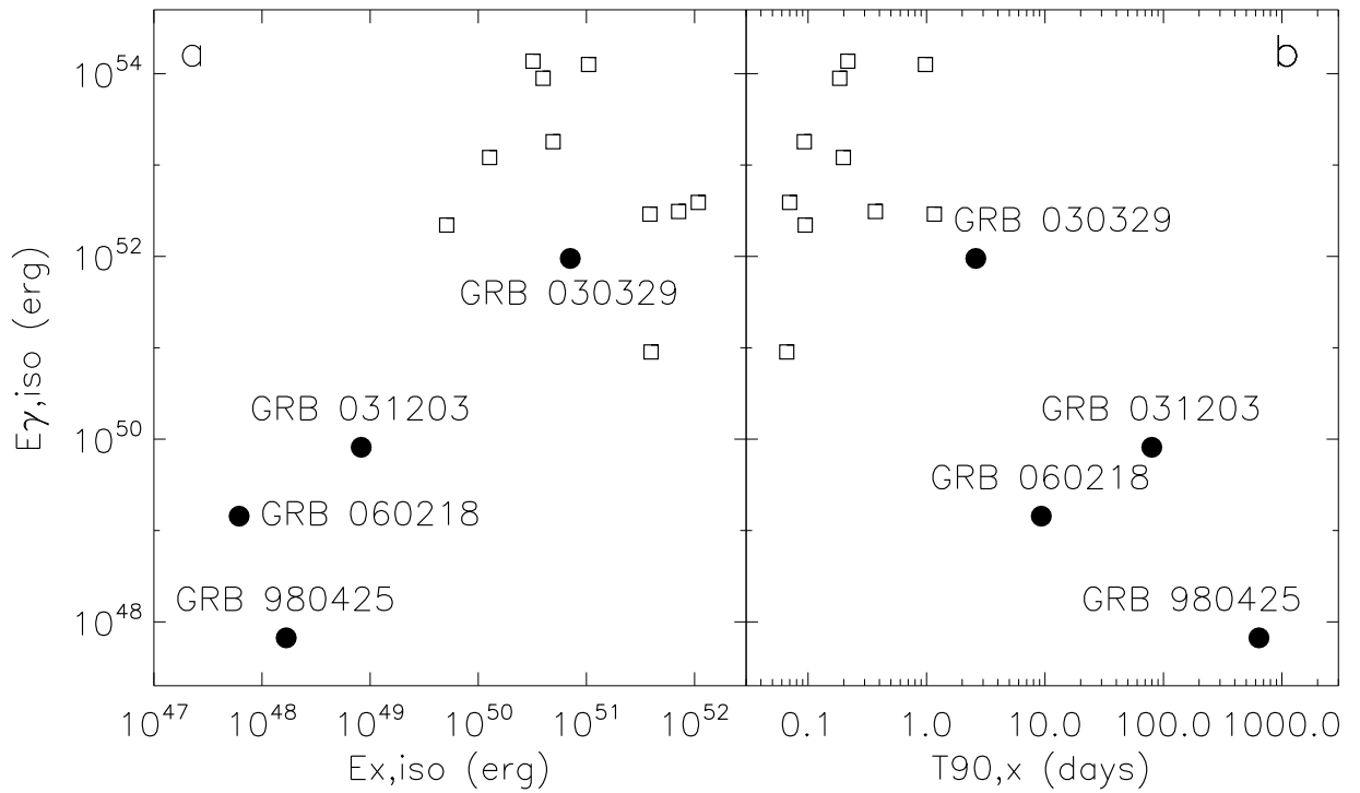
Fig. 16.— Comparison of the four SN-GRBs (full circles) with the 10 Swift GRBs presented by Nousek et al. (2006) (squares), in the E_{\gamma,iso} - E_{X,iso} plane (a) and in the E_{\gamma,iso} - T_{90,x} plane (b). The E_{\gamma,iso} values used here are determined between 20–2000 keV in the source frame.
