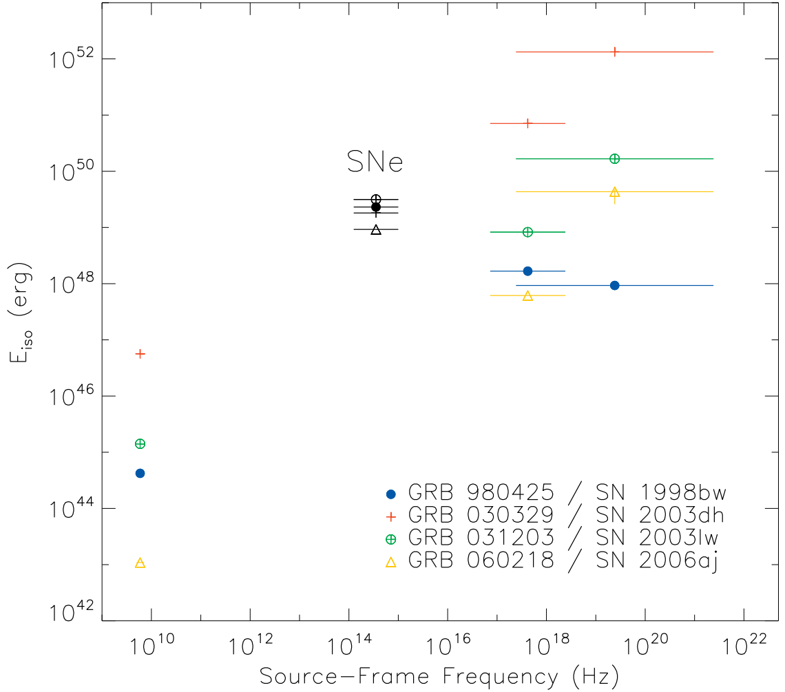
Fig. 22.— Summary of the isotropic-equivalent total emitted energy of the prompt and afterglow emission of the four GRBs, along with the properties of their associated SNe. The energetics in \gamma -ray, X-ray, Radio, and Optical (for SNe) wavelengths correspond to 1–10,000 keV, 0.3–10 keV, 5–7 GHz, 3000–24000 Å in the source frame, respectively.
