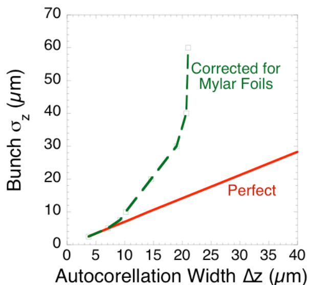
Figure 4: Bunch length as expected from a perfect autocorrelation trace (continuous red line) and corrected for the Mylar foils reflection and transmission (dashed green line). The calculations are done with Gaussian bunch shapes.
