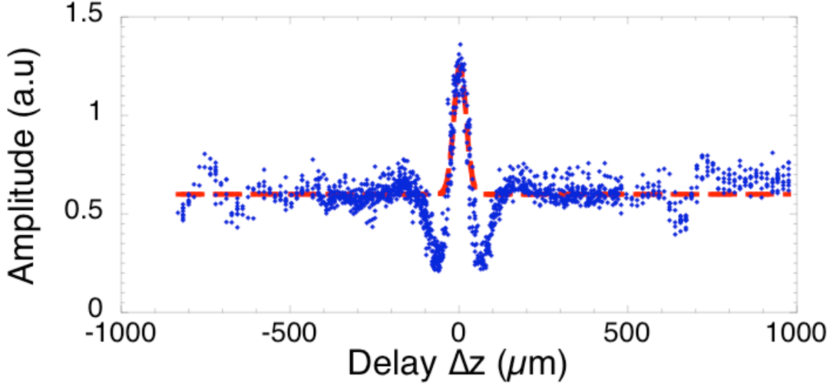
Figure 1: CTR amplitude versus delay of the movable interferometer arm \Delta z showing the electron bunch autocorrelation trace. The blue diamonds show the measured data points, the red dashed line is the Gaussian fit to the trace peak. Note that the trace was obtained from multiple scans with various \Delta z steps.
