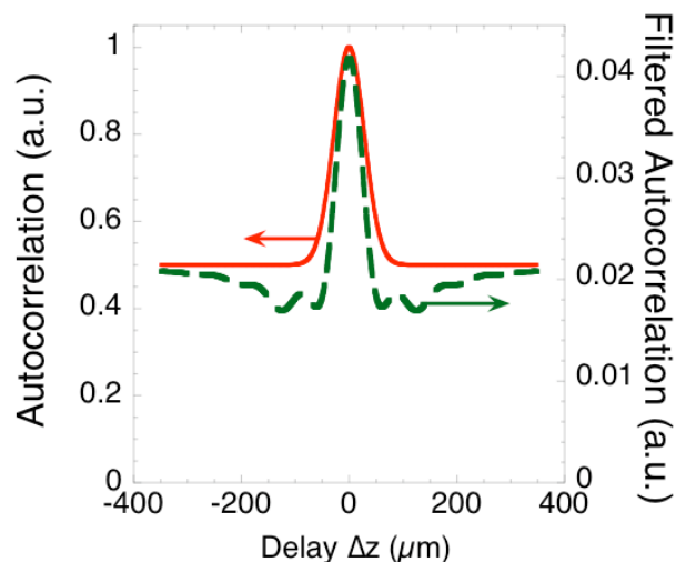
Figure 3: Autocorrelation traces ( C(\tau) in the text) calculated without (continuous red line) and with (dashed green line) the effect of the Mylar foils.
