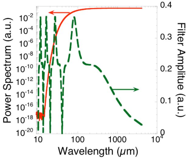
Figure 2: Power spectrum for the CTR of a Gaussian bunch with \sigma_z=20 \mu\text{m} (red continuous line) and total transmission spectrum (dashed green line) for the three Mylar foils (see text).
