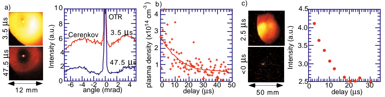
FIG. 4. Downstream foil data are shown for two wavelength ranges: (a-b) 676.4 nm (1.35 m oven) and (c) 505 nm (1 m oven). a) Images at high (3.5 \mu s delay) and low (47.5 \mu s) plasma density. Lineouts show inward shift of Cerenkov cone and increase in visible background level. b) Plasma density estimated from inward shift of Cerenkov cone angle vs. delay c) Images at \Delta t < 0 and 2.5 \mu s delay show spatial extent (limited by 2 in. pellicle aperture) of background; total intensity collected into 80 nm BW vs. delay.
