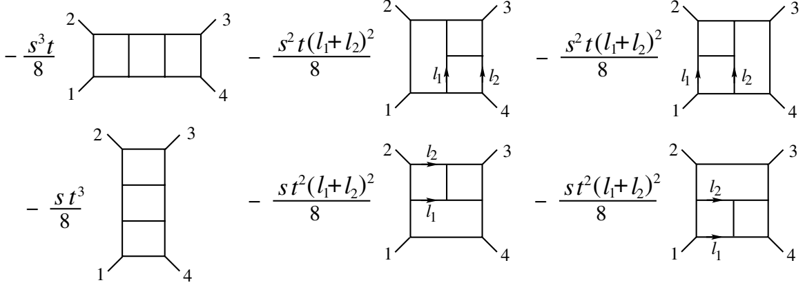
FIG. 3: Mondrian diagrams for the three-loop four-point MSYM planar amplitude given in eq. (2.5). The second and third diagrams have identical values as do the fifth and sixth. The factors of (l_1 + l_2)^2 denotes numerator factors appearing in the integrals, where l_1 and l_2 are the momenta carried by the lines marked by arrows.
