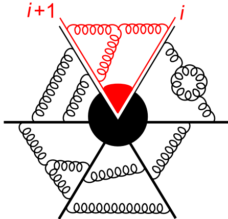
FIG. 5: Infrared structure of leading-color scattering amplitudes for particles in the adjoint representation. The straight lines represent hard external states, while the curly lines carry soft or collinear virtual momenta. At leading color, soft exchanges are confined to wedges between the hard lines.
