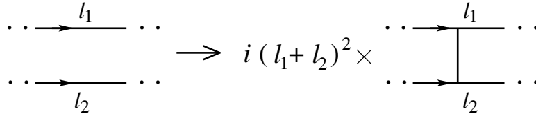
FIG. 2: The rung insertion rule for generating higher-loop integrands from lower loop ones, given in ref. [7].
