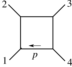
FIG. 6: The one-loop box integral.
