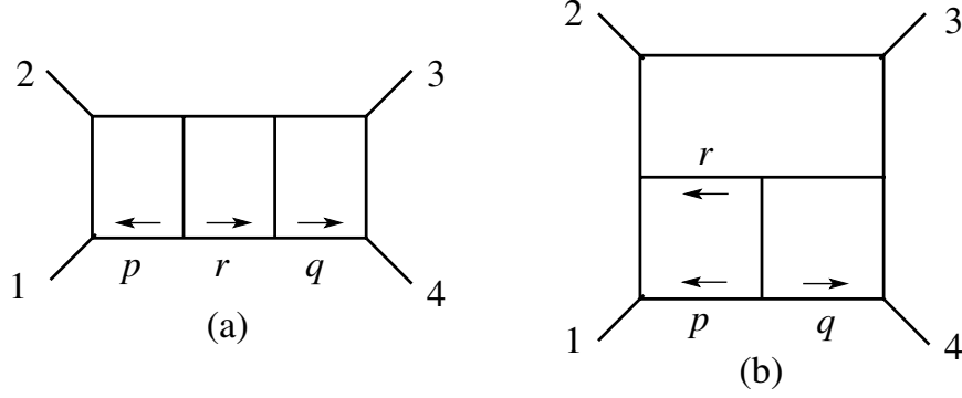
FIG. 4: The two integrals appearing in the three-loop amplitude. The “ladder” integral (a) has no factors in the numerator. The “tennis court” integral (b) contains a factor of (p+r)^2 in the numerator.
