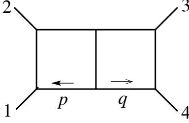
FIG. 7: The two-loop double-box integral.
