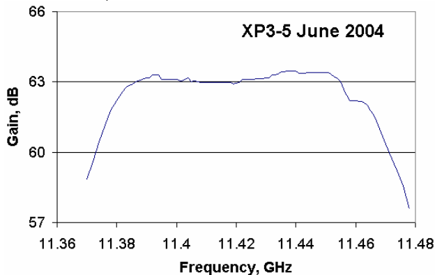
Figure 6: 3 dB bandwidth at a constant 10 MW.
