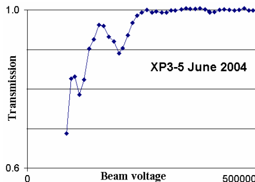
Figure 2: Typical PPM klystron beam transmission data.
