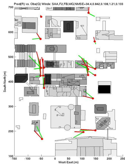
Fig. 6. Comparison of predicted wind vectors (red arrows) against 30-min average data (green arrows) measured by DPG PWIDS on z=8 m plane for IOP 8.
