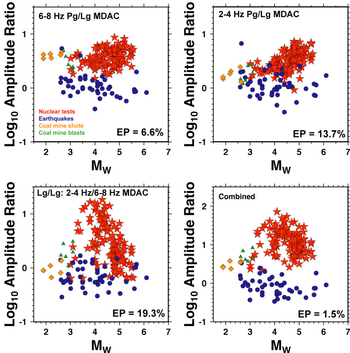
Figure 3. We show nuclear explosion discrimination from earthquake performance at station KNB for 3 different regional phase ratios after MDAC corrections were applied. In the lower right we combine these 3 ratios using an optimal set of weights determined using LDA to get a dramatic increase in performance. The combination is 0.71 (6-8Hz Pg/Lg) + 0.88 (2-4 Hz Pg/Lg) + 0.57 (2-4/6-8 Hz Lg/Lg). This shows how optimally combining even mediocre discriminants can improve performance of very good discriminants because new information always helps. Note the mine shots track the nuclear tests for the P/S ratios but not the low to high Lg ratio. Using the mine shots to obtain LDA weights would degrade the nuclear explosion discrimination performance.
