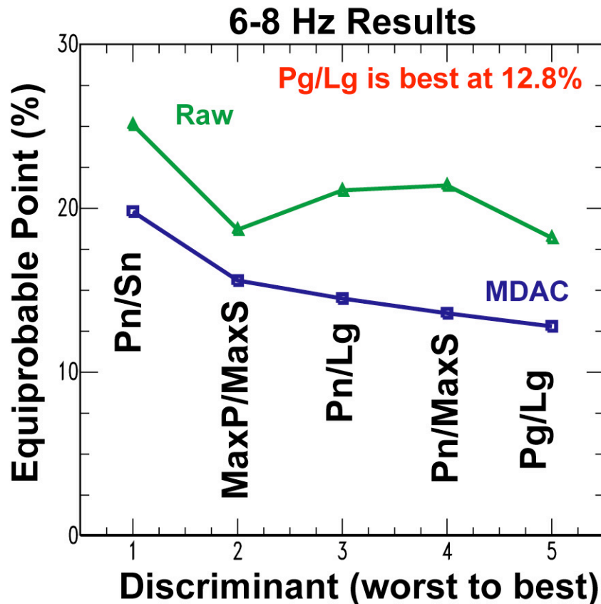
Figure 7. We combined data from 4 stations (CMB, ELK, KNB, LAC) to evaluate discriminant performance using equiprobable value as a metric. Equiprobable value is the level when the earthquake and explosion misidentification rates are equal, so the lower the number the better. We tried a variety of 6-8 Hz measures including taking the Max (Pn, Pg) and Max (Sn, Lg) and found Pg/Lg does the best. Note that the MDAC corrections significantly improve performance for all discriminants.
