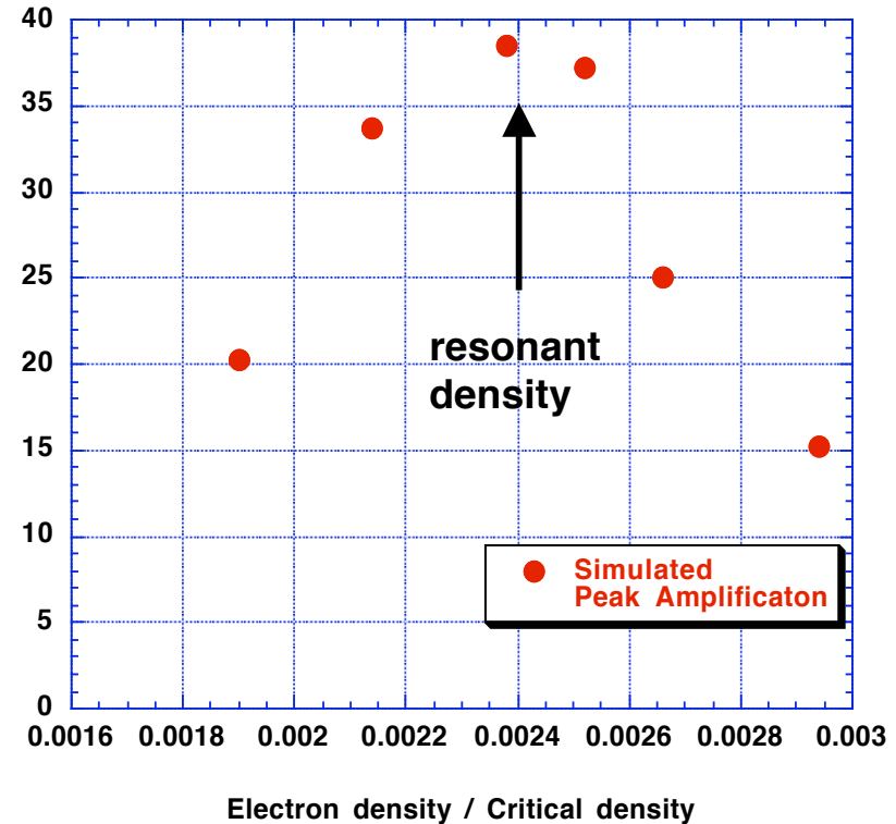
Power Amplification Vs. Density
