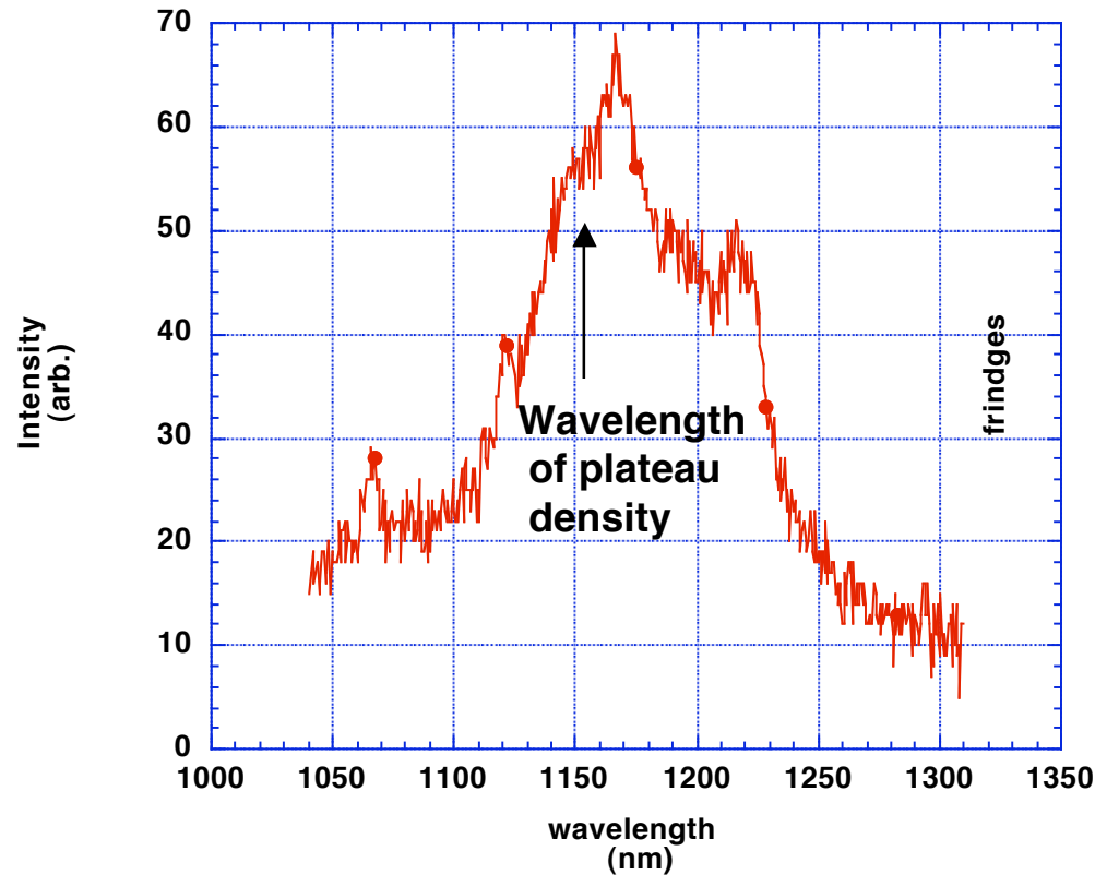
SRS Spectrum
