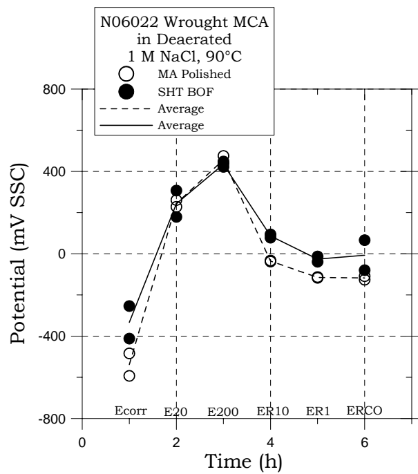
FIGURE 6 – Parameters from CPP for MA and SHT Alloy 22 in 1 M NaCl at 90°C
