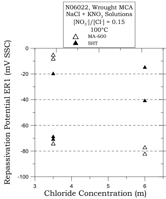
FIGURE 9 – ER1 for MA and SHT Alloy 22 Specimens in NaCl + KNO 3 solutions for a Nitrate over Chloride ratio of 0.15
