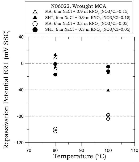
FIGURE 7 – ER1 for MA and SHT Alloy 22 Specimens in 6 m NaCl + 0.9 m KNO 3
