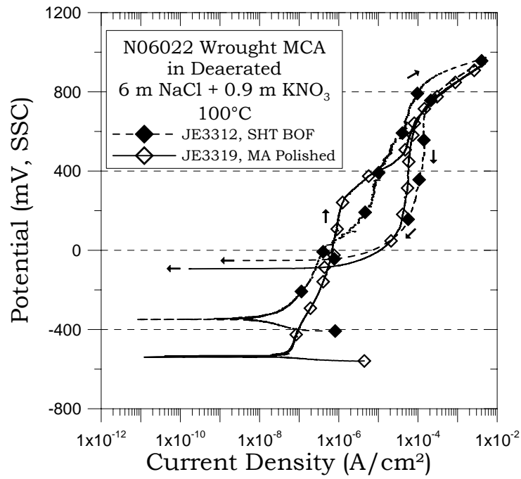
FIGURE 5 – CPP for MA and SHT Alloy 22 Specimens in 6 m NaCl + 0.9 m KNO 3 at 100°C
