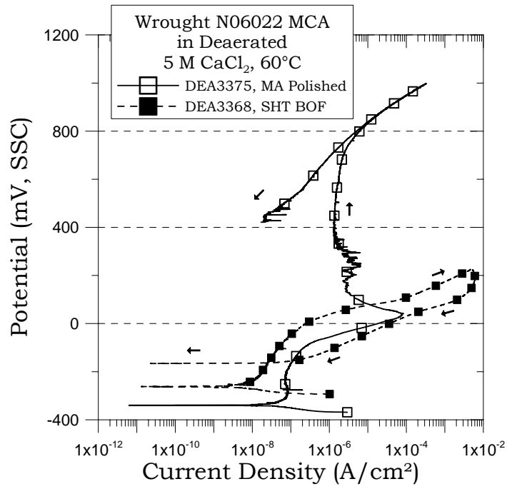
FIGURE 3 – Cyclic Potentiodynamic Polarization (CPP) for MA and SHT Alloy 22 Specimens in 5 M CaCl 2 at 60°C
