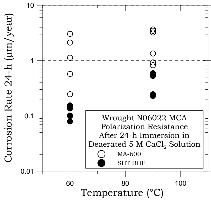
FIGURE 1 – CR for MA and SHT Alloy 22 Specimens in 5 M CaCl 2
