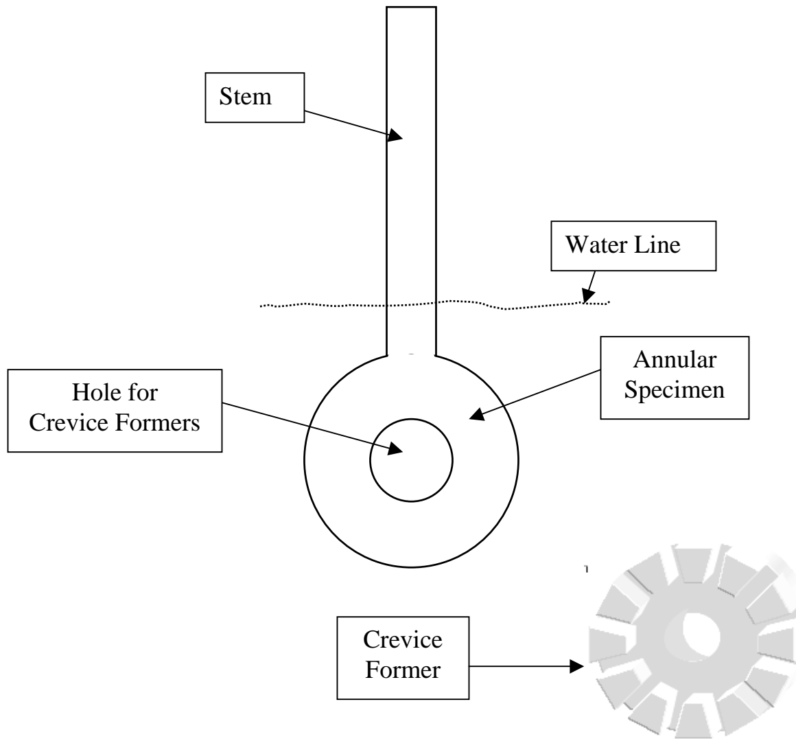
FIGURE 1 – Multiple Crevice Assembly (MCA) Specimen and Crevice Former (CF). Further photographs of the corroded specimens generally correspond to one quarter of the tested surface.
