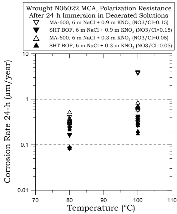
FIGURE 2 – CR for MA and SHT Alloy 22 Specimens in NaCl + KNO 3 Solutions
