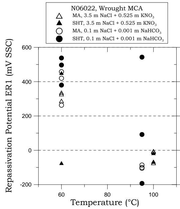
FIGURE 8 – ER1 for MA and SHT Alloy 22 Specimens in 3.5 m NaCl + 0.525 m KNO 3 and 0.1 m NaCl + 0.001 m NaHCO 3
