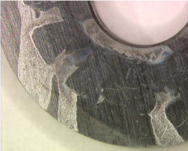
FIGURE 14 – Specimen JE3376, MA polished Alloy 22 after CPP in 5 M CaCl 2 at 90°C
