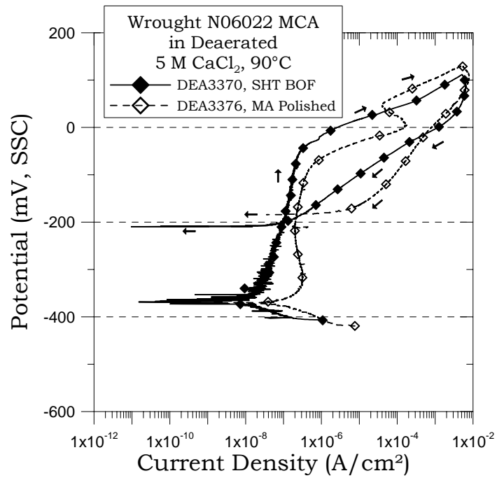
FIGURE 4 – CPP for MA and SHT Alloy 22 Specimens in 5 M CaCl 2 at 90°C
