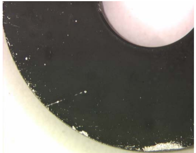
FIGURE 15 – Specimen JE3370, SHT Alloy 22 after CPP in 5 M CaCl 2 at 90°C
