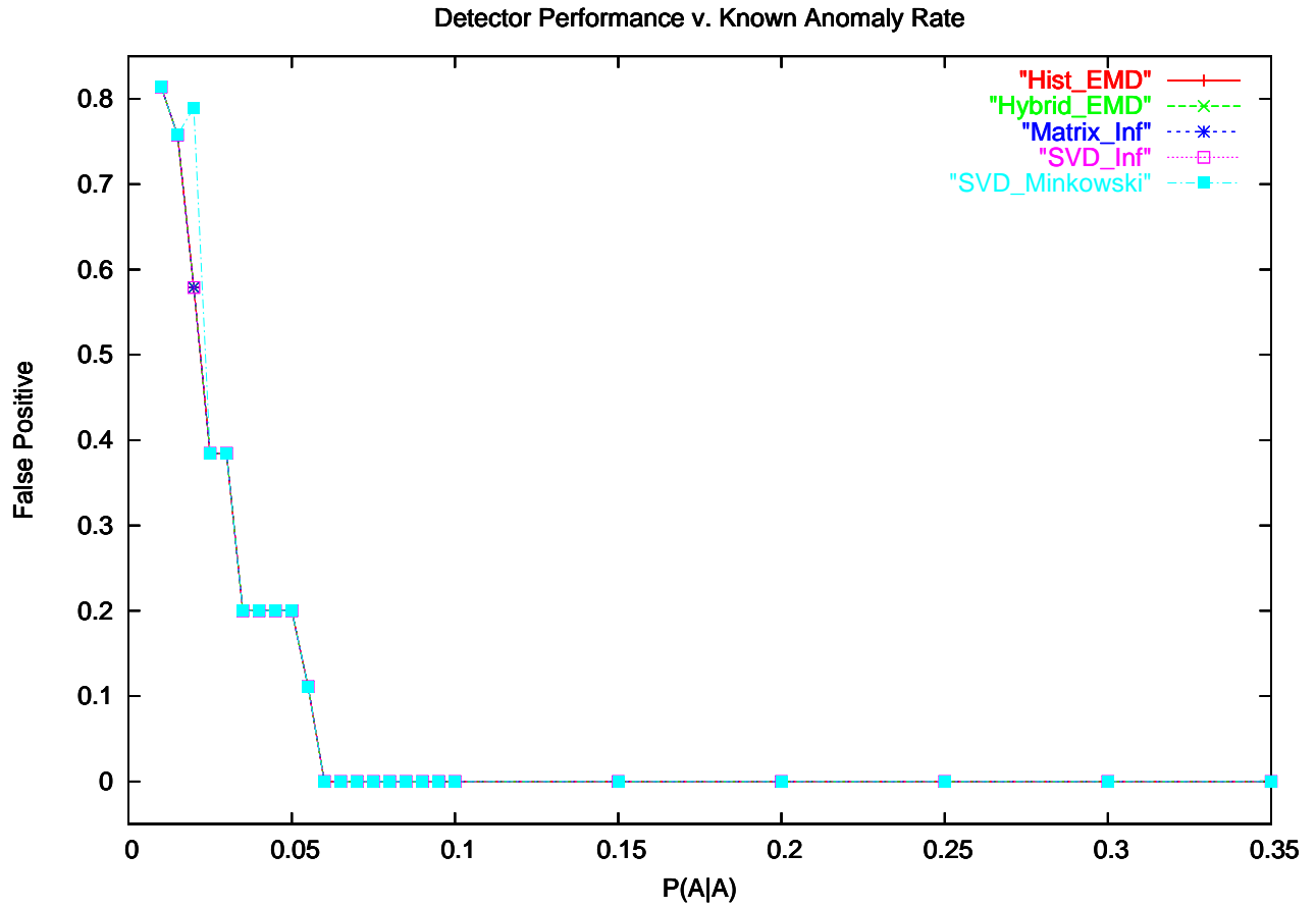
Figure 8: The curve for the performance of the detector with several combinations of model builders and model comparers for the third experiment. The horizontal axis lists the parameter aa from Figure 7, and the vertical axis lists the false positive rate where the positive class is the anomaly.
