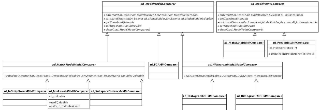
Figure 3: The model comparer hierarchy. Matrix-based model-to-model comparers extract a matrix representation of the models prior to comparison just as histogram-based model-to-model comparers extract a histogram representation of the models.
