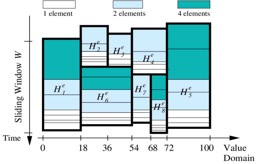
Figure 4: A hybrid histogram from [19].
