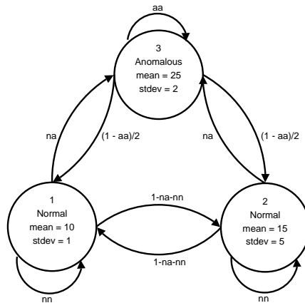
Figure 7: The Markov chain that generated the artificial data in the third experiment. Transition parameters allow for tuned datasets.
