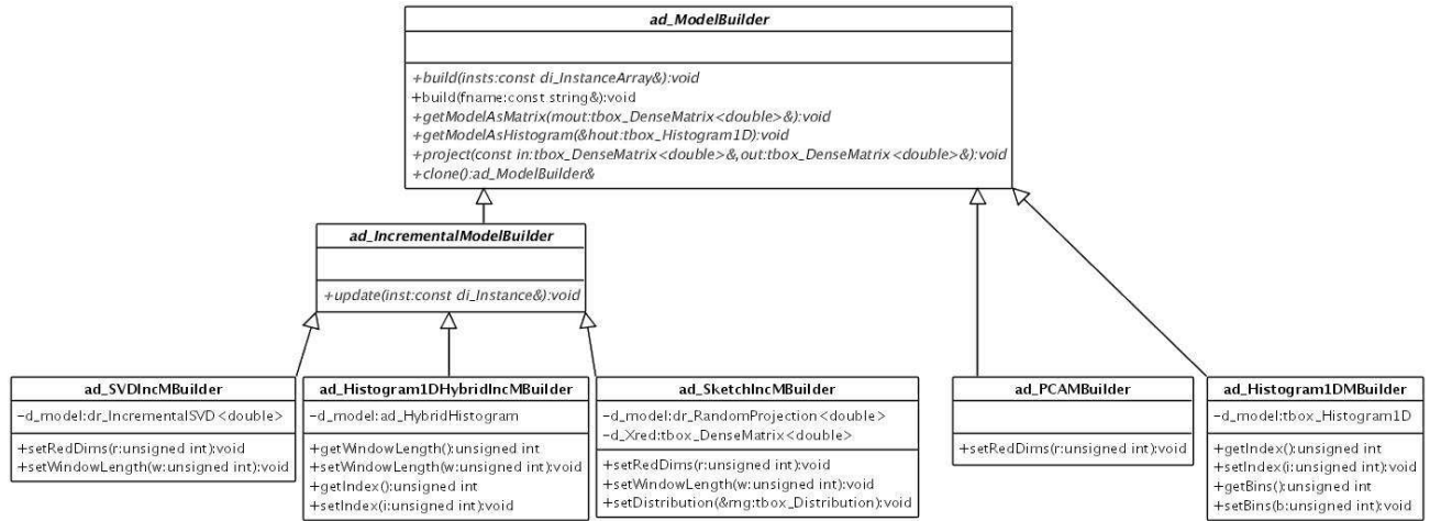
Figure 2: The model builder hierarchy.
