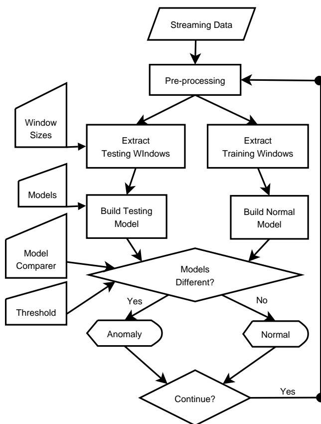
Figure 5: Anomaly detector flowchart.
