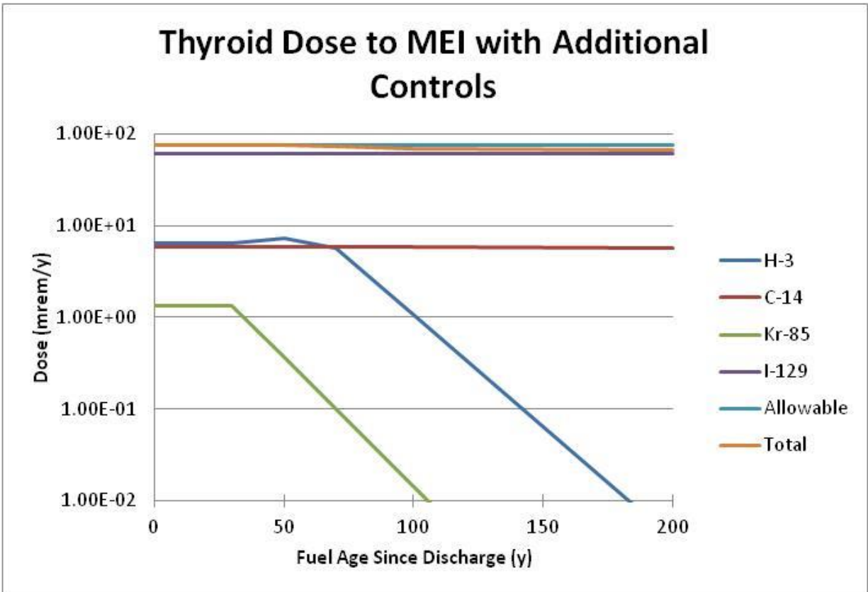
Figure C.4-8. Dose to the thyroid and dose contribution from each of the volatile radionuclides, as a function of fuel age for a 1000-t/y recycle plant processing 100-GWd/tIHM AHTGR fuel. Implementing controls required by 40 CFR 190 release limit and additional controls required to meet the 25-mrem/y whole body dose limit. Allowable thyroid dose shown is 75 mrem/y.
