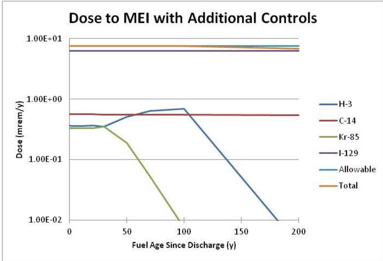
Figure B.5-9. Dose to the thyroid and dose contribution from each of the volatile radionuclides, as a function of fuel age for a 1000-t/y recycle plant processing 100-GWd/tIHM PWR MOX fuel. Implementing controls required by 40 CFR 190 release limit and additional controls required to meet an allocated 2.5-mrem/y whole body dose limit. Allowable thyroid dose shown is 7.5 mrem/y.
