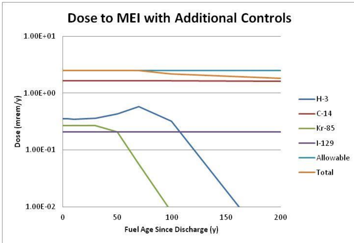
Figure A.1-5. Dose to MEI total and dose contribution from each of the volatile radionuclides, as a function of fuel age for a 1000-t/y recycle plant processing 20-GWd/tHM PWR UOX fuel. Implementing controls required by 40 CFR 190 and additional controls needed to meet an allowable dose limit at 2.5 mrem/y.
