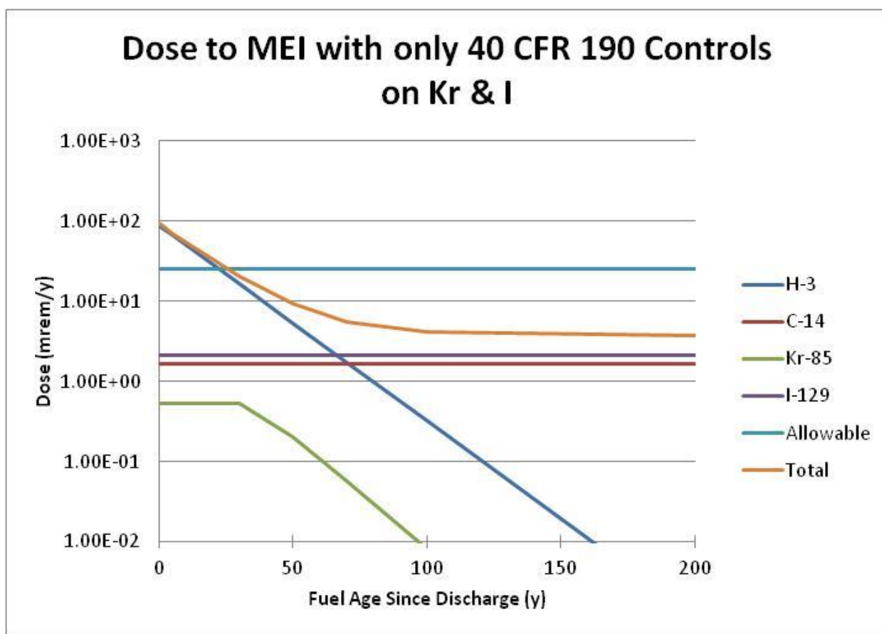
Figure A.1-2. Total whole body dose and dose contributions arising from the volatile radionuclides to the MEI from 1000-t/y recycle plant processing 20-GWd/tHM PWR UOX fuel. Allowable dose limit is shown at the 25-mrem/y whole body dose level.
