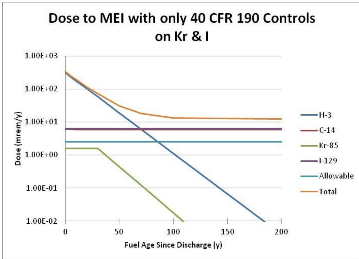
Figure A.2-3. Total whole body dose and dose contributions arising from the volatile radionuclides to the MEI from 1000-t/y recycle plant processing 60-GWd/tHM PWR UOX fuel with iodine and krypton controls per 40 CFR 190. Allowable dose limit is shown at the 2.5-mrem/y whole body dose level.
