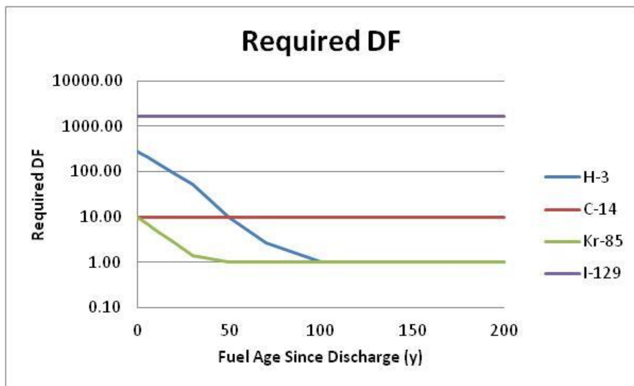
Figure C.2-6. Required DFs for each of the volatile radionuclides, as a function of fuel age for a 1000-t/y recycle plant processing 30-GWd/tHM AHTGR fuel. Implementing controls required by 40 CFR 190 and additional controls needed to meet an allowable dose limit at 2.5 mrem/y.
