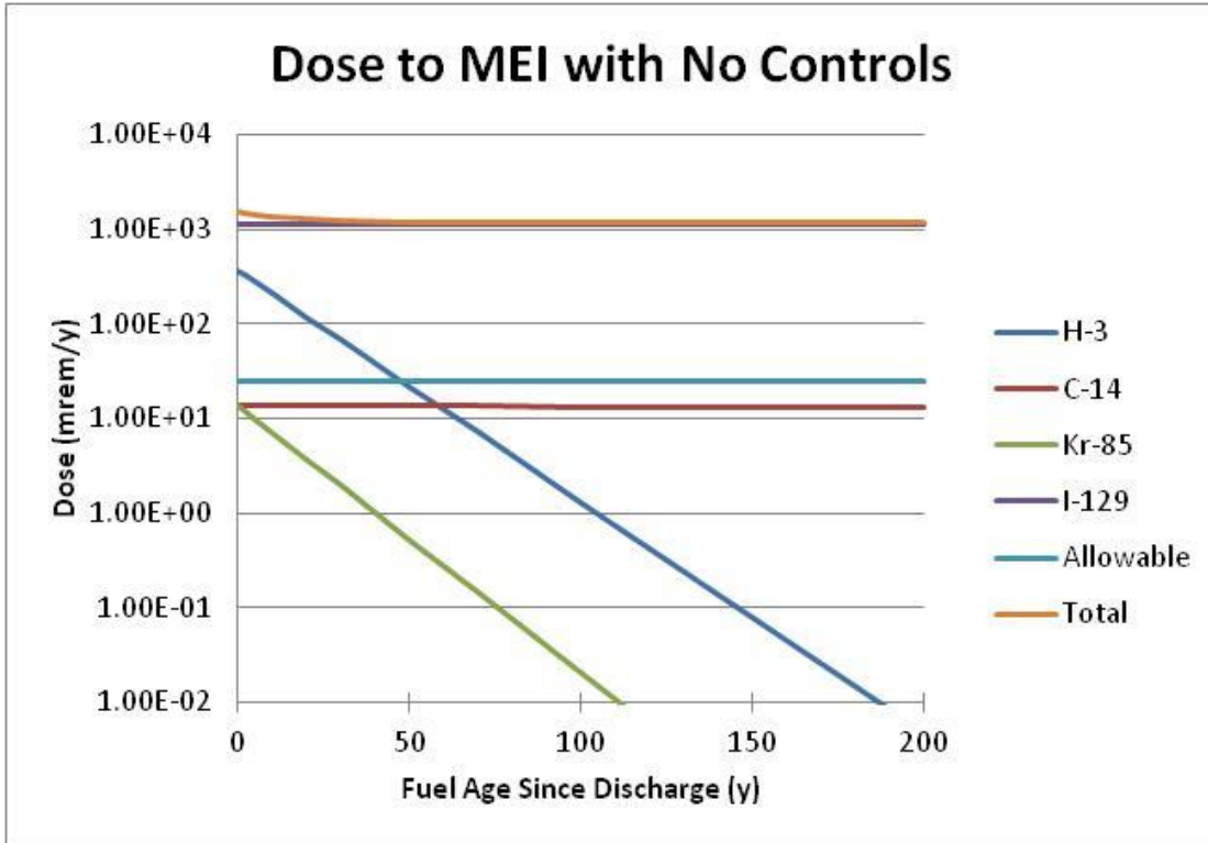
Figure C.3-1. Total whole body dose and dose contributions arising from the volatile radionuclides to the MEI from 1000-t/y recycle plant processing 60-GWd/tHM AHTGR fuel. Allowable dose limit is shown at the 25-mrem/y whole body dose level.
