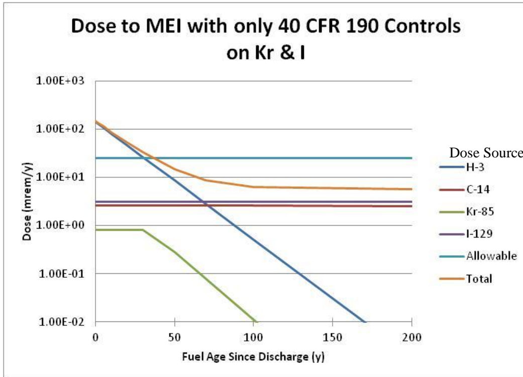
Figure 7. Total whole body dose and dose contributions arising from the volatile radionuclides to the MEI from 1000-t/y recycle plant processing 30-GWd/tIHM PWR UOX fuel with iodine and krypton controls per 40 CFR 190. Allowable dose limit is shown at the 25-mrem whole body dose level.
