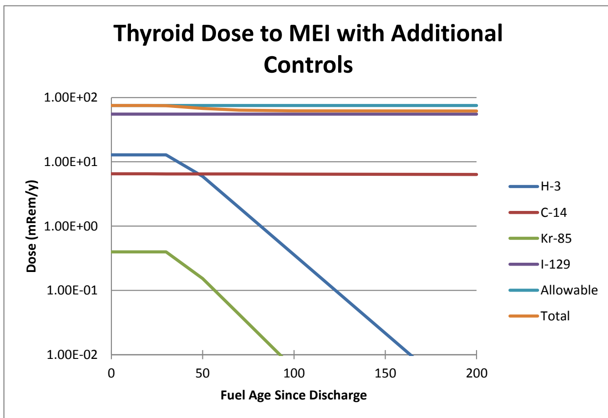
Figure C.2-8. Dose to the thyroid and dose contribution from each of the volatile radionuclides, as a function of fuel age for a 1000-t/y recycle plant processing 30-GWd/tHM AHTGR fuel. Implementing controls required by 40 CFR 190 release limit and additional controls required to meet the 25-mrem/y whole body dose limit. Allowable thyroid dose shown is 75 mrem/y.
