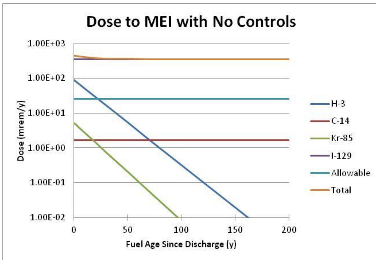
Figure A.1-1. Total whole body dose and dose contributions arising from the volatile radionuclides to the MEI from 1000-t/y recycle plant processing 20-GWd/tIHM PWR UOX fuel. Allowable dose limit is shown at the 25-mrem/y whole body dose level.
