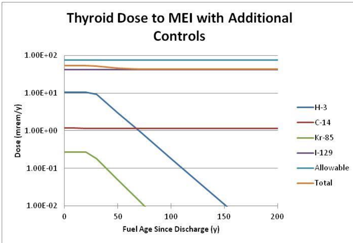
Figure B.2-8. Dose to the thyroid and dose contribution from each of the volatile radionuclides, as a function of fuel age for a 1000-t/y recycle plant processing 20-GWd/tHM PWR MOX fuel. Implementing controls required by 40 CFR 190 release limit and additional controls required to meet the 25-mrem/y whole body dose limit. Allowable thyroid dose shown is 75 mrem/y.
