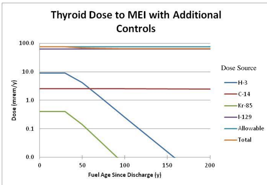
Figure 14. Dose to the thyroid and dose contribution from each of the volatile radionuclides with fuel age for a 1000-t/y recycle plant processing 30-GWd/tIHM PWR UOX fuel. Implementing controls required by 40 CFR 190 release limit and additional controls required to meet the 25-mrem whole body dose limit. Allowable thyroid dose shown is 75 mrem.
