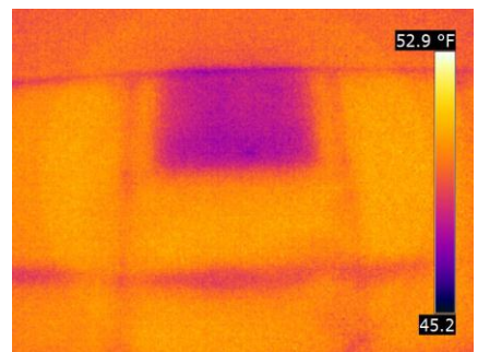
Fig. 51. Gable vent from inside sunroom.
