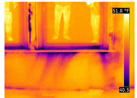
Fig. 57. Thermal "fingers" from air intrusion around windows. (Body heat from data takers is reflected from window.)
