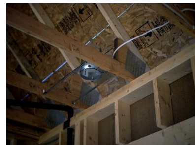
Fig. 19. Recessed lighting installed before ceiling is finished and insulated.
