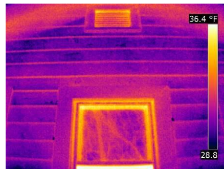
Fig. 50. Gable vent in sunroom area of the west façade.
