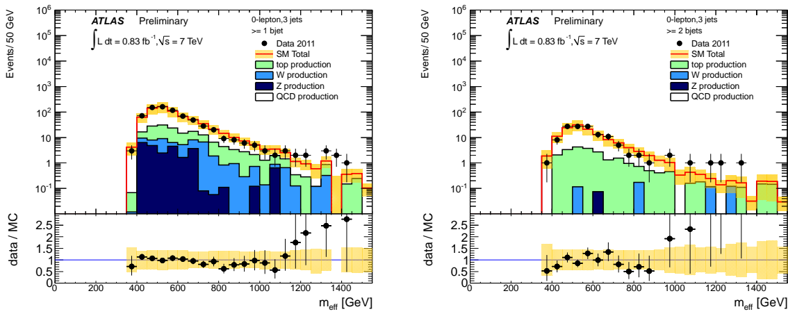
Figure 2: Effective mass distribution for the QCD control region ( \Delta\phi_{min} < 0.4 ) for events with 1 (left) or 2 (right) b -tagged jets. The lower plot shows the bin-by-bin ratio of the data to the SM expectation. The QCD prediction validated in these control samples is derived using the smearing method described in the text, other SM background contributions are estimated from MC. The yellow band shows the full systematic uncertainty on the SM expectation
