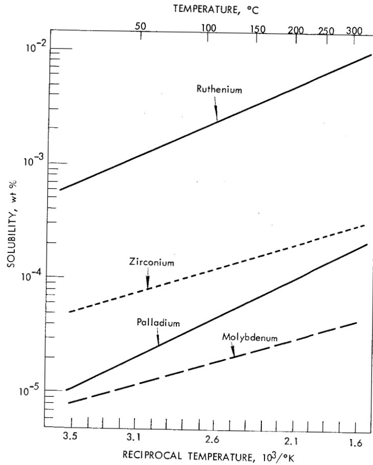
Fig. 2.5. Solubility of several fission product metals in uranium-saturated mercury. --- Established solubility; — upper solubility limit as defined by limit of detection.
