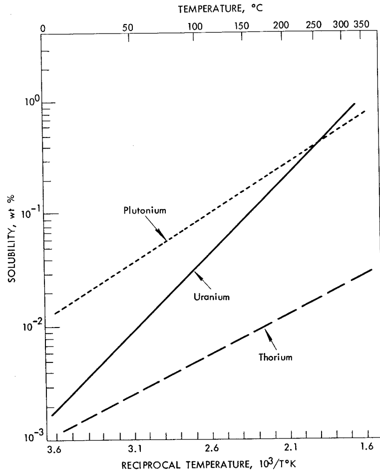
Fig. 2.1. Solubility of plutonium, uranium, and thorium in mercury. Plutonium from data of Bowersox and Leary. 13
