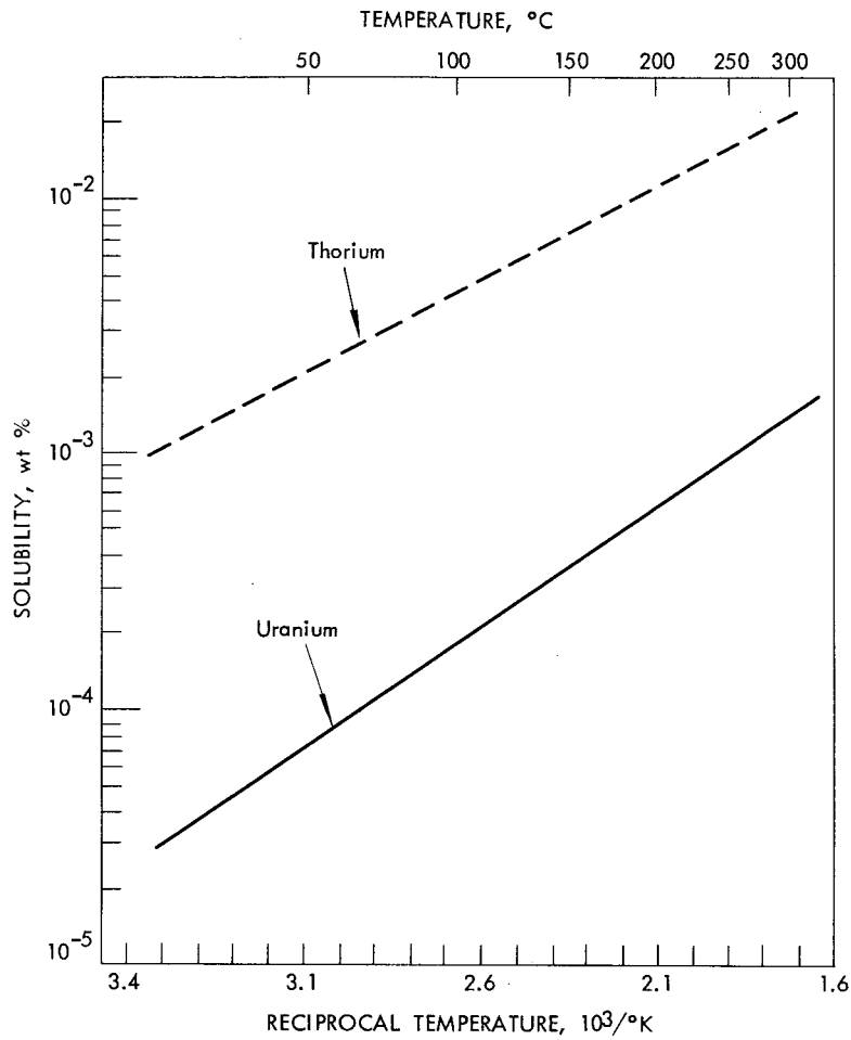
Fig. 2.3. Solubility of a uranium-thorium mixture, 4000 g of uranium per ton of thorium.
