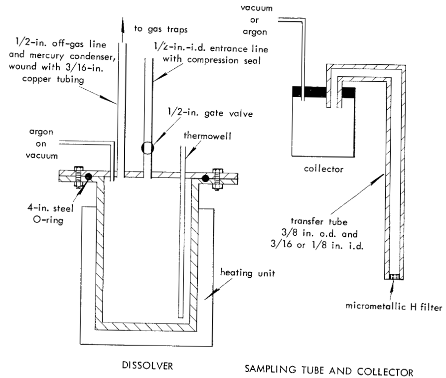
Fig. 3.1. Stainless steel apparatus for mercury solubility determinations.
