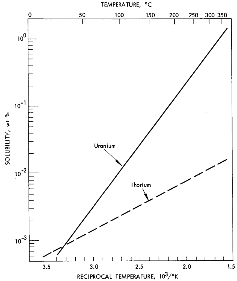
Fig. 2.2. Solubility of uranium and thorium in a mutually saturated solution.
