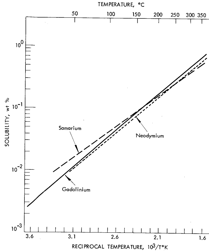
Fig. 2.4. Solubility of samarium, neodymium, and gadolinium in mercury.
