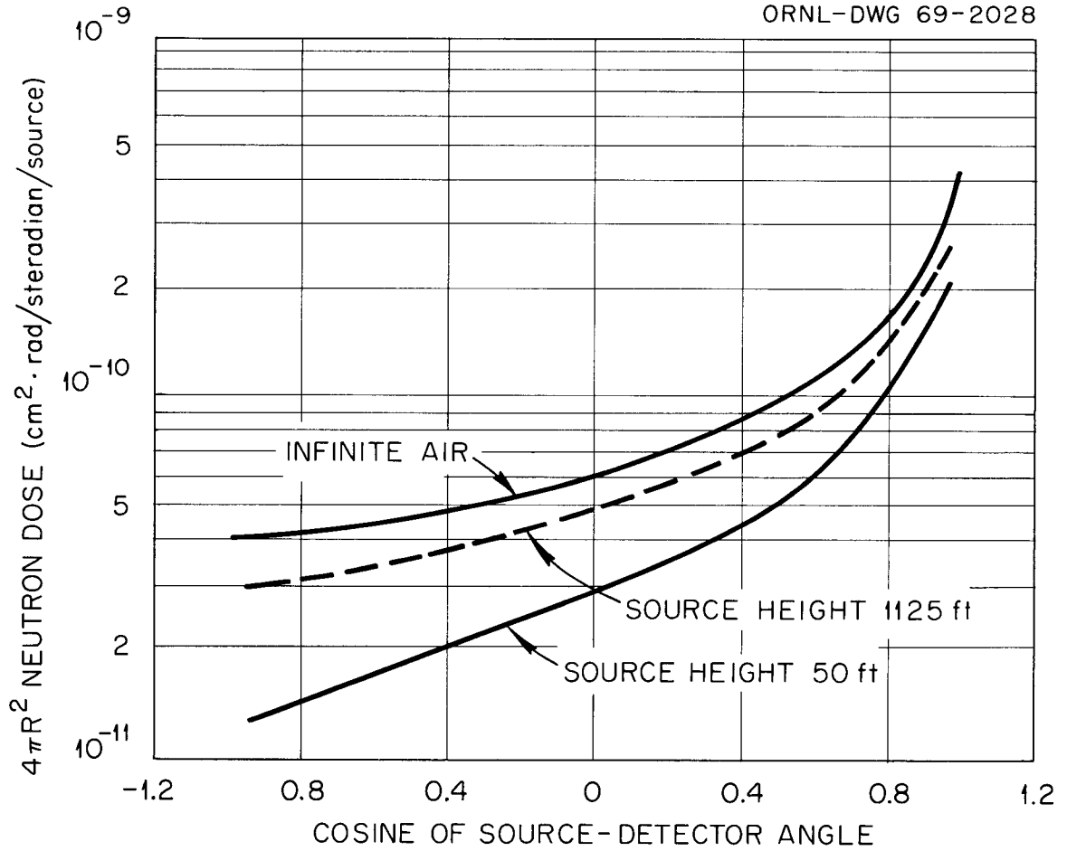
Fig. 4. Angular Distribution of Neutron Dose at a Range of 900 Meters Due to a 12.2- to 15-MeV Source. For the air-over-ground case, the detector is 3 ft above the ground.
