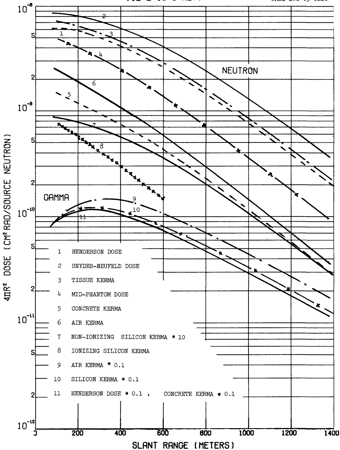
Fig. 2. 4\pi R^2 Dose Versus Range Due to a 12.2- to 15-MeV Source.
