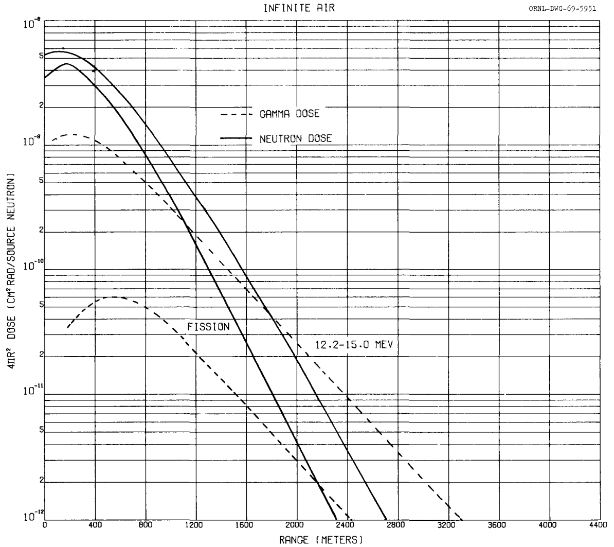
Fig. 3. 4\pi R^2 Dose Versus Range for both 12.2- to 15-MeV and Fission Sources.
