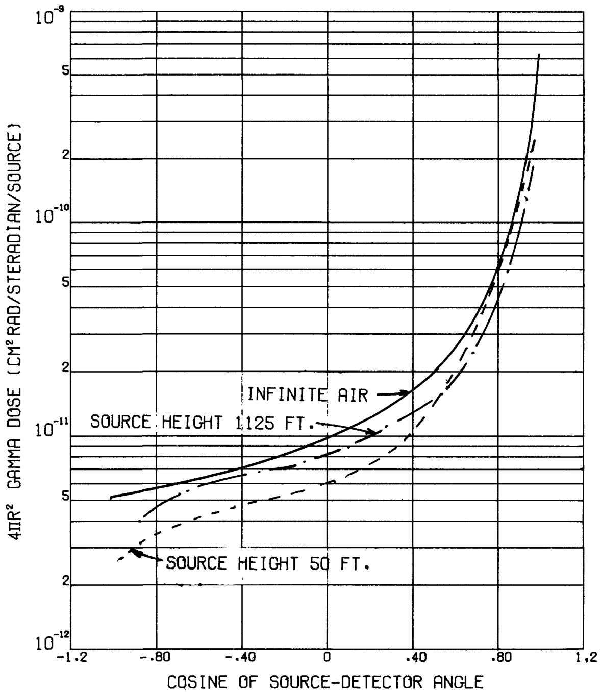
Fig. 5. Angular Distribution of Gamma-Ray Dose at a Range of 900 Meters Due to 12.2- to 15-MeV Source. For the air-over-ground case, the detector is 3 ft above the ground.
