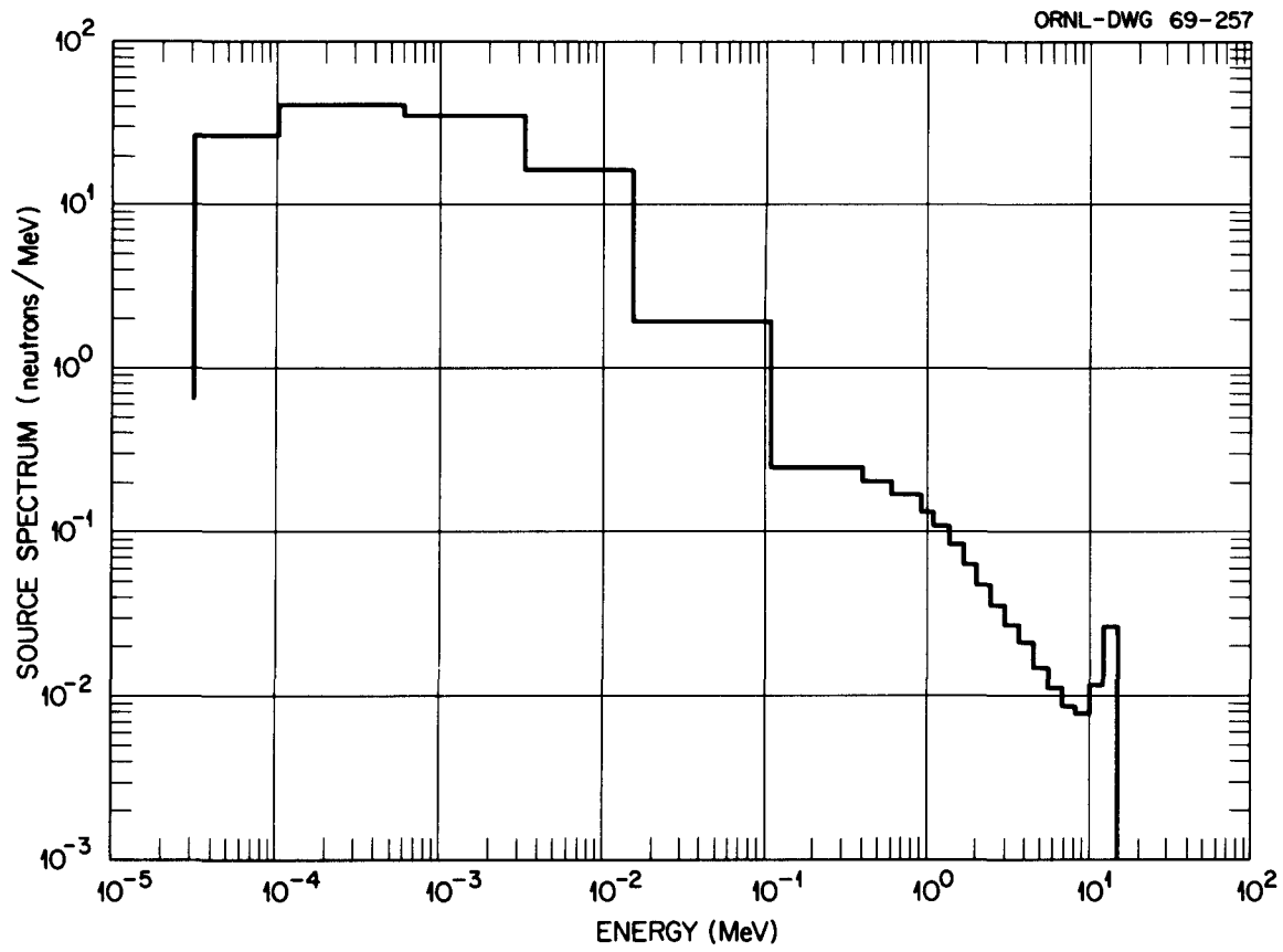
Fig. 1. Source Energy Spectrum for a Typical Thermonuclear Weapon.
