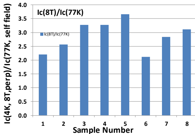
Fig. 8. Ratio of critical current measured at 4 K in 8 T background field (applied perpendicular to the wide face of tape) and at 77 K, self-field.
