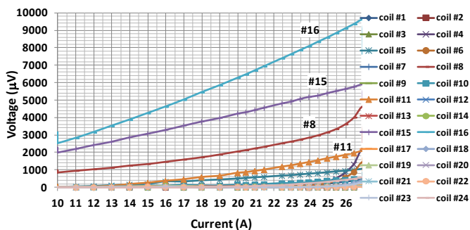
Fig. 9. Performance of individual pancakes during a test where several of them got degraded (as seen by the onset of voltage well before 25 A). These pancakes have been tested several times before and showed no such behavior.
