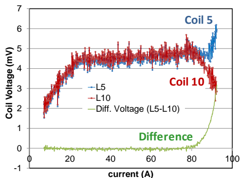
Fig. 6. Measured voltage in two pancake coils 5 (L5) and 10 (L10) along with the difference between the two to detect the pre-quench phase during a current ramp with changing rate (accelerating, constant and decelerating).
