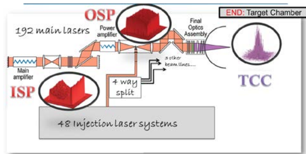
Figure 4: Simplified view of the main laser model showing the beam shape at the Integrated Sensor Package (ISP) the Output Sensor Package (OSP) and the Target Chamber Center (TCC)
