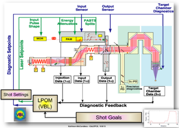
Figure 5: Diagram showing the cycle of data flowing into the laser setup from LPOM (Blue and Green) and back into the LPOM model (Black).
