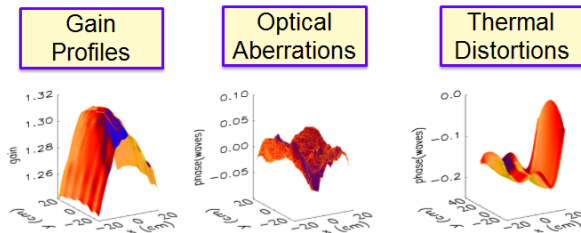
Figure 3: Sample of various spatial distributions which affect the beam’s performance as it interacts in the optical chain.
