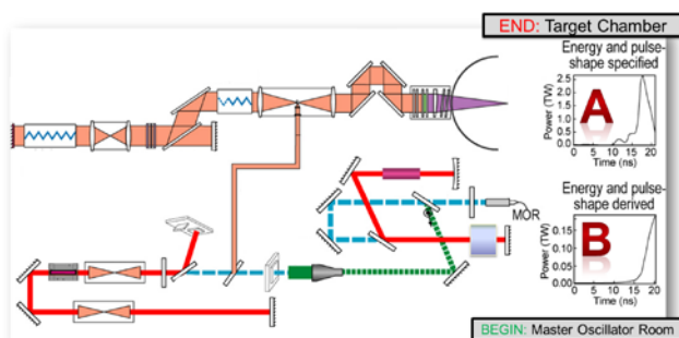
Figure 1: A sample beam line layout with Master Oscillator Room (MOR) at the beginning (B) and Target Chamber at the end (A)
