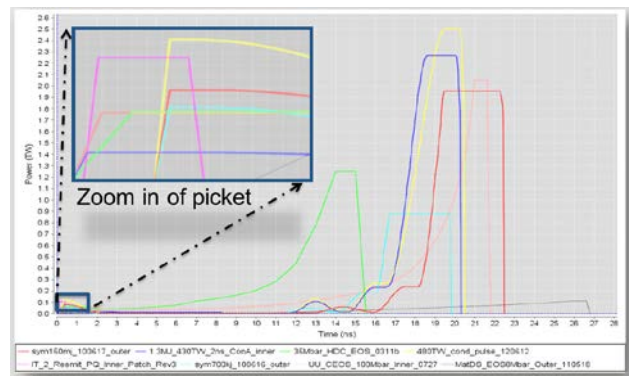
Figure 2: Example of pulse shapes for different experiments. Both small features (picket) and larger scale features must be accurately shaped.
