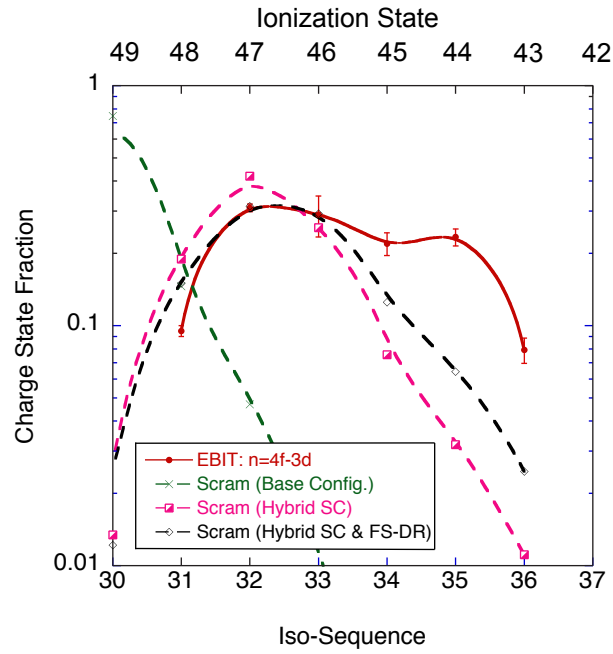
FIG. 7. Comparison of the Au charge state distribution at 2.66 keV determined from from the 4f \rightarrow 3d transitions measured from the EBIT plasma and simulations from SCRAM.
