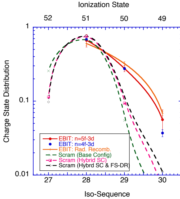
FIG. 4. Comparison of the Au charge state distribution at 4.54 keV determined from the 5f \rightarrow 3d and 4f \rightarrow 3d transitions and radiative recombination emission measured from the EBIT plasma and simulations from SCRAM.
