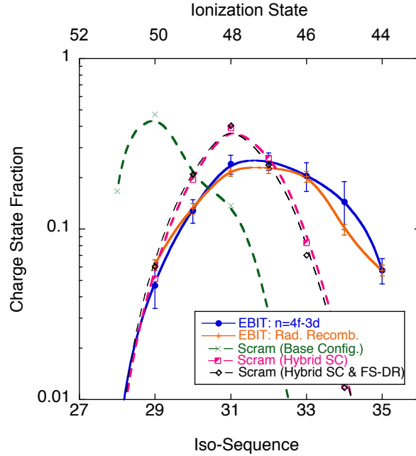
FIG. 6. Comparison of the Au charge state distribution at 2.92 keV determined from the 4f \rightarrow 3d transitions and radiative recombination emission measured from the EBIT plasma and simulations from SCRAM.
