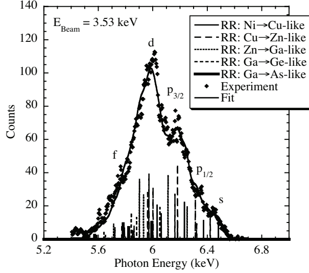
FIG. 3. Radiative recombination spectrum measured by the XRS in a plasma with an E_{Beam} = 3.53 keV. The RR features are fit with calculations from GRASP to infer the CSD.
