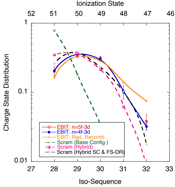
FIG. 5. Comparison of the Au charge state distribution at 3.53 keV determined from the 5f \rightarrow 3d and 4f \rightarrow 3d transitions and radiative recombination emission measured from the EBIT plasma and simulations from SCRAM.
