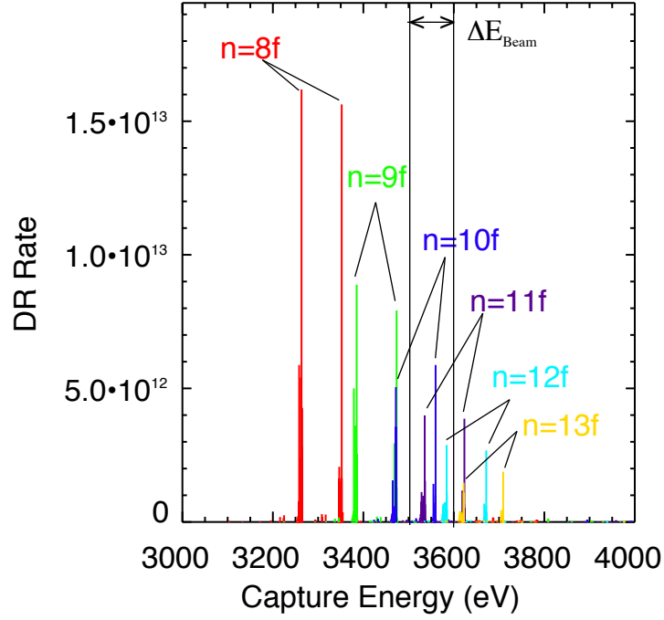
FIG. 8. Dielectric Capture Rate vs. Capture Energy (eV) for 3d6fnf with 8 \leq n \leq 13 for Ni-like Au into Cu-like Au in the E_{beam} = 3.53 keV monoenergetic Beam EBIT plasma.
