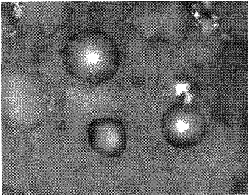
Fig. 6. Typical Uranium Carbide Spheres Produced in Induction Plasma Torch Reactor. Mag. 500X.
