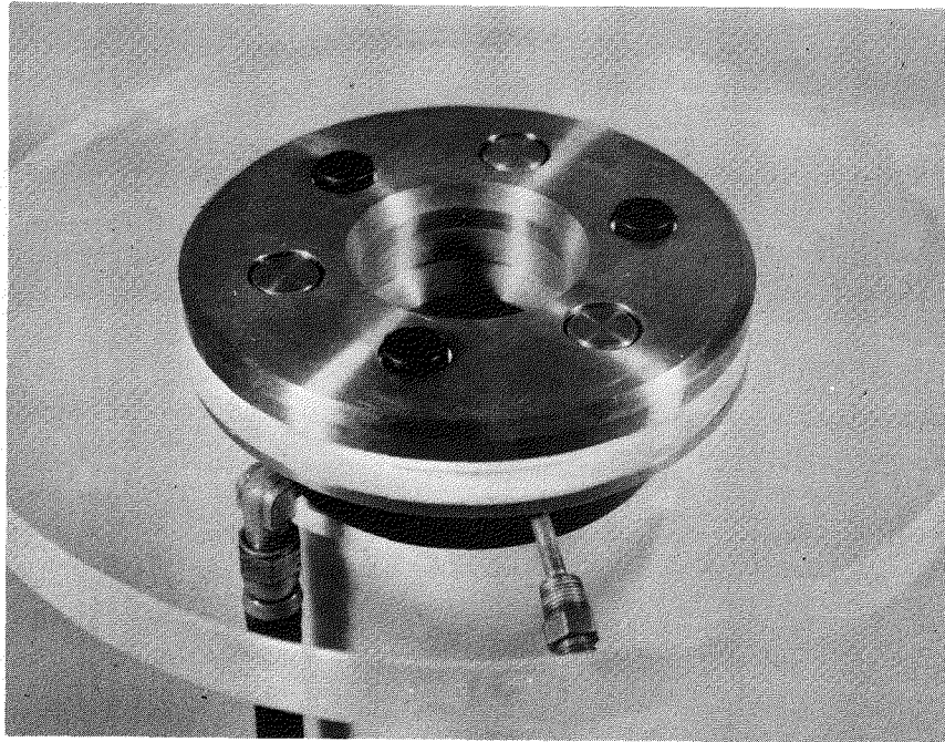
a. Torch Assembly before Run
