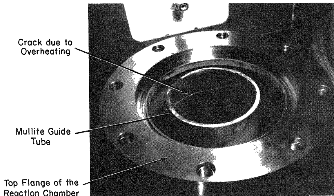
Fig. 10. Top Portion of Mullite Tube, Showing Breakage due to Overheating
