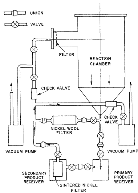
Fig. 5 Product Receiver Assembly
