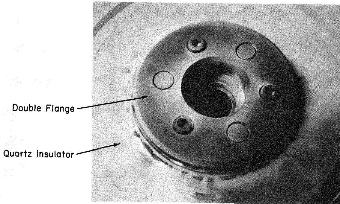
b. Torch Assembly after Run
