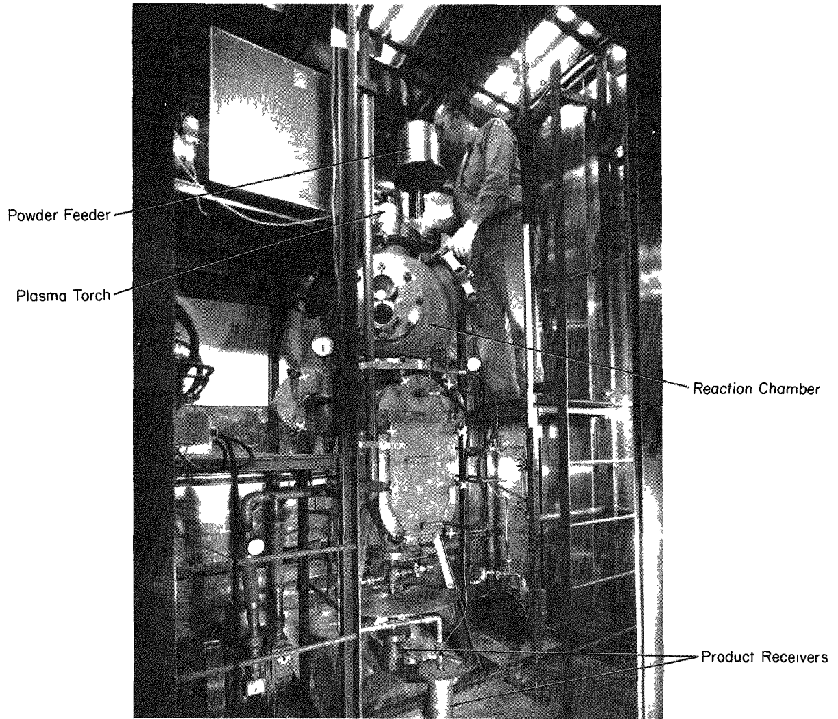
Fig. 4. Induction Plasma Torch Reactor. ANL Neg. No. 308-2114.
