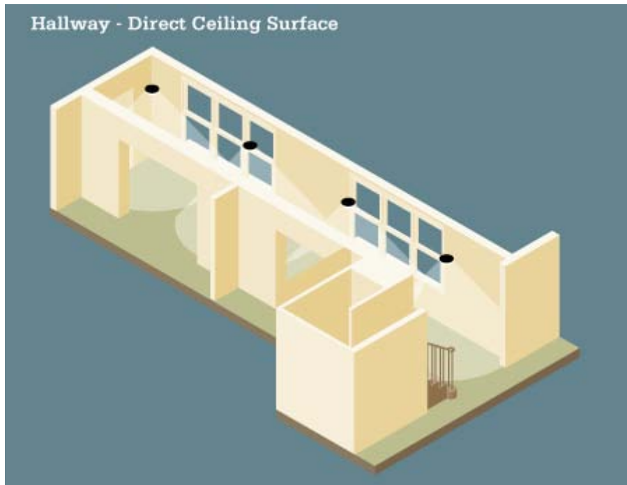
Figure 86. Direct - ceiling surface fixtures.
