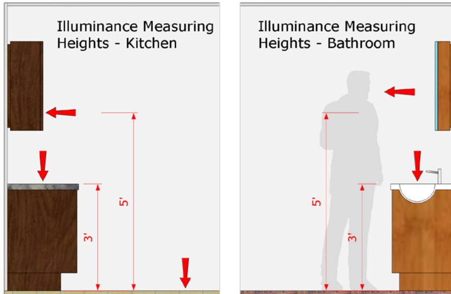
Figure 15. Illuminance measuring heights for (left) kitchen, (right) bathroom, and floor illumination. (Arrows indicate surfaces to be illuminated).
