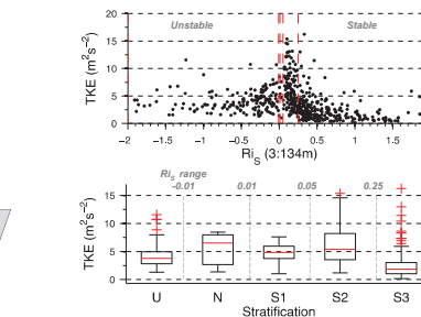
Figure 6. TKE as a function of stability in October 2011. Data are for wind speeds greater than 3 m/s from all directions.
