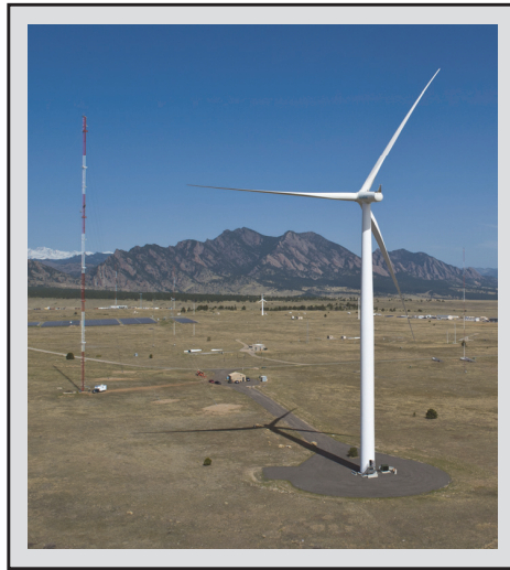
Figure 1. A wind turbine at the National Wind Technology Center near Boulder, Colorado. The hub is 80 m above ground. The inflow monitoring tower (left, WNW from the turbine) is 135 m tall. Photo by Dennis Schroeder NREL/PIX 19013.
