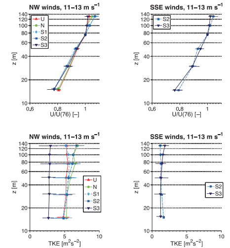
Figure 7. Changes in mean flow profiles and turbulent kinetic energy as a function of wind direction and stability. Data are from October 2011. Profiles are grouped into unstable (U), neutral (N), and increasingly stable (S1 - S3) conditions using the Richardson number from 3 to 134 meters above ground.
