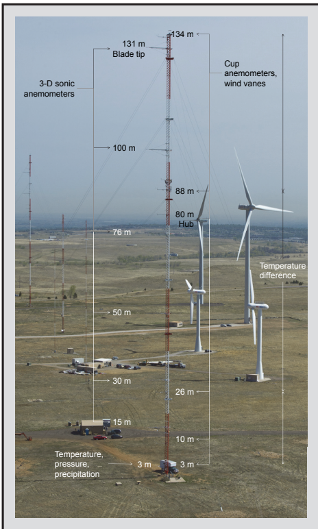
Figure 2. Instrumentation on the 135-m tower measures mean and turbulent properties of flow into a utility-scale turbine. Photo by Dennis Schroeder NREL/PIX 19023.
