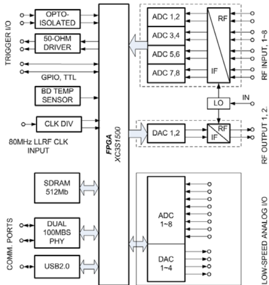
Figure 1. Functional diagram of the field controller module.
