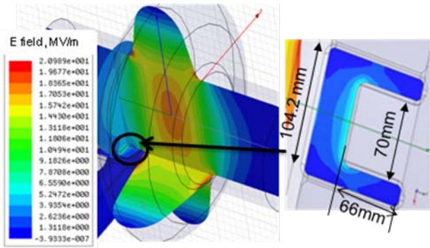
Figure 2 2. HFSS plot of the electric field intensity in the waveguide to beam pipe coupling aperture. Fields are normalized to 2.4 MV accelerating voltage.
