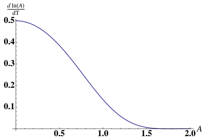
Figure 2: Cooling rate for the given set of parameters with no painting.
