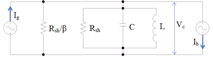
Figure 2: Equivalent circuit of FPC in the cavity.
