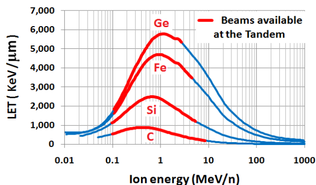
Figure 4: LET values in water as function of energy [9] for four of the ion beams available at the BNL Tandem. The available energies are indicated in red.
