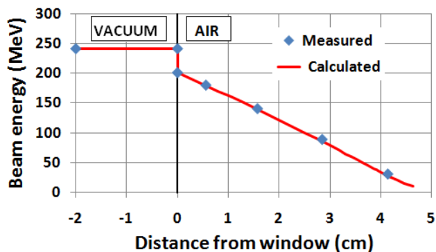
Figure 3: Energies of an iron beam, first in vacuum with and without interposing the 95 microinch thick HAVAR window and then in air as function of the distance from the window. The errors are smaller than the points. The initial energy was 241 MeV and the energy loss values in HAVAR and in air are well reproduced by the red curve calculated by using results from the SRIM code [9]
