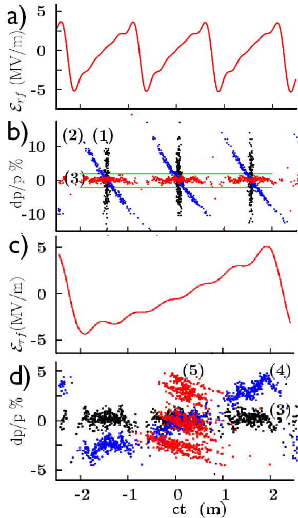
Figure 2: Longitudinal Merge: a) 201 MHz + harmonics; b) Initial Rotation (1)=initial, (2)=drifted, (3)=after rf 1 ; c) 67 MHz + harmonics; d) Merge (3)=from above, (4)=rf 2 , (5)=drifted).
