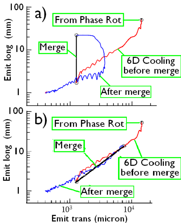
Figure 5: Longitudinal vs transverse emittances from phase rotation to 6D cooling, including bunch merges: a) with 2D merge; b) with 6D merge.
