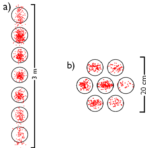
Figure 4: x - y distributions in transverse merging: a) after fan-out for capture into 7 transports; b) at end of transports, before capture as one beam.
