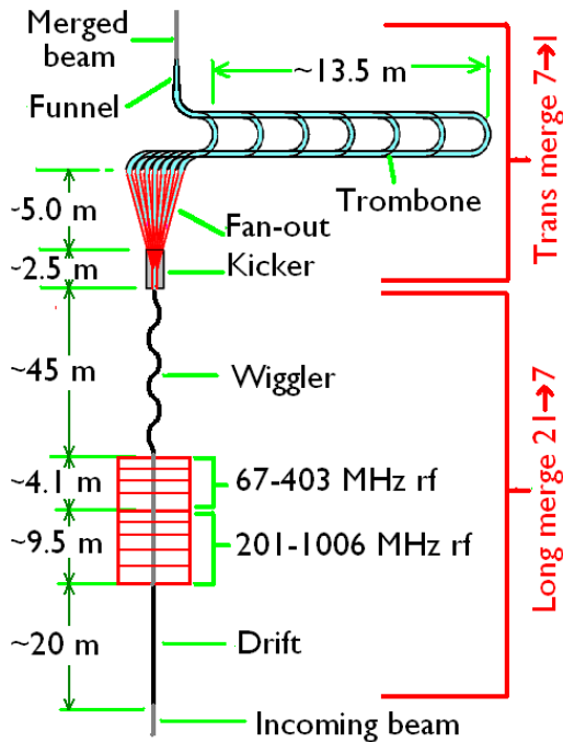
Figure 1: Schematic of 6D merge.
