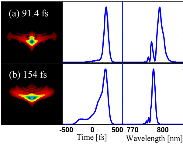
Figure 1: Each row corresponds to a simulation result. The FWHM pulse duration of the main temporal peak is also shown for each case. The three columns, starting from left, show FROG images, temporal and spectral distributions. Amplitudes are normalized. No taper is applied for (a), but 6% linear taper starting from z = 7 m for (b).
