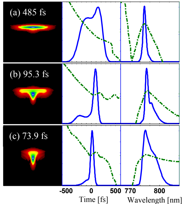
Figure 2: Each experimental FROG result is a row in the figure labelled by the FWHM of the main temporal peak. The three columns, starting from left, show retrieved FROG images, temporal and spectral distributions including phase. Amplitudes (blue) are normalized and phases (green) are plotted from -10 to +10 rad.
