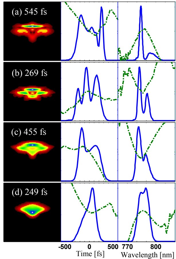
Figure 5: Typical experimental FROG results for the tapered case.
