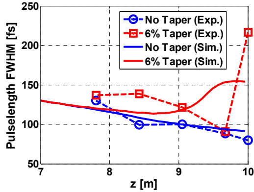
Figure 4: Radiation pulselength (FWHM) evolution along the undulator. Blue and red lines are for non-tapered and tapered cases, respectively. Solid and dashed lines are for simulations and for experiments, respectively.
