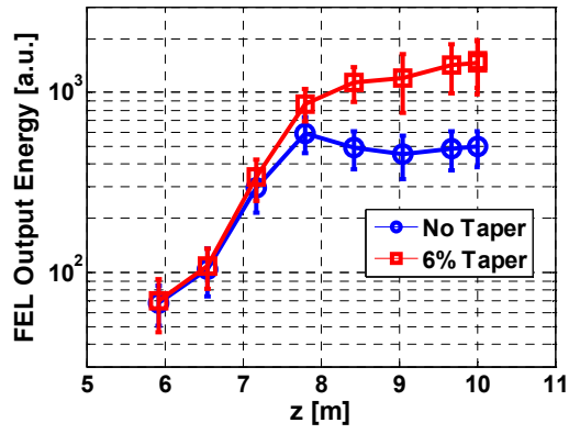
Figure 3: Gain curves with and without tapering.
