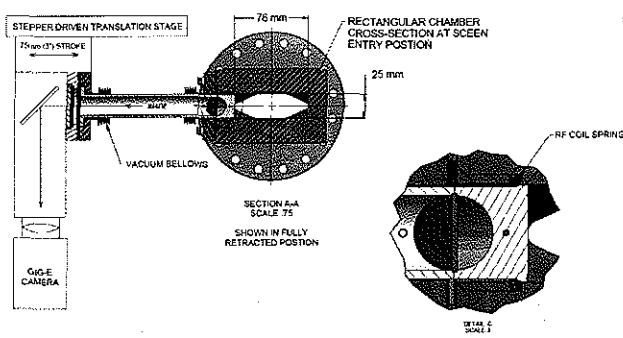
Figure 3: Vacuum chamber for the second flag.
