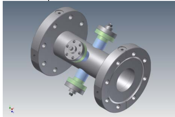
Figure 3: Design of the round BPM housing.
