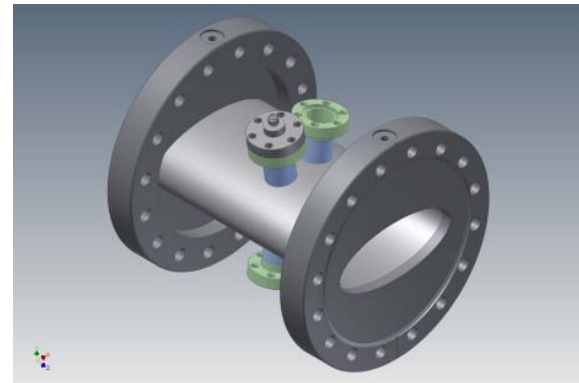
Figure 4: Design of the elliptical BPM housing.
