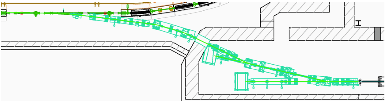
Figure 1: Linac to Booster Transfer Line
