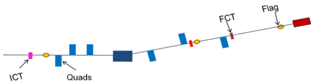
Figure 6: Layout of the transport line to the second dump. Beam enters from the left side.
