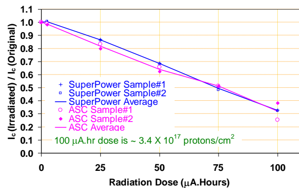
Figure 1 Normalized critical current versus radiation for self-field.
