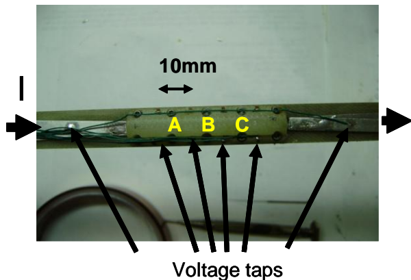
Figure 4: A photograph of a sample holder with 4mm YBCO tape and 10mm segments "A", "B" and "C" irradiated. A 4mm wide YBCO sample is placed under the G-10 cover. The position of voltage taps is shown. The direction of current is shown as left to right arrow.
