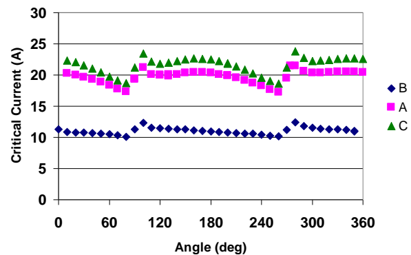
Figure 6: Critical current at three different sections at 0.5T at a high dose level (100 \mu A -hr) for SuperPower samples
