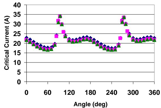
Figure 5: Critical Current at different sections at the same magnetic field (0.5 T) at a low dose level (2.5 \mu A -hr) for SuperPower samples.
