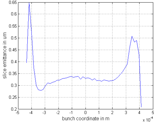
Figure 2: Slice emittance of a 250 pC bunch at the end of the injector. The assumed thermal emittance is 0.23 \mu\text{m} .
