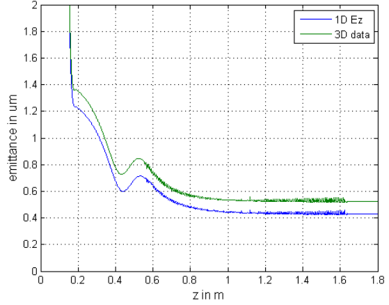
Figure 6: Comparison of simulations using on-axis 1D E_z fields and 3D fields.
