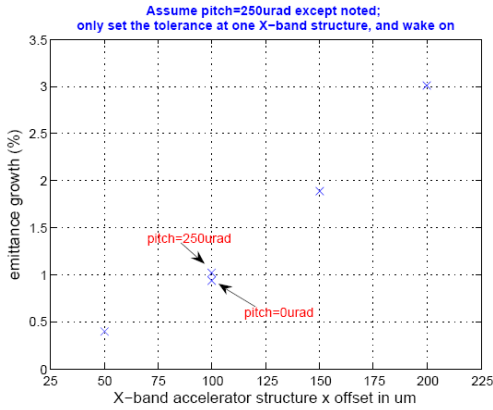
Figure 5: Emittance growth vs the structure transverse offset for a 333 pC bunch charge.
