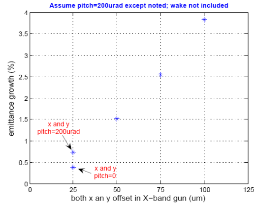
Figure 4: Emittance sensitivity to the gun alignment. A 200 \mu\text{rad} pitch is assume except as noted in the plot.
