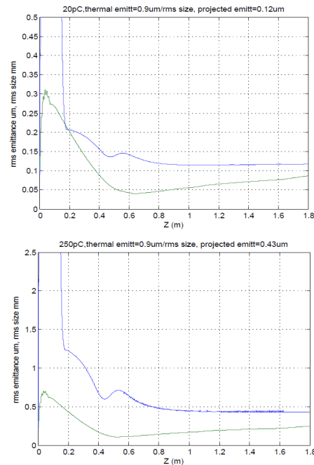
Figure 1: Normalized projected emittance and rms beam size along the injector beamline for 20 pC (top) and 250 pC (bottom) bunch charges.
