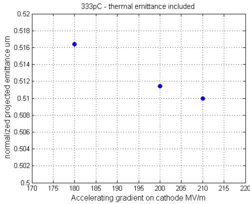
Figure 3: Emittance versus cathode gradient for a 333 pC bunch charge. Thermal emittance is included.
