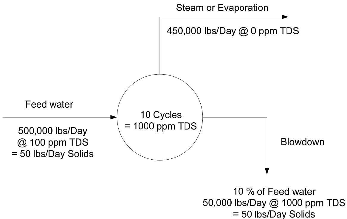
Figure A 1: Cycles of Concentration and Mass Flow Example of a Steam System
