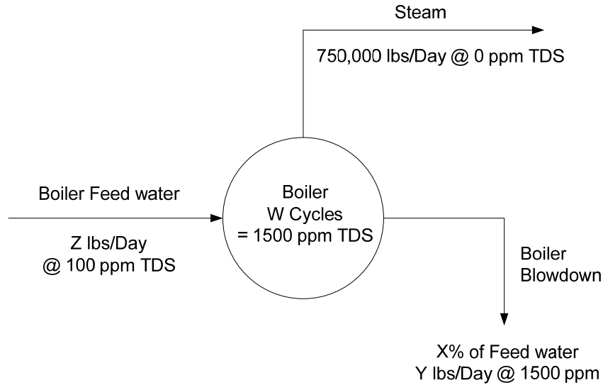
Figure A 2: Sample Boiler Scenario
