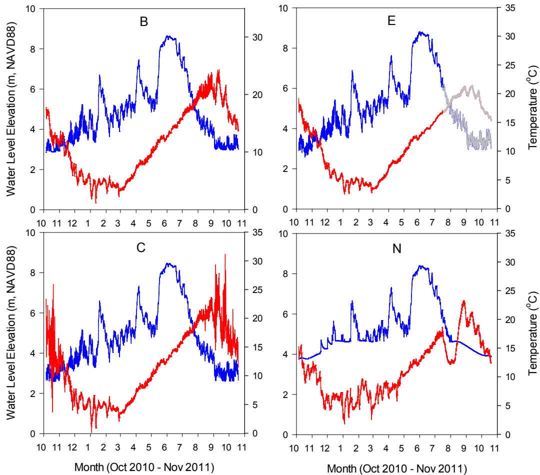
Figure 3.2. Water-surface elevation (blue) and water temperature (red) from Hobo data loggers at Sites B, C, E, and N at the SRD. The Hobo sensor at Site E was discovered to have moved from its installation location and been buried in sediment on July 17, 2011; displayed in gray. Therefore, data following this time period should be considered uncorrected.
