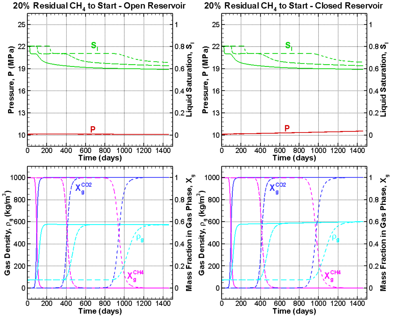
Figure 12. Transient response at 50 m (solid), 100 m (long dash), and 150 m (short dash) away from the injection well for \text{CO}_2 injection into (a) open and (b) closed shallow reservoirs containing brine with 20% residual \text{CH}_4 .
