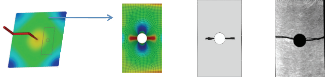
ORNL and PNNL models support prediction from process to property. Left to right: global injection molding flow prediction, global stress prediction, progressive failure prediction, and x-ray of failed sample.
