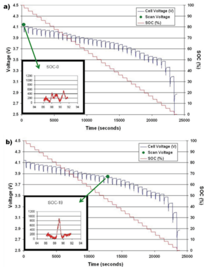
Plots of a GM 15-Ah cell from this project showing the fully charged state (open circuit voltage, V_{OC} = 4.15 V) in dark blue and state of charge at the midpoint of discharge ( V_{OC} = 3.85 V) in red, as a function of time: a) before discharging and b) during discharging. Insets at lower left are neutron intensity vs 2\theta scans.
