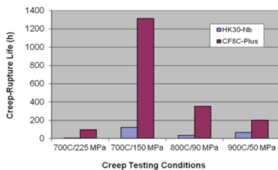
Comparison of creep rupture (top) and yield strength (bottom) for CF8C-Plus and HK30Nb cast austenitic stainless steels.
