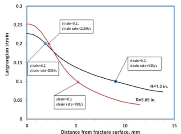
Strain distribution of AM60B specimens with two different radii. Tests were conducted at nominal speed of 500 in./s.
