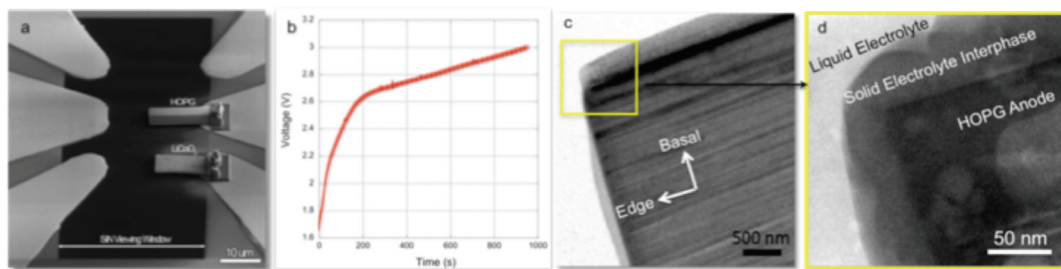
(a) Scanning electron microscopy micrograph of battery electrodes [highly oriented pyrolytic graphite (HOPG) anode and lithium cobalt oxide cathode] attached to the biasing microchips and across the silicone nitride membrane, (b) charging curve, (c) bright-field TEM image of HOPG anode before experiment, and (d) snapshot acquired during in situ electrochemistry experiment depicting the formation of the SEI on the surface of the graphite anode.
