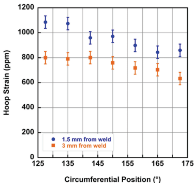
Neutron circumferential strain mapping of SWA showing variation of hoop strain at two distances from weld.
