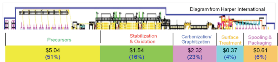
Breakdown of CF production costs (Base diagram courtesy of Harper International.)
