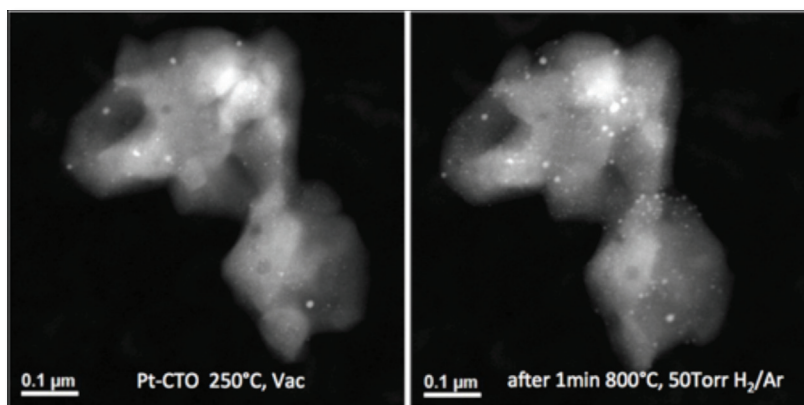
Results of a reduction experiment on a platinum-perovskite material using ORNL's specialized in situ heating technology. Bright spots are platinum nanoparticles. Image on the left was taken before the reduction treatment; image on the right is after a reduction treatment for 1 minute in a 50 Torr reducing atmosphere at a nominal temperature of 800°C.
