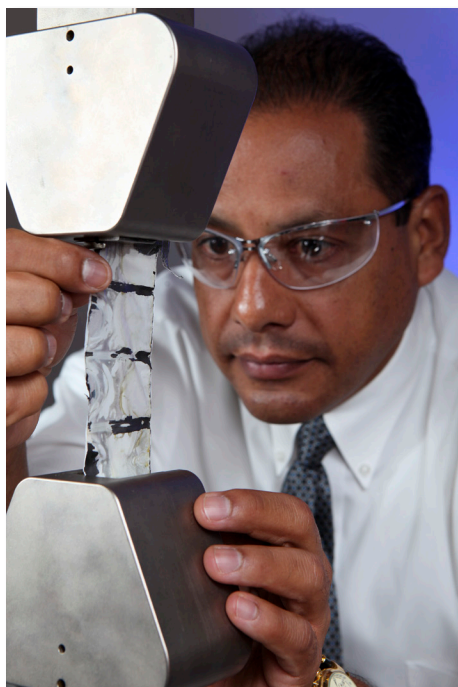
A mechanical testing machine used to characterize the stress-strain response of various battery materials.
