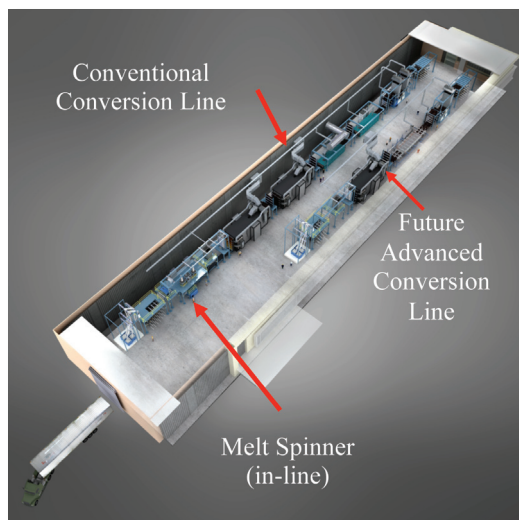
Layout of the Carbon Fiber Technology Facility production area.
