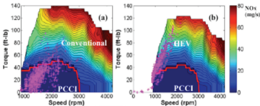
Engine speed-load map illustrating opportunities for premixed-charge compression ignition use during an urban driving duty cycle for (a) a conventional (nonhybrid) passenger vehicle and (b) an equivalent size HEV. Pink crosses correspond to engine operating points. Solid colors correspond to engine-out NO x levels.
