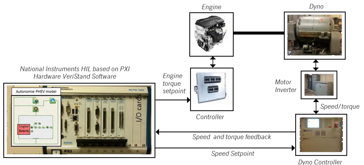
Engine-in-the-loop test platform.
