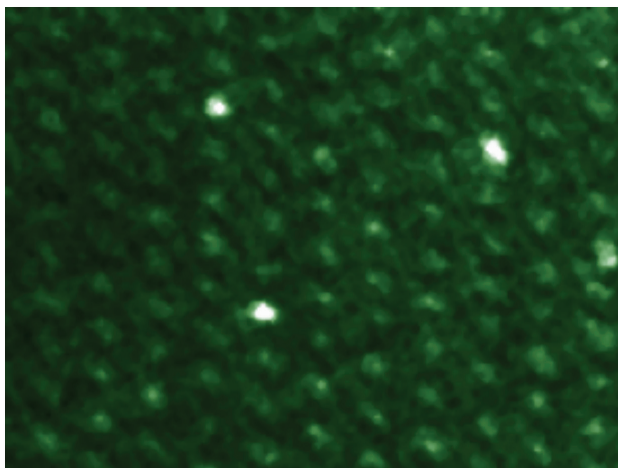
The first example of a "single-atom" catalyst; the three bright spots are platinum atoms on the surface of an iron oxide support material.
