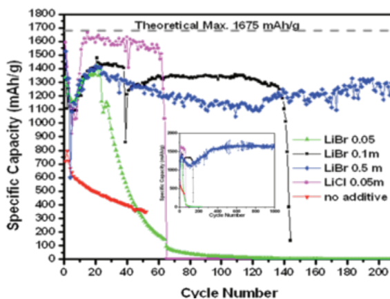
Cycle performance of Li-S batteries with and without electrolyte additives.
