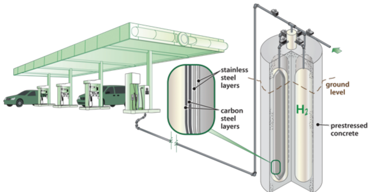
Schematic drawing of ORNL's innovative composite vessel for safe and cost-effective storage of high-pressure hydrogen.
