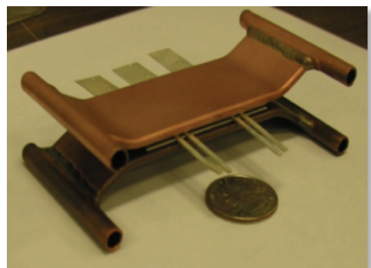
Planar_Bond_All photo showing double-sided planar interconnections and integrated mini-coolers.
