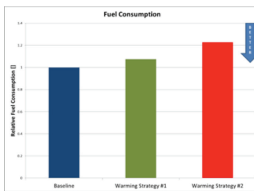
Emissions improvements and fuel penalty associated with vehicle supervisory strategies that prewarm the engine and filter out transient conditions while the engine is cold.
