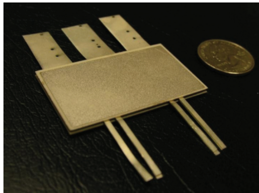
Planar_Bond_All photo showing double-sided planar interconnections.
