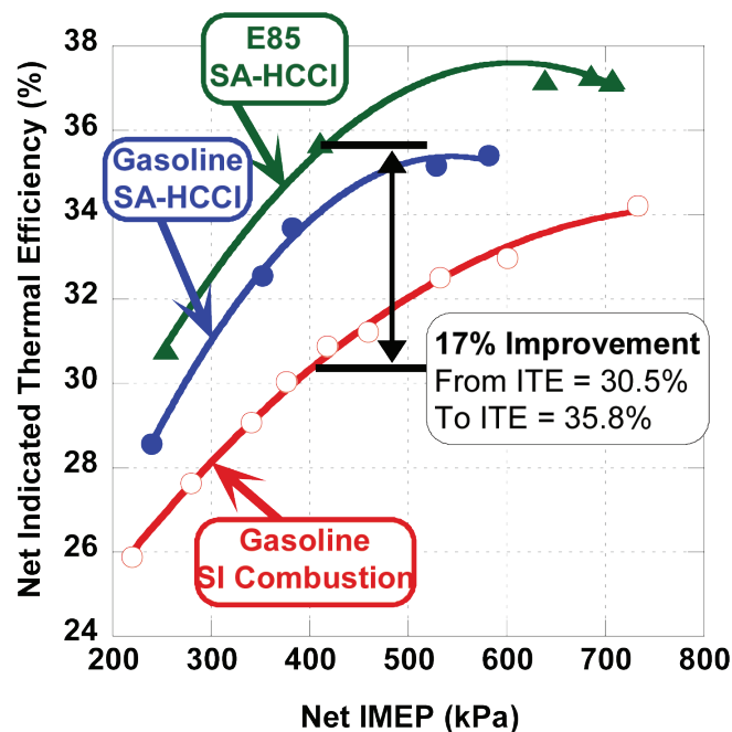
Net indicated thermal efficiency at 2,000 rpm as a function of net IMEP for conventional SI combustion with gasoline and SA-HCCI combustion with gasoline and E85.
