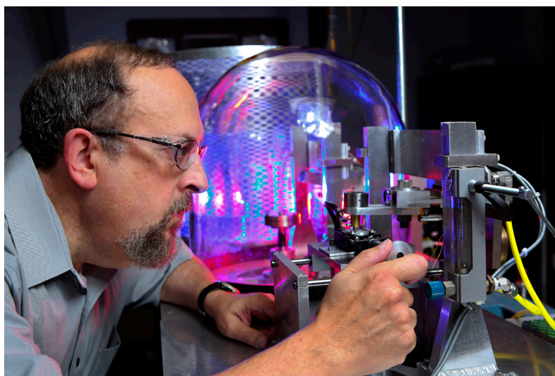
A reciprocating tribometer is used to measure the friction forces between battery materials during repeated charging and discharging.
