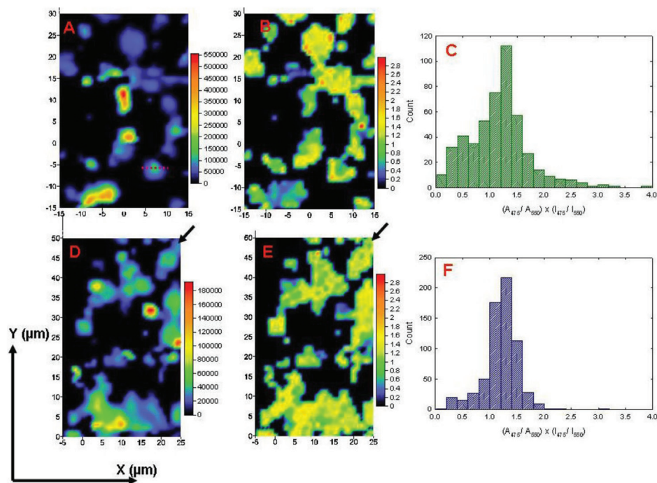
Raman maps showing local SOC variation across NCA electrodes cycled at 4.1 V under constant current condition at 3-C rate with 1 hour potentiostatic step. SOC plots show the local inhomogeneity across the electrode surface and could vary under electrochemical conditions.
