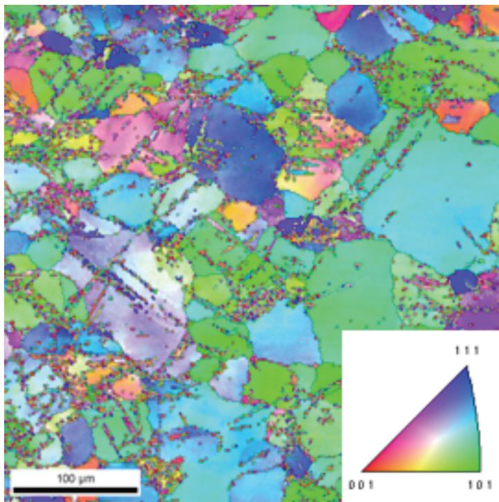
EBSD image showing the microstructure and microtexture of ZEK100 asymmetrically rolled at 150°C after a 5% reduction. The inverse pole figure map (inset) provides a key to the color-crystallographic orientation relationship.
