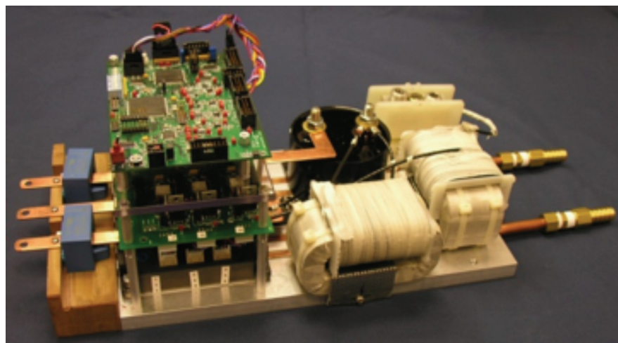
Photo of the 10 kW ZCSI prototype.
