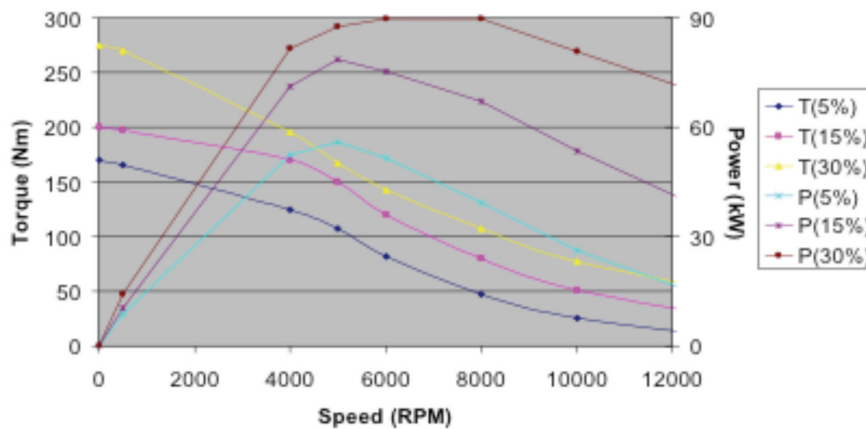
Simulated peak torque and power versus speed for various torque ripple levels.
