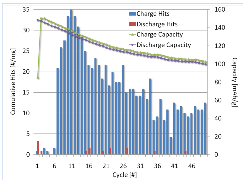
Bar graph of AE activity for each charge and discharge step. A clear majority of events were observed during charging, and a fatigue-type AE activity onset was seen.
