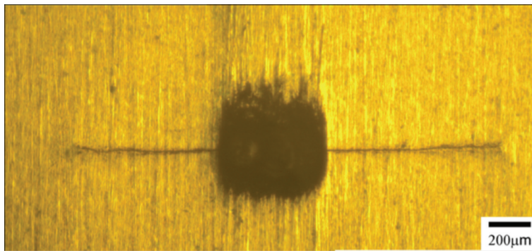
Close up look at the microscope image of a fatigue crack in an AM60 magnesium alloy sample subjected to the Thixomolded® thermomechanical processing heat treatment.
