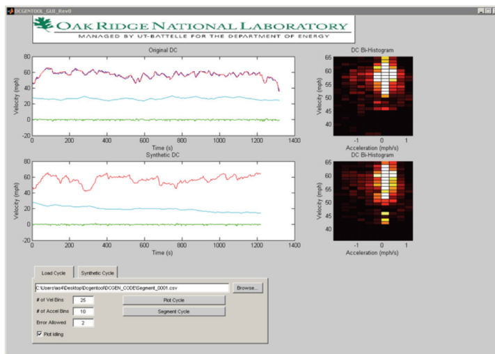
Duty Cycle Generation Tool showing comparison of original (top) and synthetic (bottom) duty cycles
