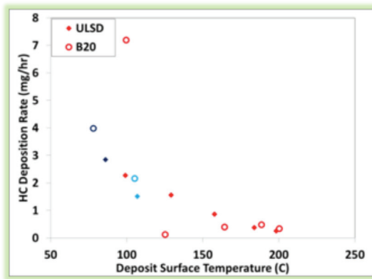
HC deposition rate versus temperature for 0.05 kg/min/tube EGR stream containing 100 ppm HCs.
