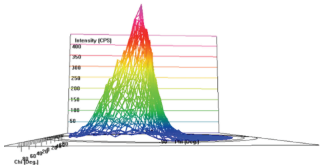
Three-dimensional x-ray pole figures plotting intensity of the (002) or basal planes as a function of azimuthal and tilt angle for the asymmetrically rolled AZ31B.
