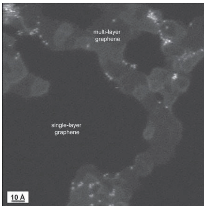
Z-contrast scanning transmission electron microscopy image showing graphene sheet (single- and multi-layered) with individual Pt atoms (brightly imaging) deposited on surface. Note that all the Pt atoms deposit preferentially at the edge sites (or steps where graphene layers overlap) and not on sites associated with the sp^2 -bonded flat (002) surfaces.
