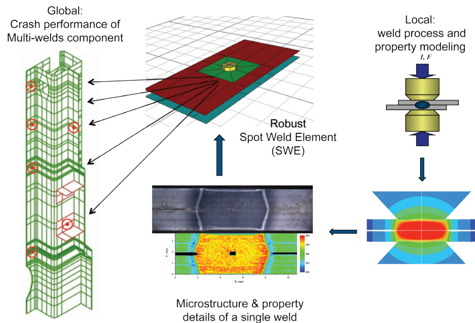
Local-global approach for developing robust spot weld crash simulation framework.
