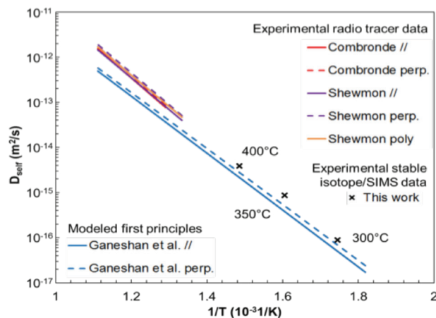
Arrhenius plot of the self-diffusion coefficients in pure Mg using the SIMS-based stable isotope thin-film technique. Comparison with an extrapolation of the published self-diffusion radioactive tracer data at high temperatures (more than 400°C) shows excellent agreement.
