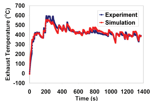
Comparison between predicted and measured coolant temperature and exhaust temperature for the PHEV Prius with a cold start at -7^{\circ}\text{C} .
