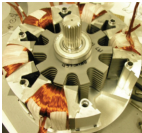
Partially assembled prototype showing yoke-wound stator coils.
