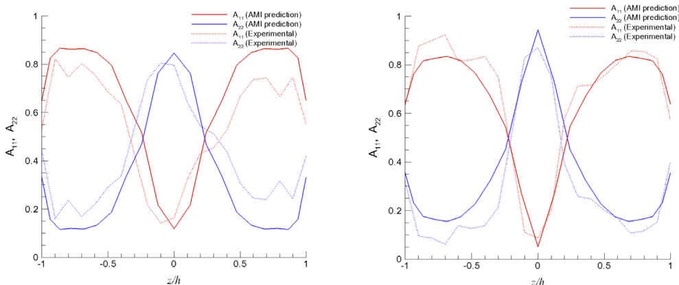
Comparisons of the experimental and predicted fiber orientation results for (left) the 40% slow-fill glass/PP center-gated plaque, worst case; and (right) the 40% fast-fill glass/PA6,6 center-gated plaque, best case. Series designated A11 represent flow direction orientation, and series designated A22 represent cross-flow direction orientation.
