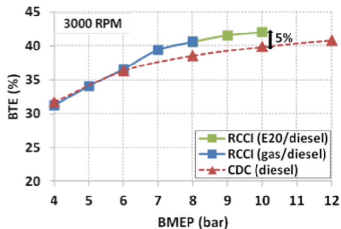
RCCI (blue) using gasoline and diesel compared with conventional diesel (red), showing up to 5% increase in brake thermal efficiency as engine load is increased at 3,000 rpm. The load expansion of RCCI with E20 (20% ethanol, 80% gasoline) is shown in green.
