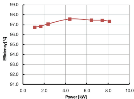
Efficiency chart for the ZCSI prototype, indicating a maximum efficiency of 97.6%.
