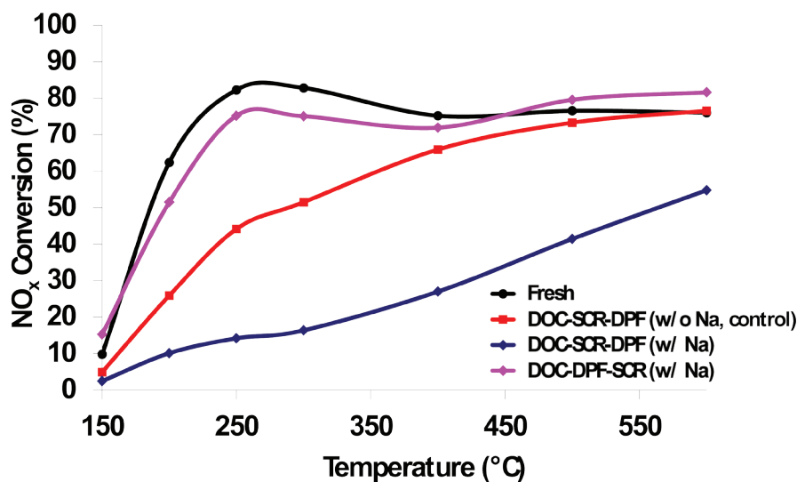
SCR \text{NO}_x reduction performance illustrating the impact of Na in the DOC-SCR-DPF arrangement compared to the minimal effects when the DPF is in front of the SCR (DOC-DPF-SCR).
