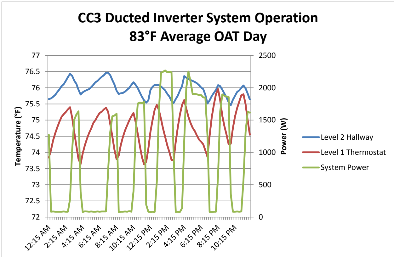
Figure 31: CC3 Ducted Inverter system Operation – 83°F Average OAT Day
