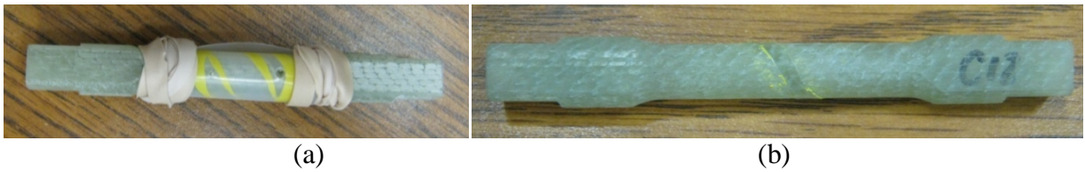
Figure 39. Pictures showing a composite SNTT sample (a) before and (b) after resin infusion.
