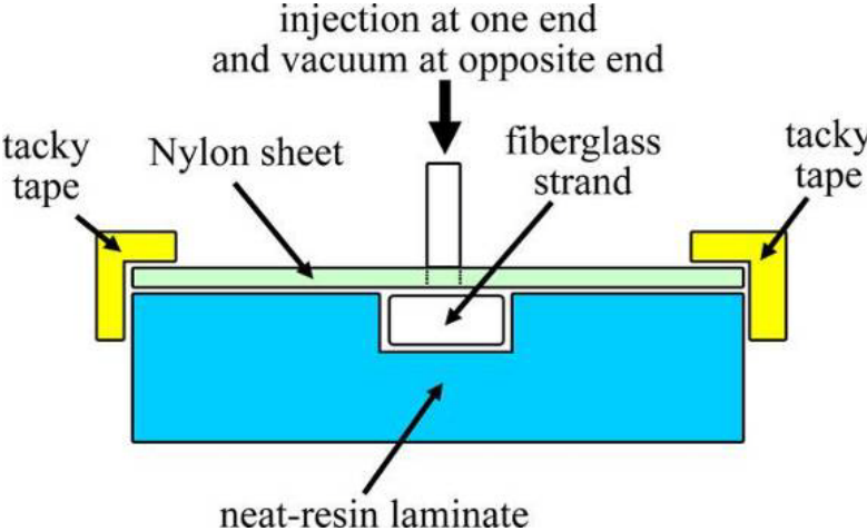
Figure 6. Groove infusion setup
