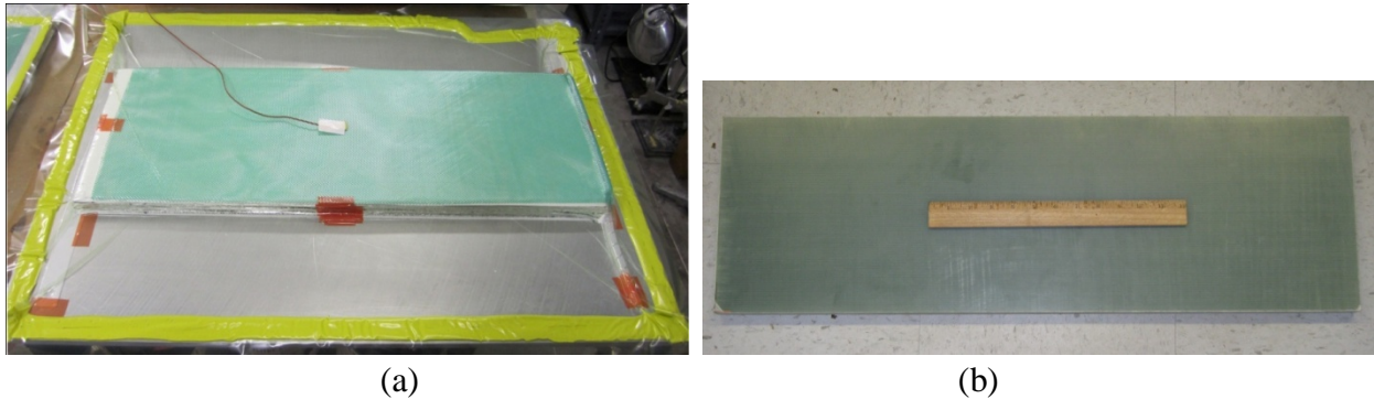
Figure 33. (a) Vacuum assisted infusion process for composite fabrication, and (b) a finished composite plate.
