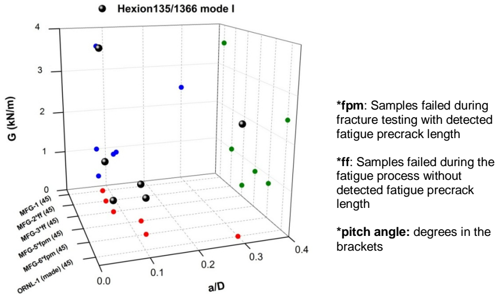
Figure 28. Energy release rates of epoxy Hexion135/1366 at mode I failure
