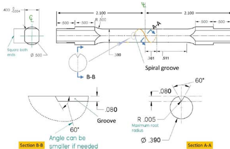
Figure 34. The geometry of the composite SNTT samples.
