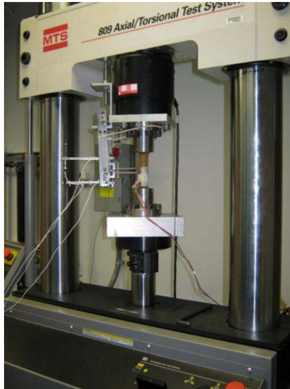
Figure 7. MTS 809 Axial/torsional test system used for SNTT.
