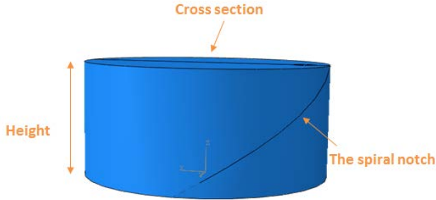
Figure 13. The geometry of the epoxy SNTT model
