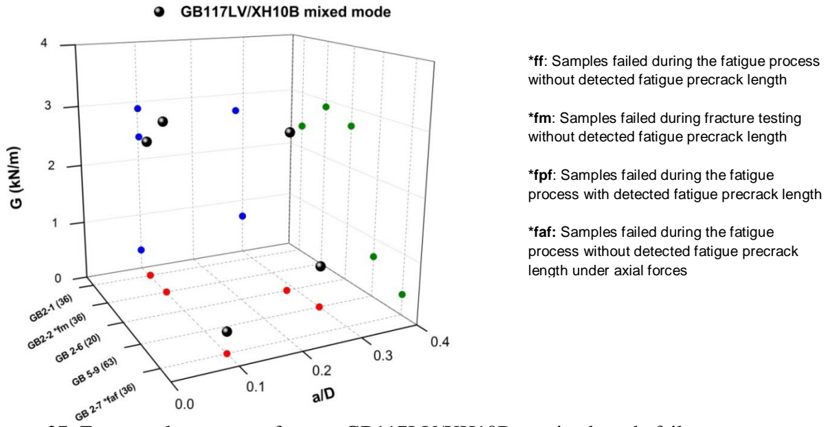
Figure 27. Energy release rates of epoxy GB117LV/XH10B at mixed mode failure
