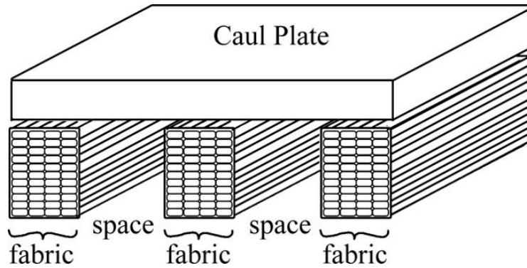
Figure 30. Schematic for sandwich test specimen between the vacuum bag material and the aluminum mold.
