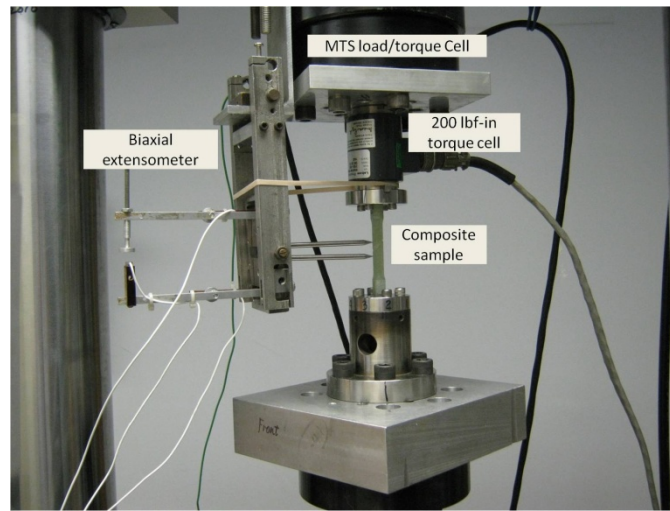
Figure 41. SNTT testing setup of composite bars using a 200 lbf-in torque cell.
