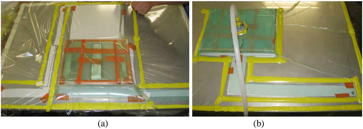
Figure 31. Pictures showing (a) the vacuum-bagging step, and (b) the infusion process. However, this approach was proved to be very difficult. During the infusion process, resin flow entered the exit port leaving a large volume of empty space between the fabric stacks (Figure 32). Lots of air bubbles remained in the infused fabrics. Thus, it was concluded that this approach was not appropriate using the current setup.
