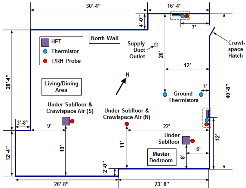
Figure 6. Schematic showing the sensor layout in WC4 crawlspace.
