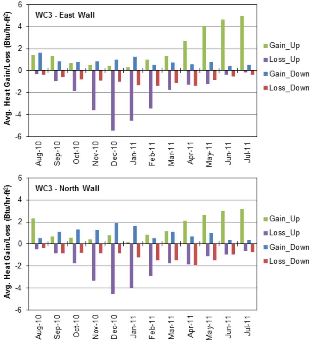
Figure 16. Monthly heat gains and losses through the crawspace walls in WC3.
