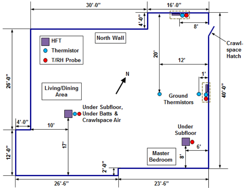
Figure 5. Schematic showing the sensor layout in WC3 crawlspace.
