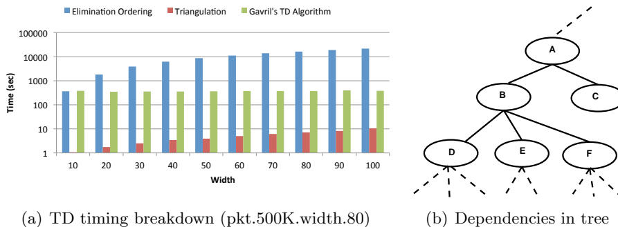
Figure 3: Tree decompositions
