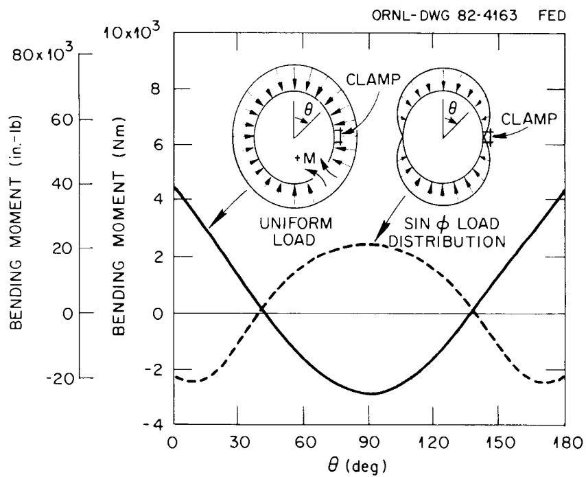
Fig. 6-33(b). Elliptical shell ring bending movements due to clamping loads.
