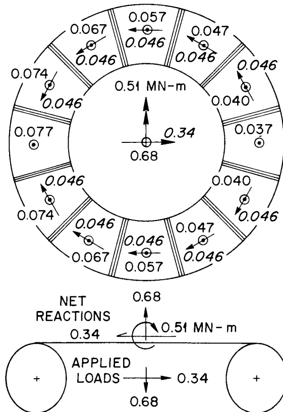
Fig. 6-29. Free body of torus under dead weight and seismic loads.
