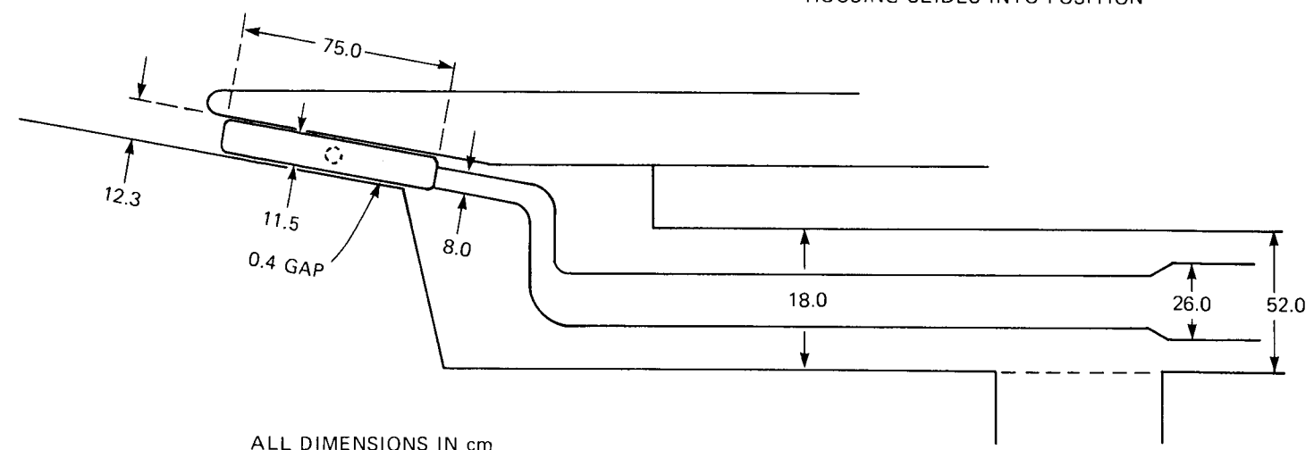
Fig. 4-19(a). Detail of typical diode for FED-A.
