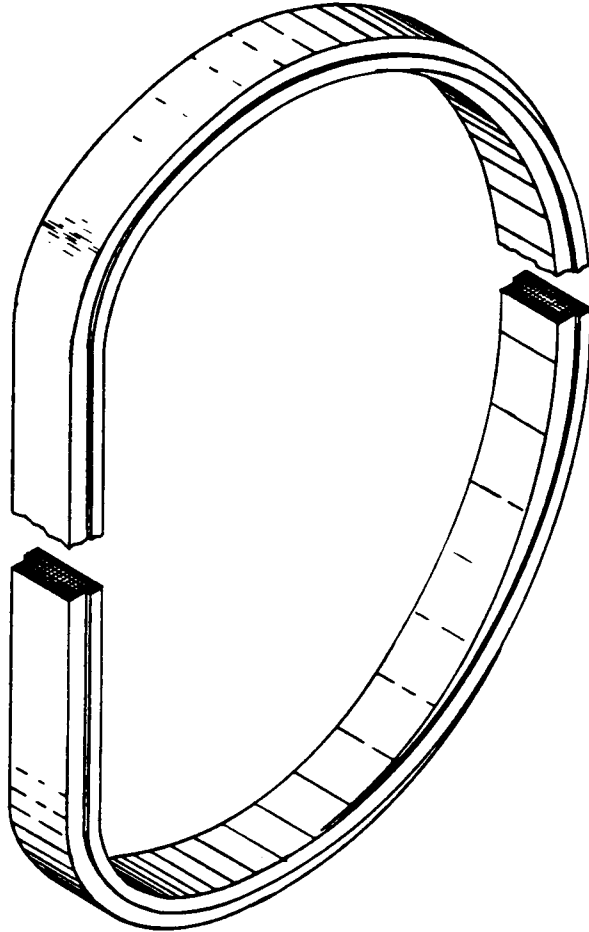
Fig. 8-13. Isometric view of proposed winding configuration.
