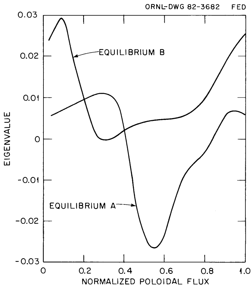
Fig. 3-14. Eigenvalues of the differential equation for n = \infty stability, negative for unstable flux surfaces, are shown for equilibria A and B.
