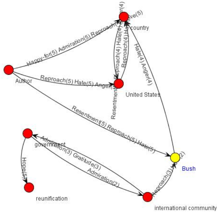
Fig. 13. Benchmark affect-entity diagram for document 20.24.49-8480.
