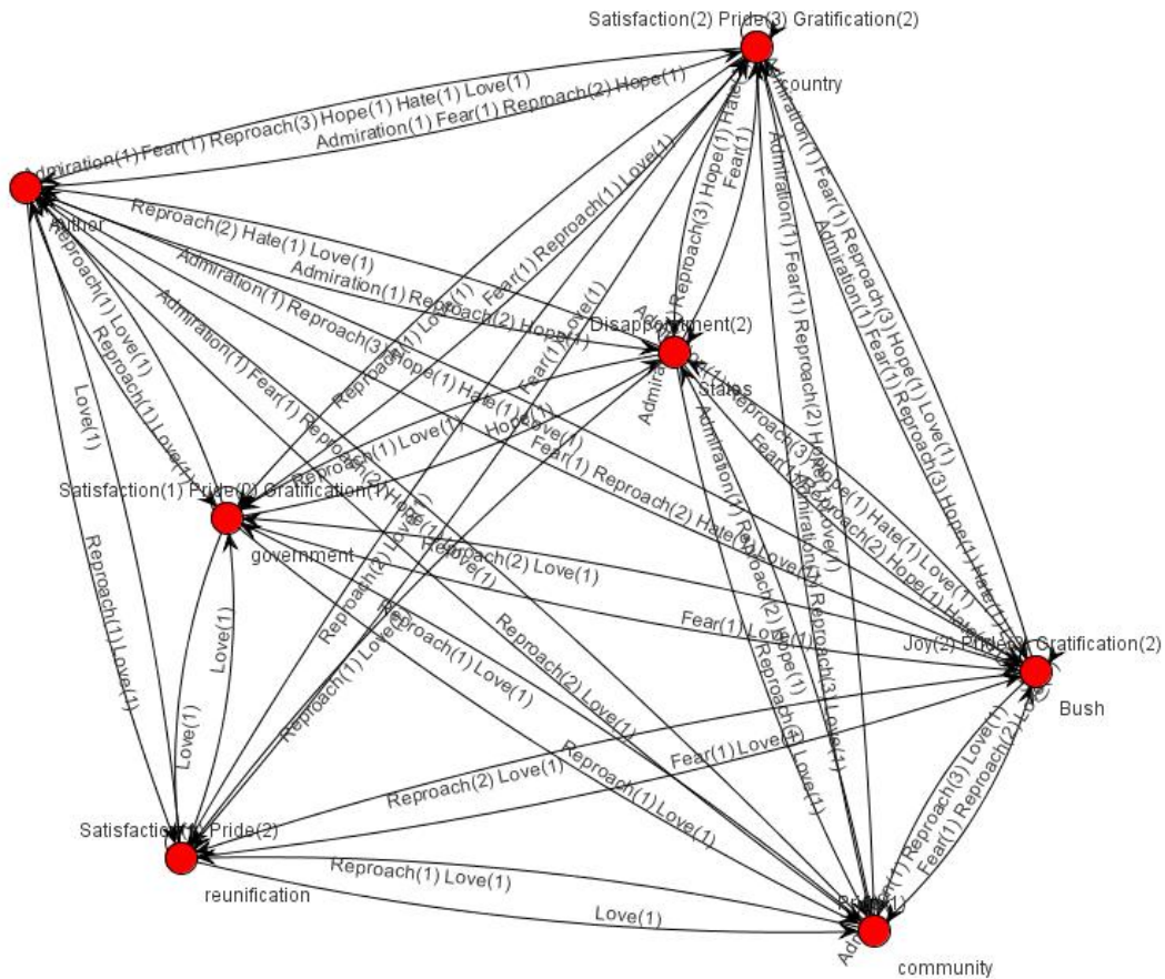
Fig. 14. Affect algorithm (highest fitness - 1379 relations) generated affect-entity diagram for document 20.24.49-8480.
