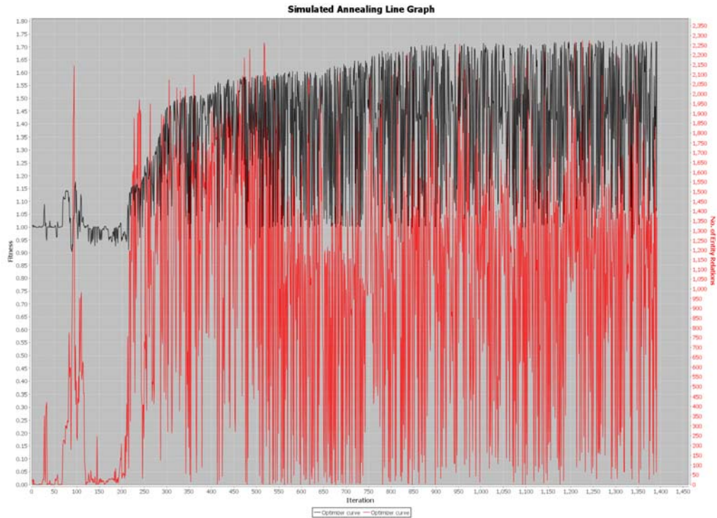
Fig. 11. Fitness results from an initial simulated annealing optimization of the affect propagation algorithm using 50 selected MPQA document annotations.
