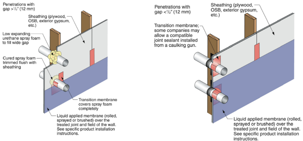
Figure 28. Mechanical penetrations
