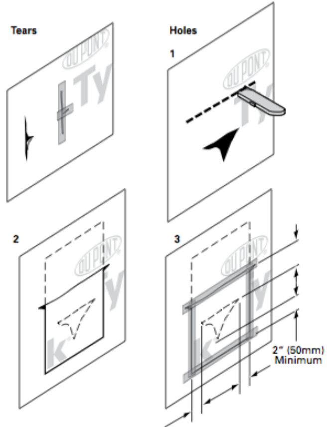
Figure 2. Example manufacturer’s instructions for the repair of tears and holes
