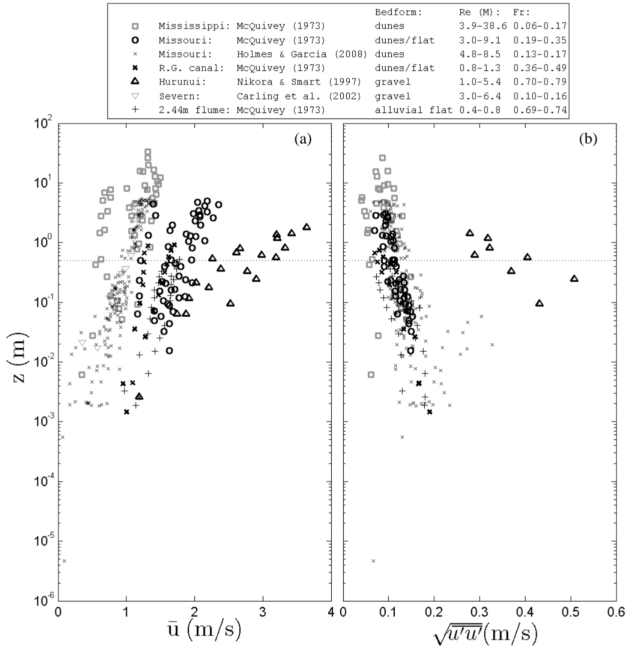
Figure 4. (a) Mean longitudinal velocity profiles. (b) Longitudinal turbulence intensity profiles. The dashed horizontal line indicates z = 0.5 m. HKEC devices will typically operate at depths greater than 0.5m off the bed.
