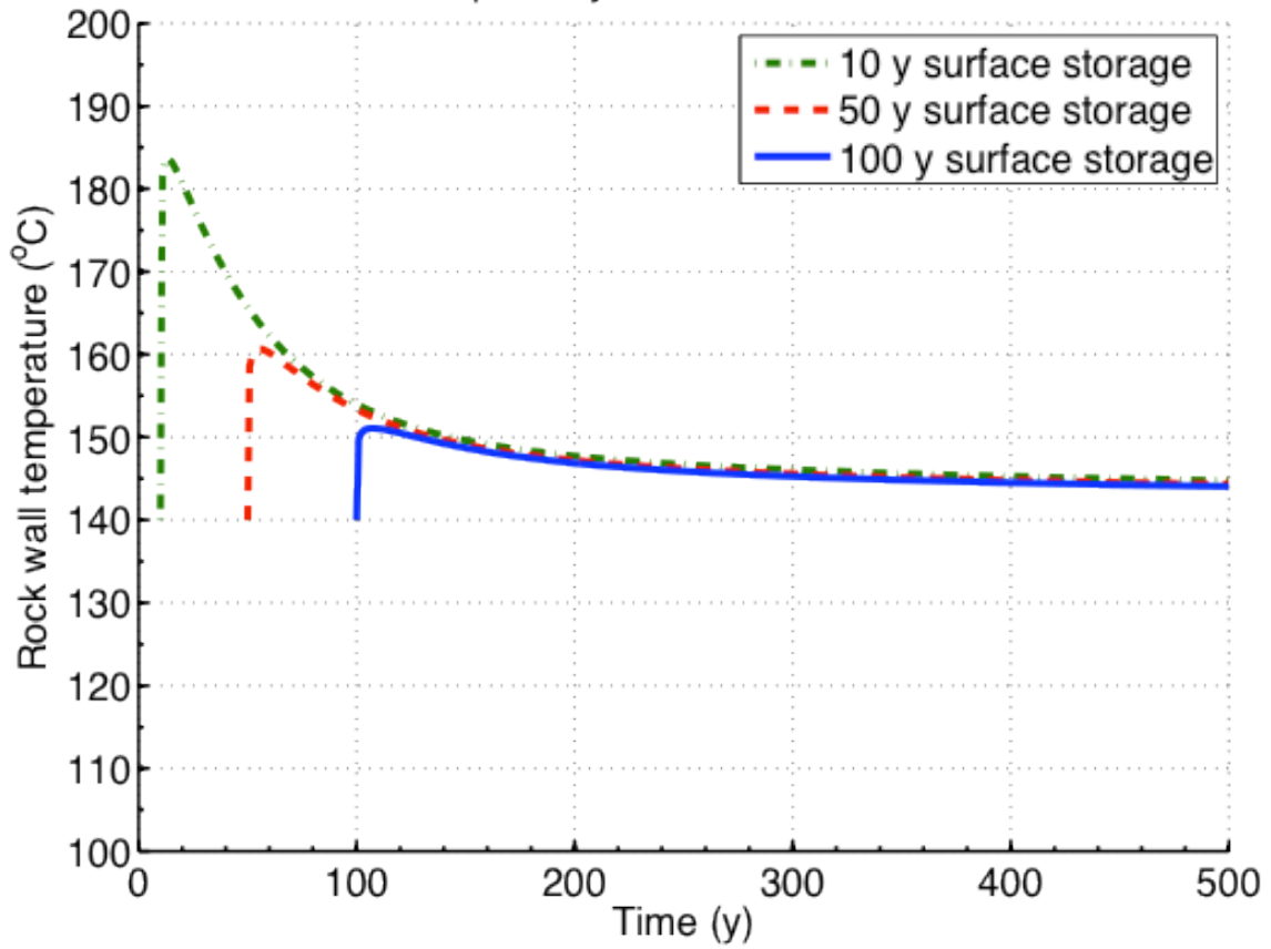
Figure H.3-19 Transient host rock temperature at the calculation radius after storage times of 10, 50 and 100 years for UOX-1 in a deep borehole
