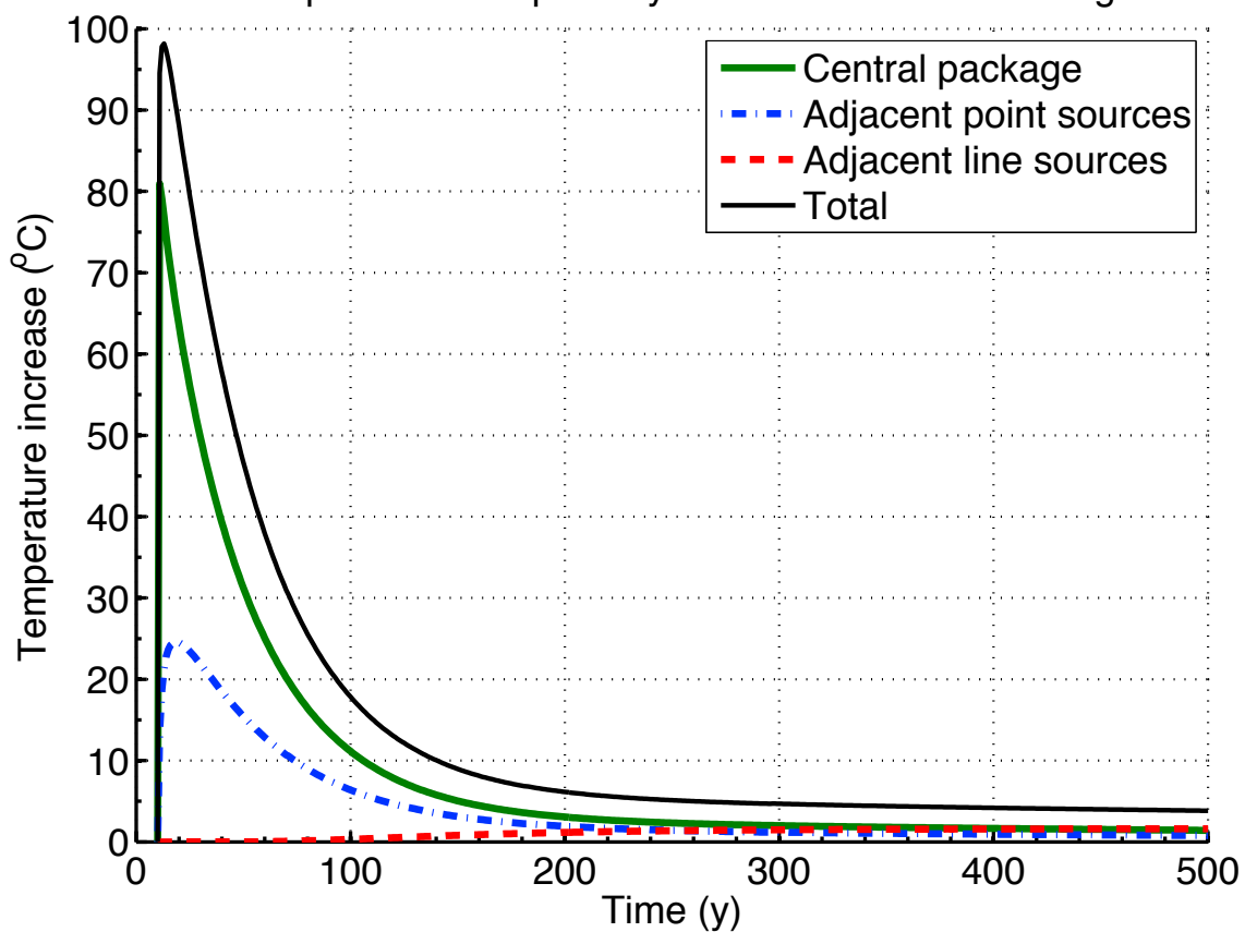
Figure H.2-21 Contributions to the transient rock temperature at the calculation radius from the central package, adjacent point sources and adjacent line sources for one narrow co-extraction (co-extraction-0.291) HLW canister per waste package in a deep borehole. The narrow canister contains 0.291 times the waste in a standard canister
