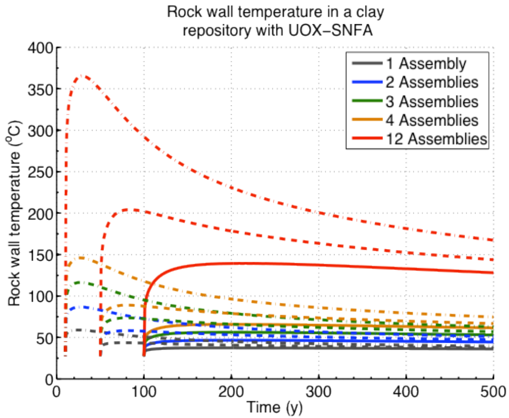
Figure H.3-7 Transient host rock temperature at the calculation radius after storage times of 10, 50 and 100 years for a waste package containing 1, 2, 3, 4 and 12 UOX assemblies in clay
