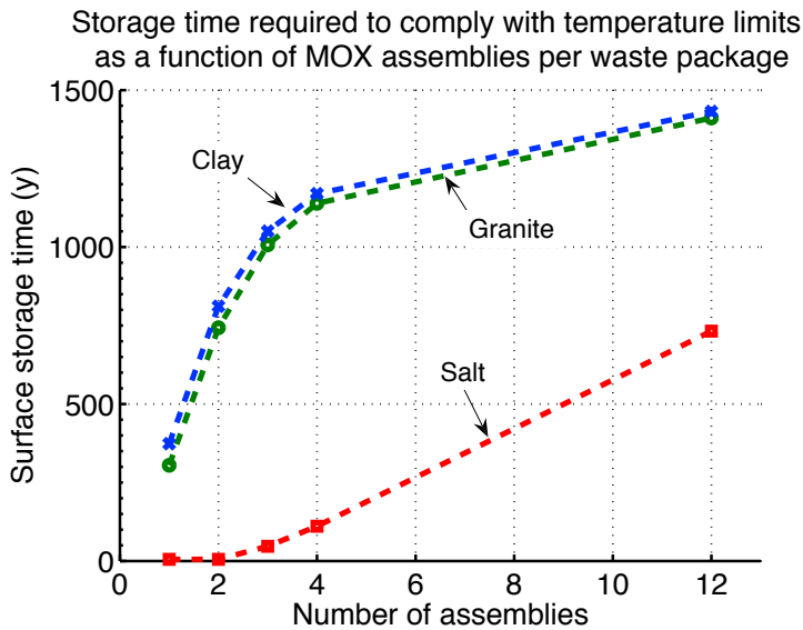
Figure 5.2-8 Minimum surface storage time necessary to comply with waste package surface temperature limit as function of MOX assemblies per waste package in a granite, clay, and salt repository (with 75% of the waste package surface contacting intact salt)
