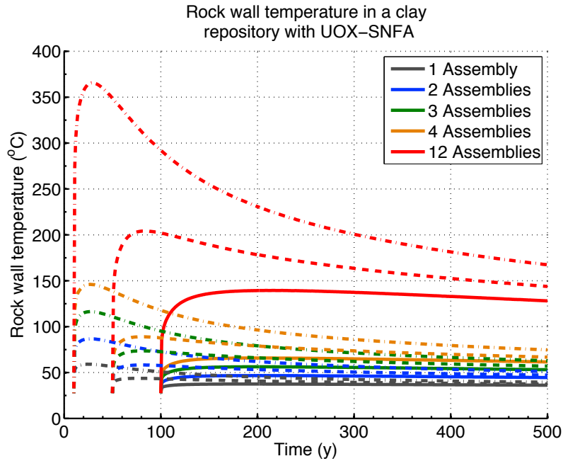
Figure 5.2-3 Transient host rock temperature at the “calculation radius” after storage times of 10, 50 and 100 years for a waste package containing 1, 2, 3, 4 and 12 UOX assemblies per waste package in clay
