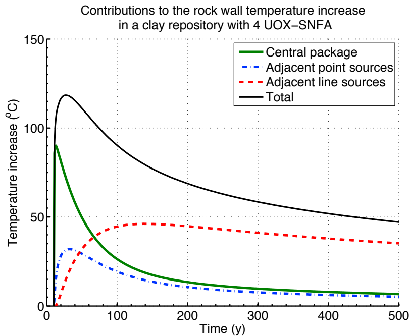
Figure 5.2-4 Contributions to the transient rock temperature at the “calculation radius” from the central package, adjacent point sources and adjacent line sources for 4 UOX assemblies per waste package in clay after 10 years storage
