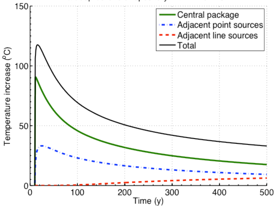
Figure H.2-20 Contributions to the transient rock temperature at the calculation radius from the central package, adjacent point sources and adjacent line sources for MOX-1 in a deep borehole
