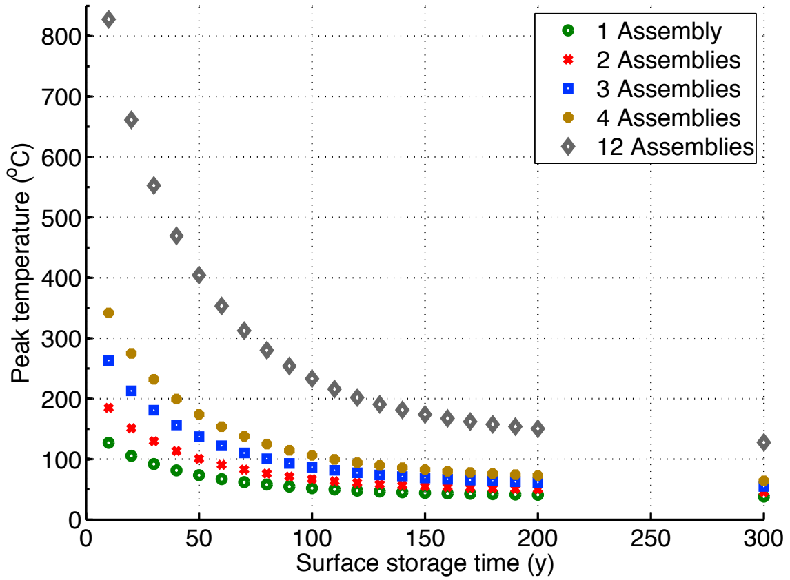
Figure H.5-3 Waste package surface peak temperature as a function of surface storage time for UOX in a clay repository
