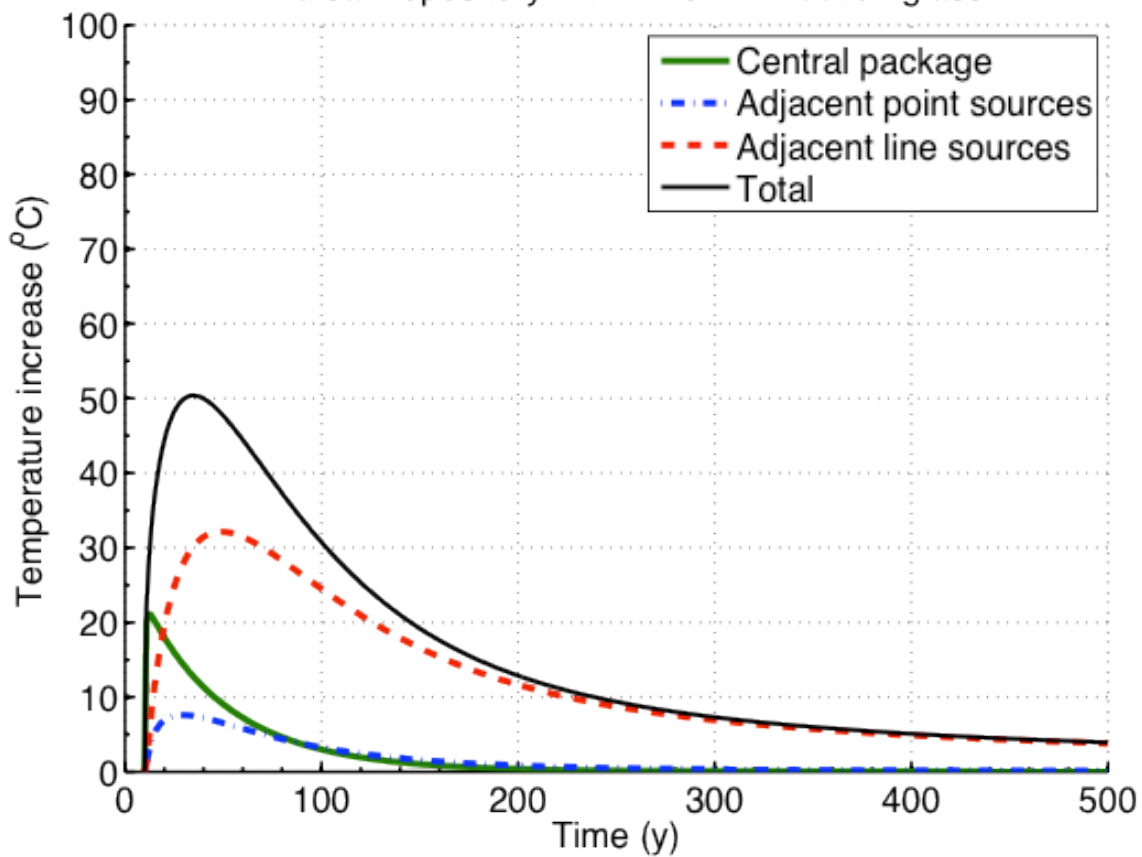
Figure H.2-16 Contributions to the transient rock temperature at the calculation radius from the central package, adjacent point sources and adjacent line sources for new extraction-1 in salt
