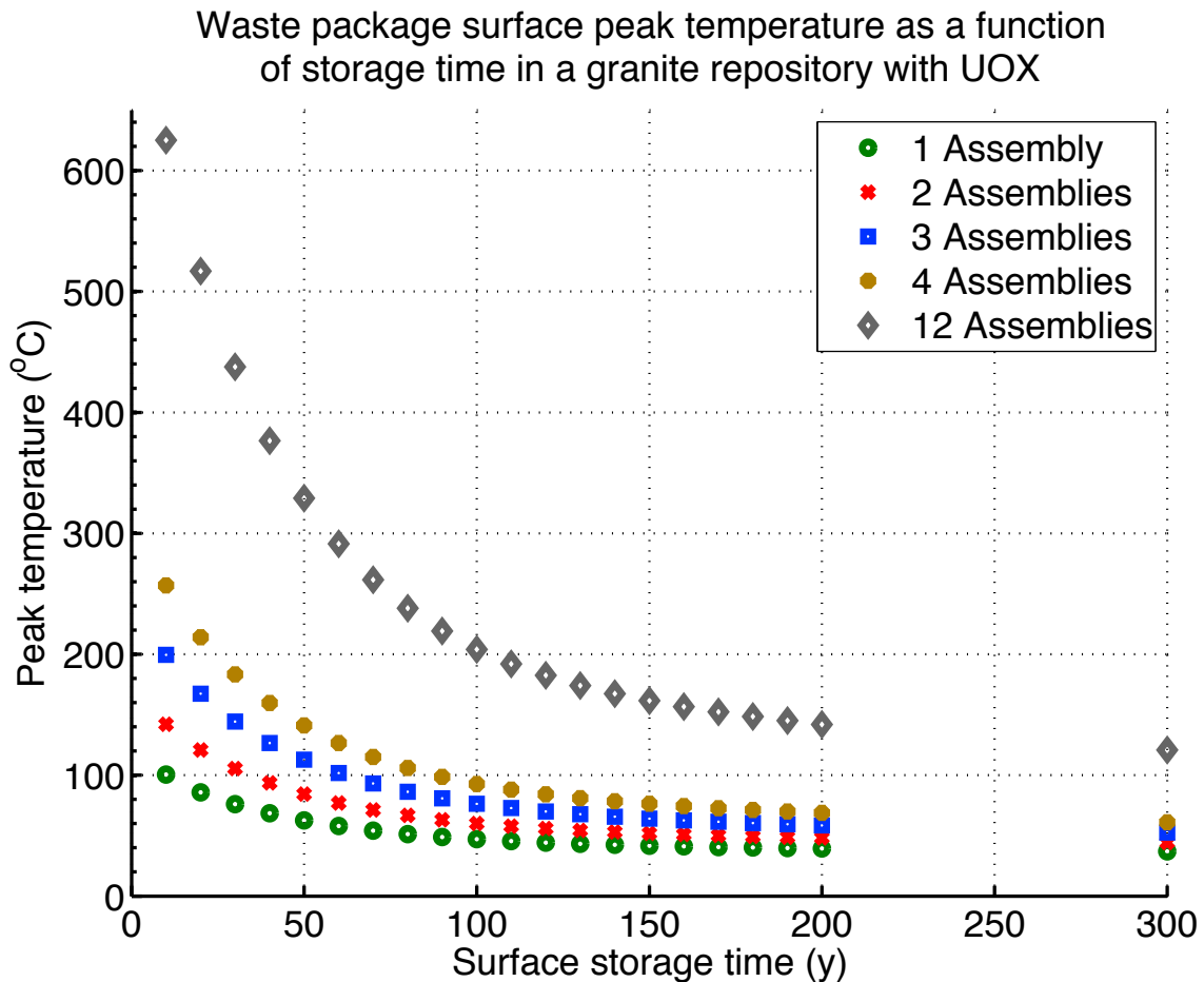
Figure H.5-1 Waste package surface peak temperature as a function of surface storage time for UOX in a granite repository
