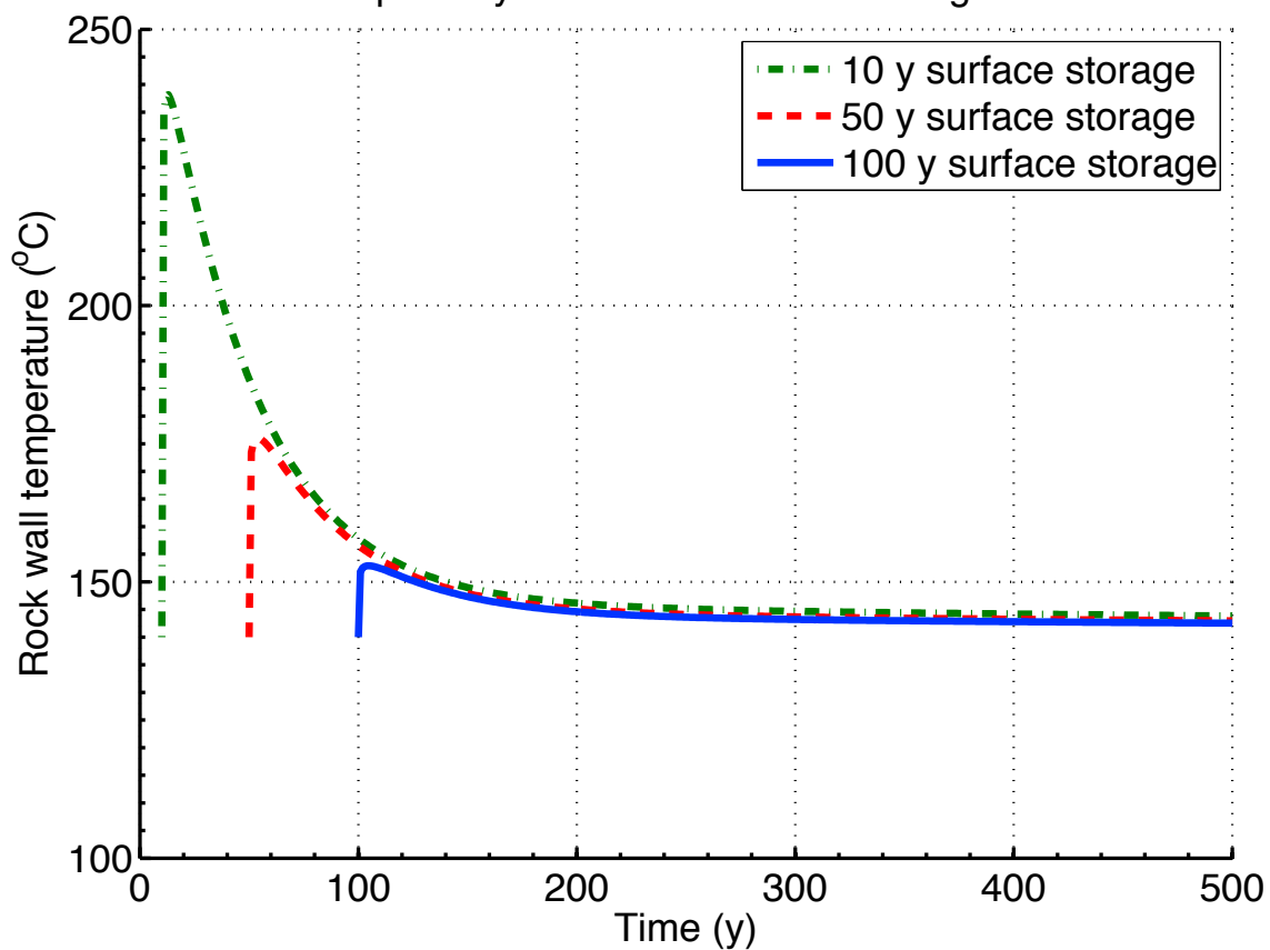
Figure H.3-21 Transient host rock temperature at the calculation radius after storage times of 10, 50 and 100 years for co-extraction-0.291 in a deep borehole
