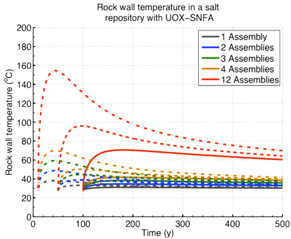
Figure H.3-13 Transient host rock temperature at the calculation radius after storage times of 10, 50 and 100 years for a waste package containing 1, 2, 3, 4 and 12 UOX assemblies in salt
