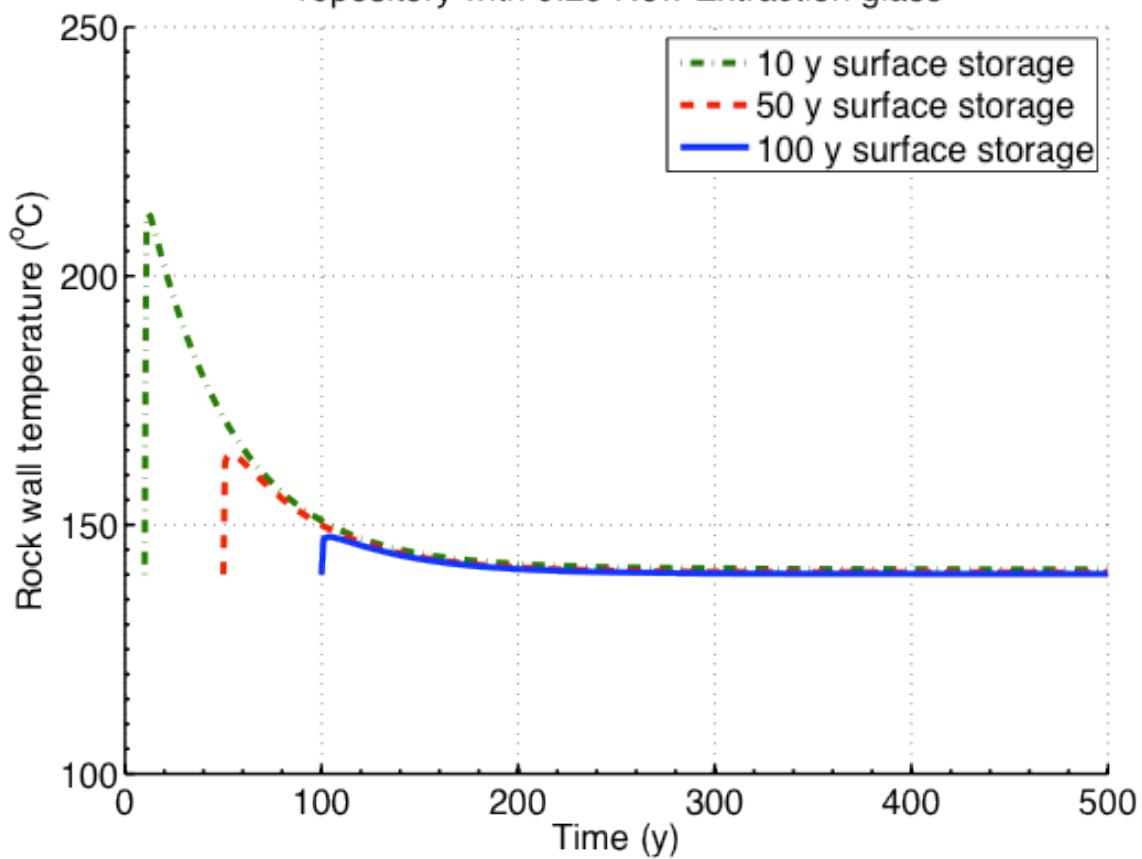
Figure H.3-22 Transient host rock temperature at the calculation radius after storage times of 10, 50 and 100 years for new extraction-0.291 in a deep borehole
