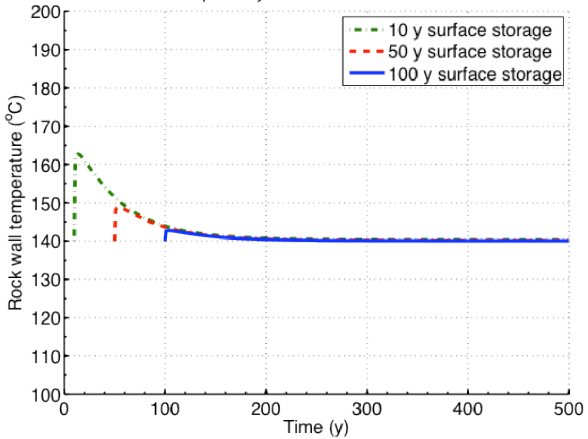
Figure H.3-23 Transient host rock temperature at the calculation radius after storage times of 10, 50 and 100 years for ECC-0.291 in a deep borehole
