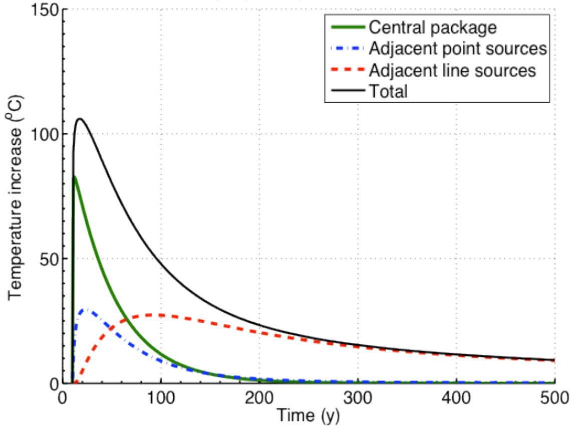
Figure H.2-11 Contributions to the transient rock temperature at the calculation radius from the central package, adjacent point sources and adjacent line sources for ECC-1 in clay
