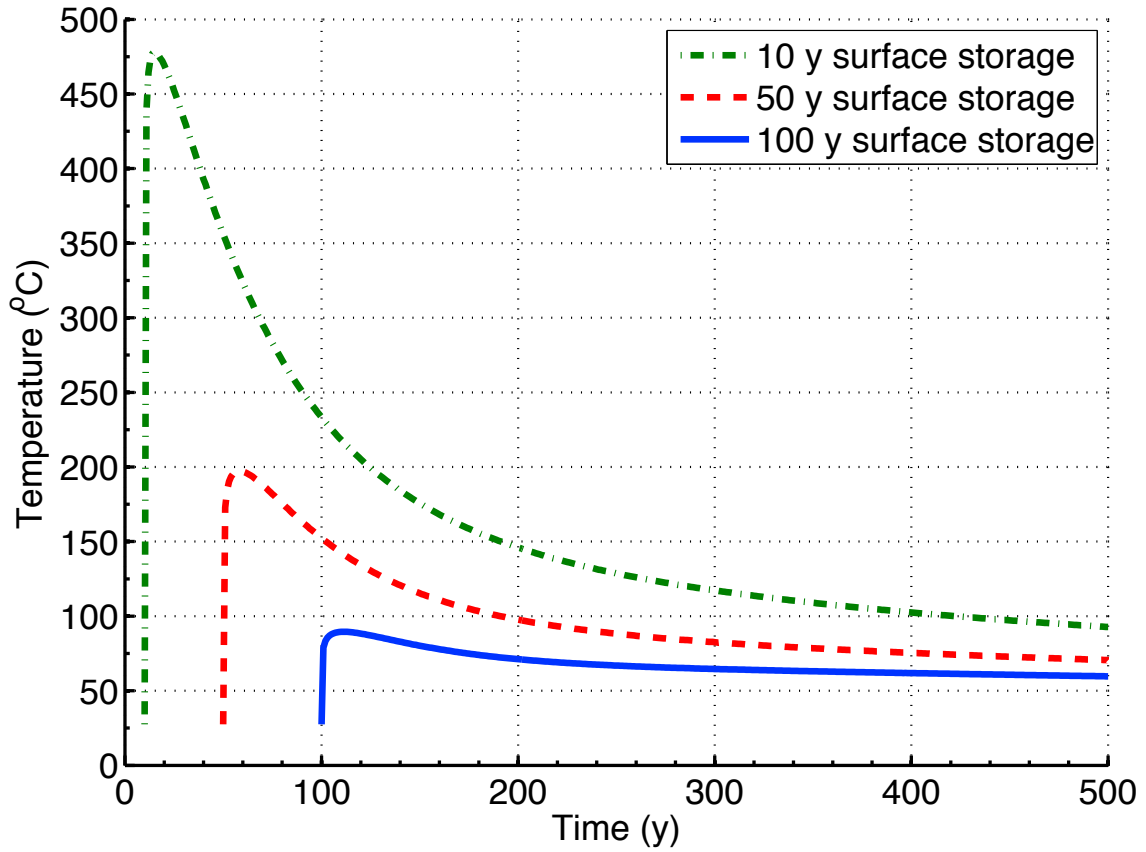
Figure H.4-9 Calculated waste package temperature after storage times of 10, 50 and 100 years for co-extraction-1 in clay
