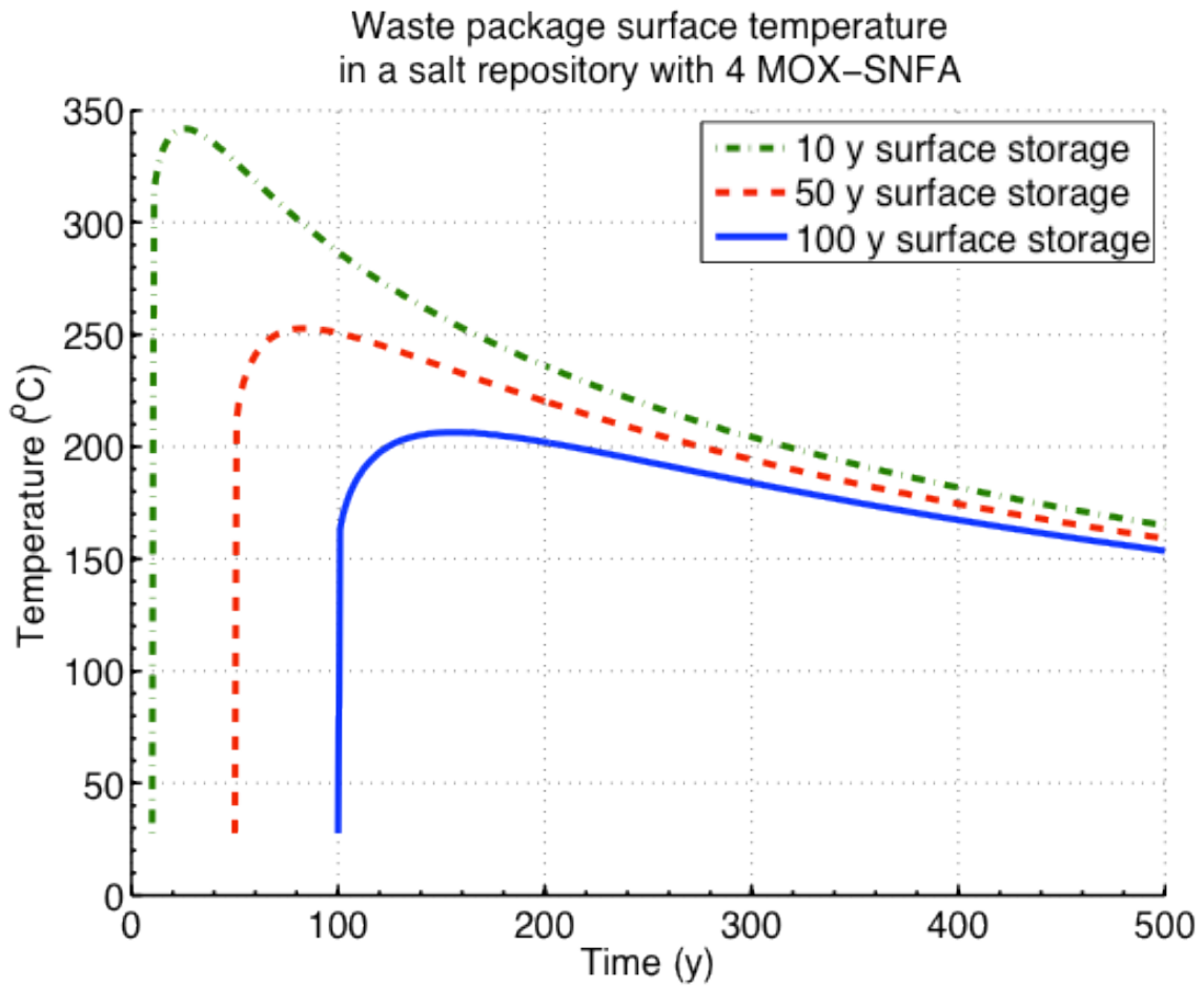
Figure H.4-14 Calculated waste package temperature after storage times of 10, 50 and 100 years for MOX-4 in salt, with 75% of the waste package surface contacting intact salt
