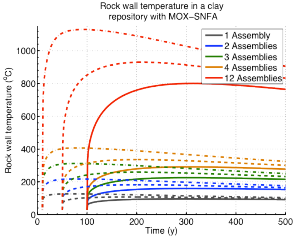
Figure H.3-8 Transient host rock temperature at the calculation radius after storage times of 10, 50 and 100 years for a waste package containing 1, 2, 3, 4 and 12 MOX assemblies in clay
