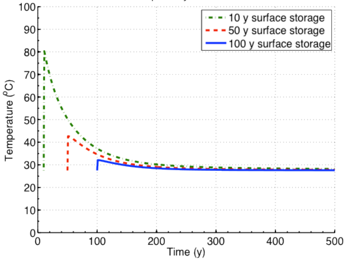
Figure H.4-18 Calculated waste package temperature after storage times of 10, 50 and 100 years for ECM-1 in salt, with 75% of the waste package surface contacting intact salt
