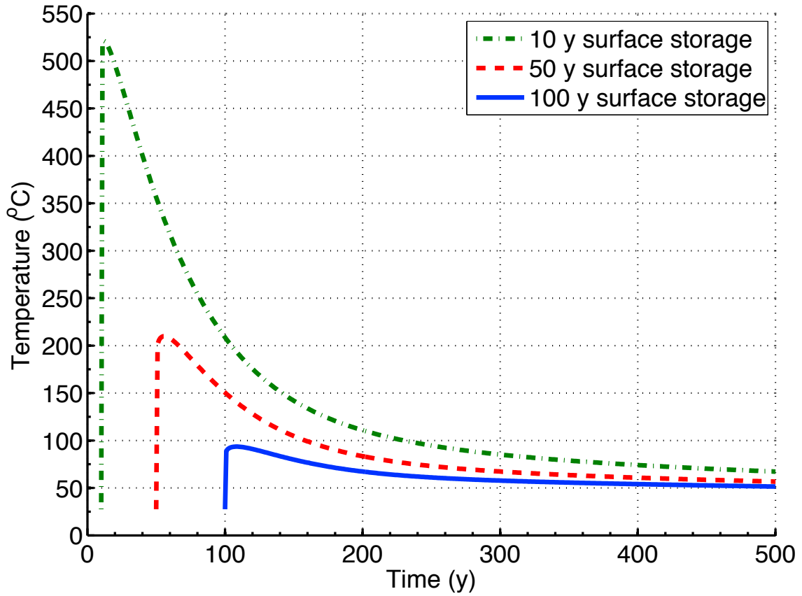
Figure H.4-3 Calculated waste package temperature after storage times of 10, 50 and 100 years for co-extraction-1 in granite
