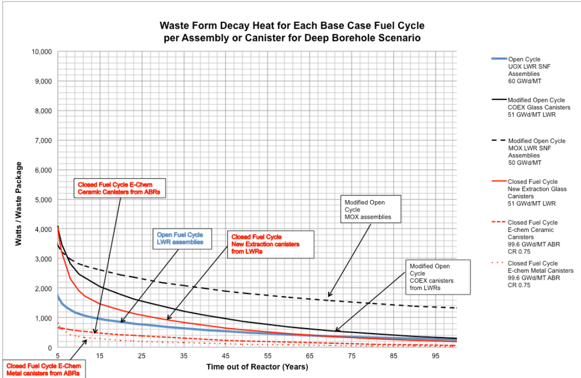
Figure 5.1-8 Decay heat curves for 1 UOX or MOX assembly and 0.291 co-extraction, new extraction, EC-ceramic or EC-metal canister per waste package (deep borehole design)
