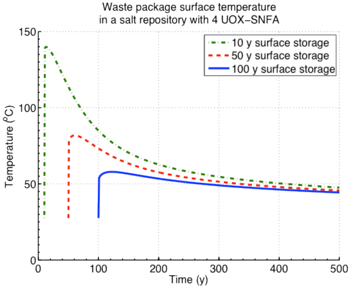
Figure H.4-13 Calculated waste package temperature after storage times of 10, 50 and 100 years for UOX-4 in salt, with 75% of the waste package surface contacting intact salt
