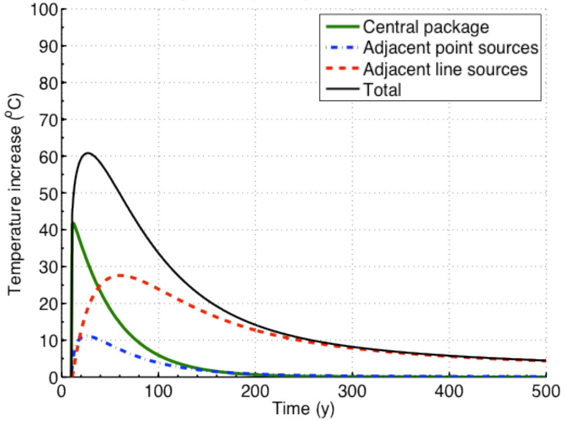
Figure H.2-5 Contributions to the transient rock temperature at the calculation radius from the central package, adjacent point sources and adjacent line sources for one EC-Ceramic HLW (ECC-1) canister per waste package in granite
