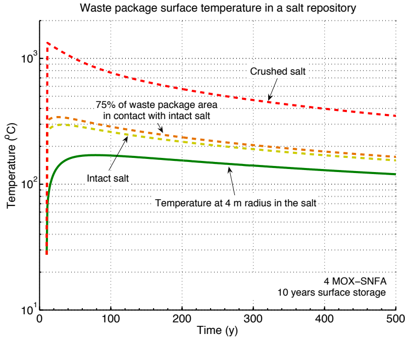
Figure 5.2-4 Calculated waste package temperature after 10 years storage time for 4 MOX assemblies per canister in salt assuming the waste package is in contact with crushed salt or intact salt, either fully or for 75% of its area
