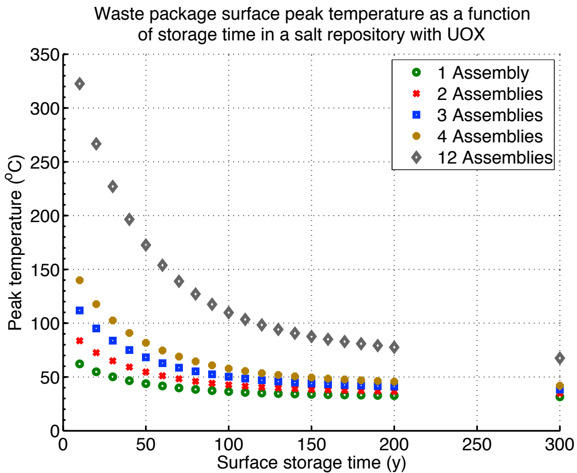
Figure H.5-5 Waste package surface peak temperature as a function of surface storage time for UOX in a salt repository with 75% of the waste package surface contacting intact salt
