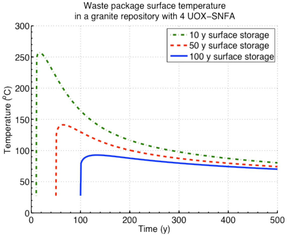
Figure H.4-1 Calculated waste package temperature after storage times of 10, 50 and 100 years for UOX-4 in granite
