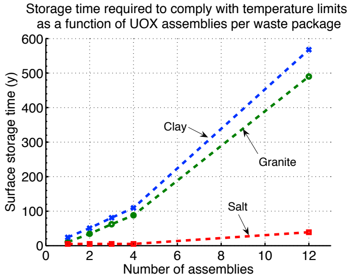
Figure 5.2-7 Minimum surface storage time necessary to comply with waste package surface temperature limit as function of UOX assemblies per waste package in a granite, clay, and salt repository (with 75% of the waste package surface contacting intact salt)
