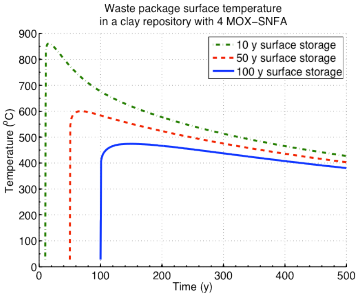
Figure H.4-8 Calculated waste package temperature after storage times of 10, 50 and 100 years for MOX-4 in clay
