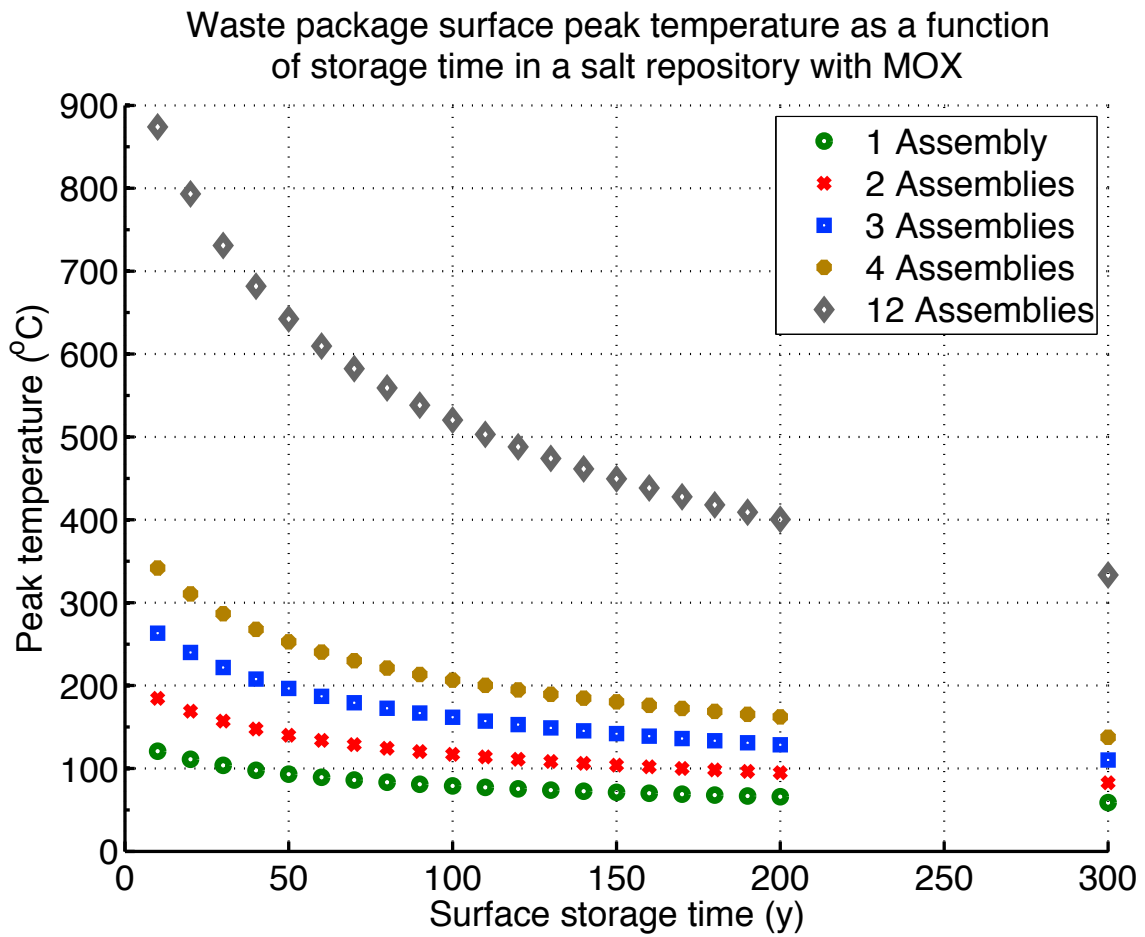
Figure H.5-6 Waste package surface peak temperature as a function of surface storage time for MOX in a salt repository with 75% of the waste package surface contacting intact salt
