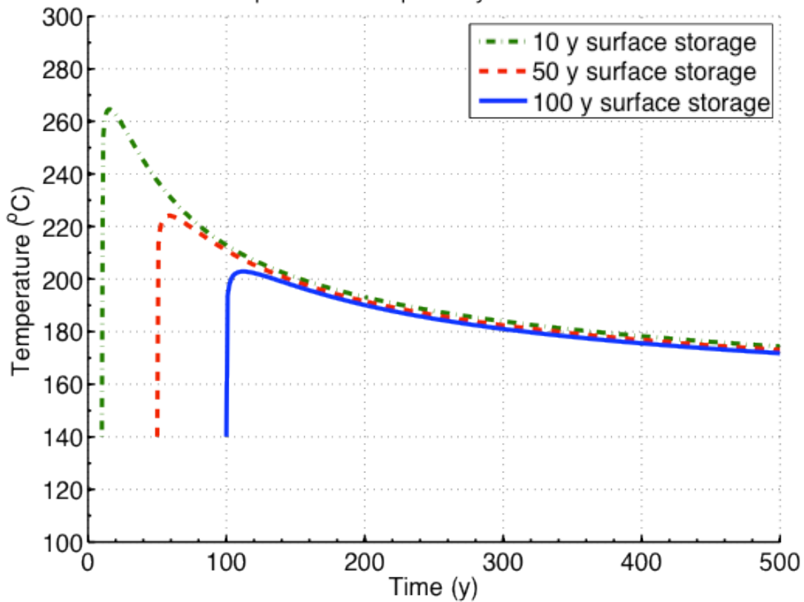
Figure H.4-20 Calculated waste package temperature after storage times of 10, 50 and 100 years for MOX-1 in a deep borehole
