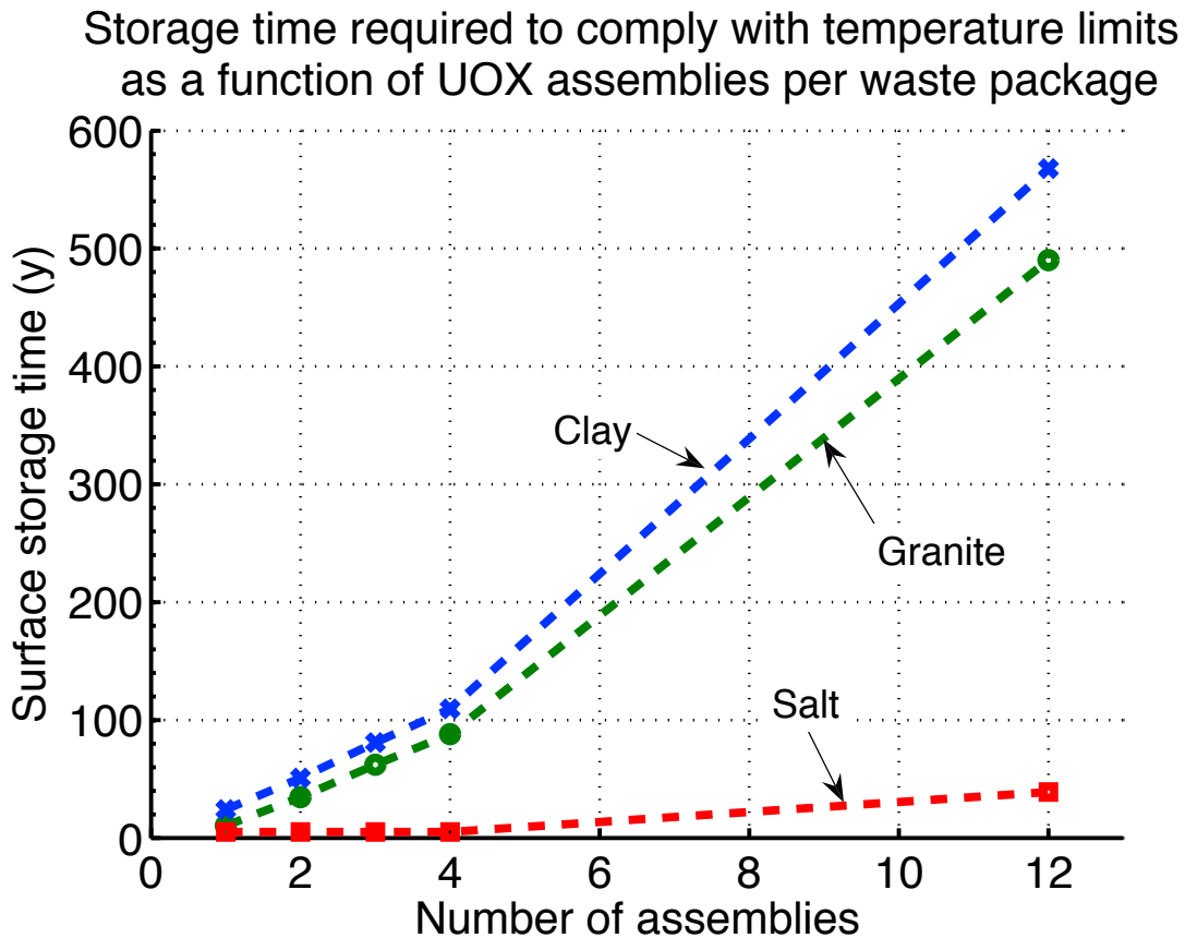
Figure H.6-1 Minimum surface storage time necessary to comply with waste package surface temperature limit as function of UOX assemblies per waste package in a granite, clay, and salt (with 75% of the waste package surface contacting intact salt) repository
