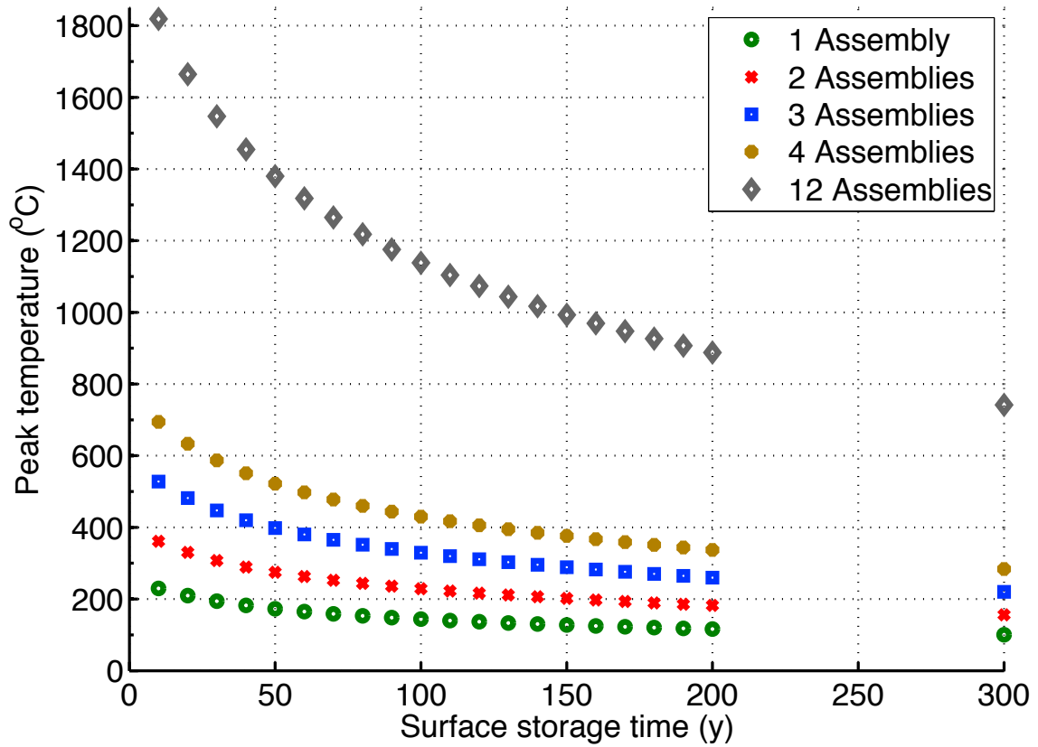
Figure H.5-2 Waste package surface peak temperature as a function of surface storage time for MOX in a granite repository
