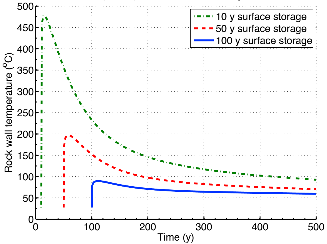
Figure H.3-9 Transient host rock temperature at the calculation radius after storage times of 10, 50 and 100 years for co-extraction-1 in clay
