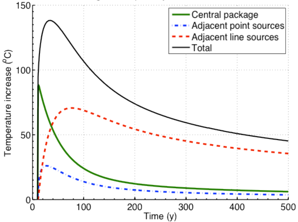
Figure H.2-1 Contributions to the transient rock temperature at the calculation radius from the central package, adjacent point sources and adjacent line sources for 4 UOX assemblies per waste package (UOX-4) in granite
