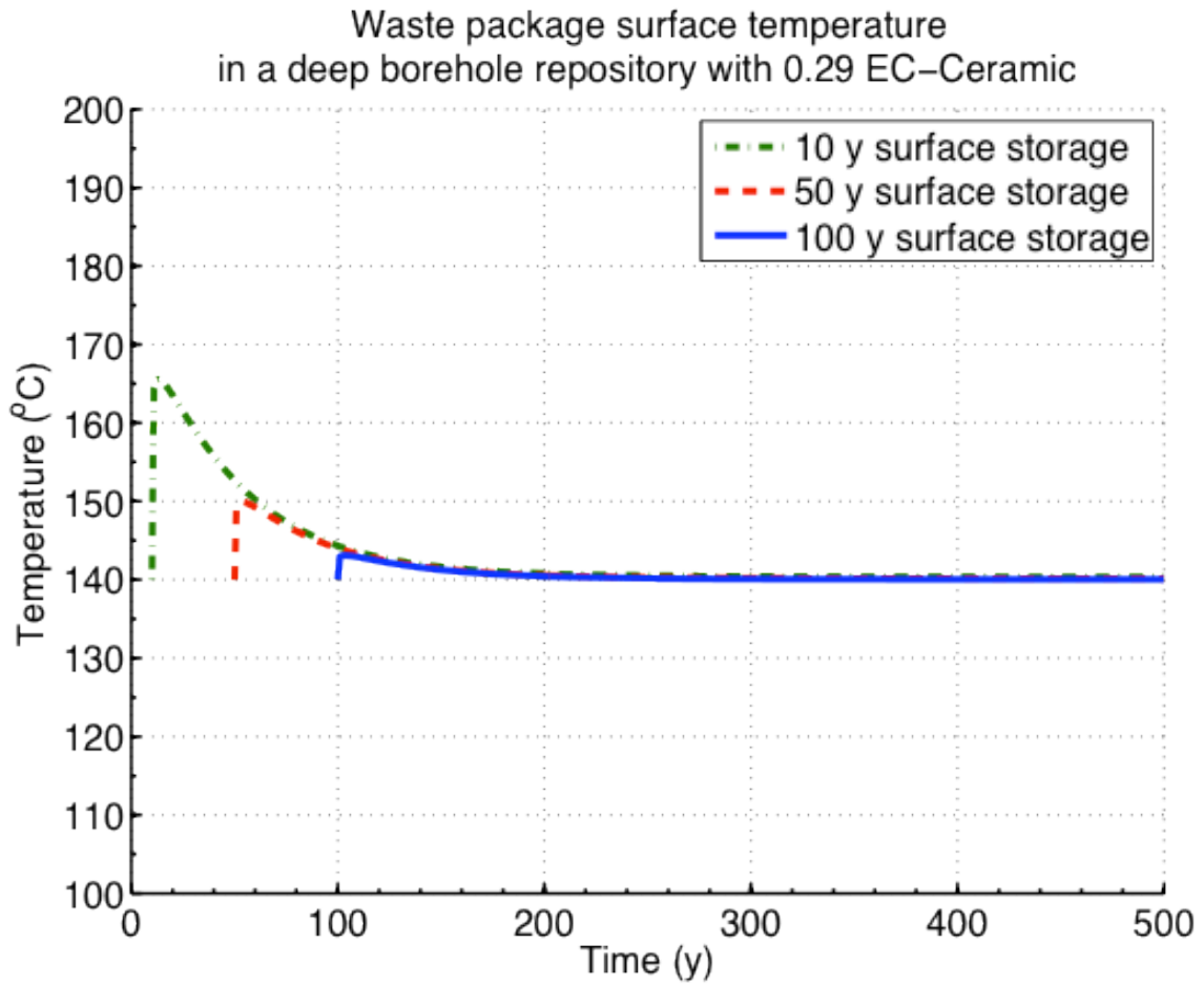
Figure H.4-23 Calculated waste package temperature after storage times of 10, 50 and 100 years for ECC-0.291 in a deep borehole
