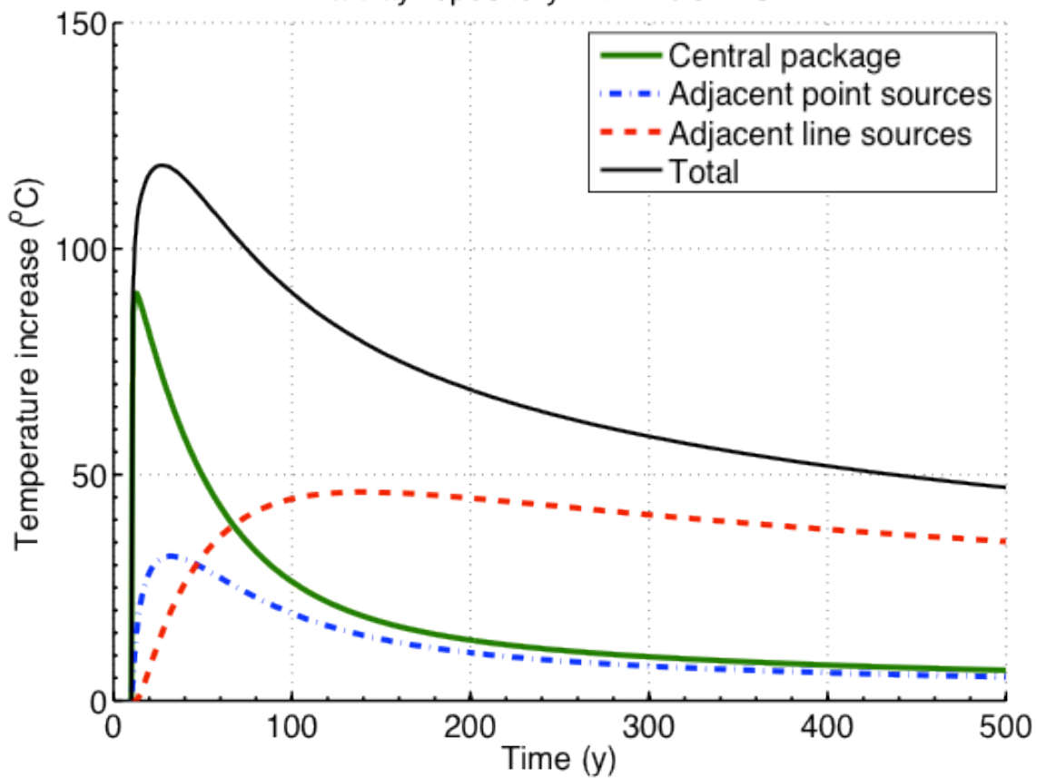
Figure H.2-7 Contributions to the transient rock temperature at the calculation radius from the central package, adjacent point sources and adjacent line sources for UOX-4 in clay
