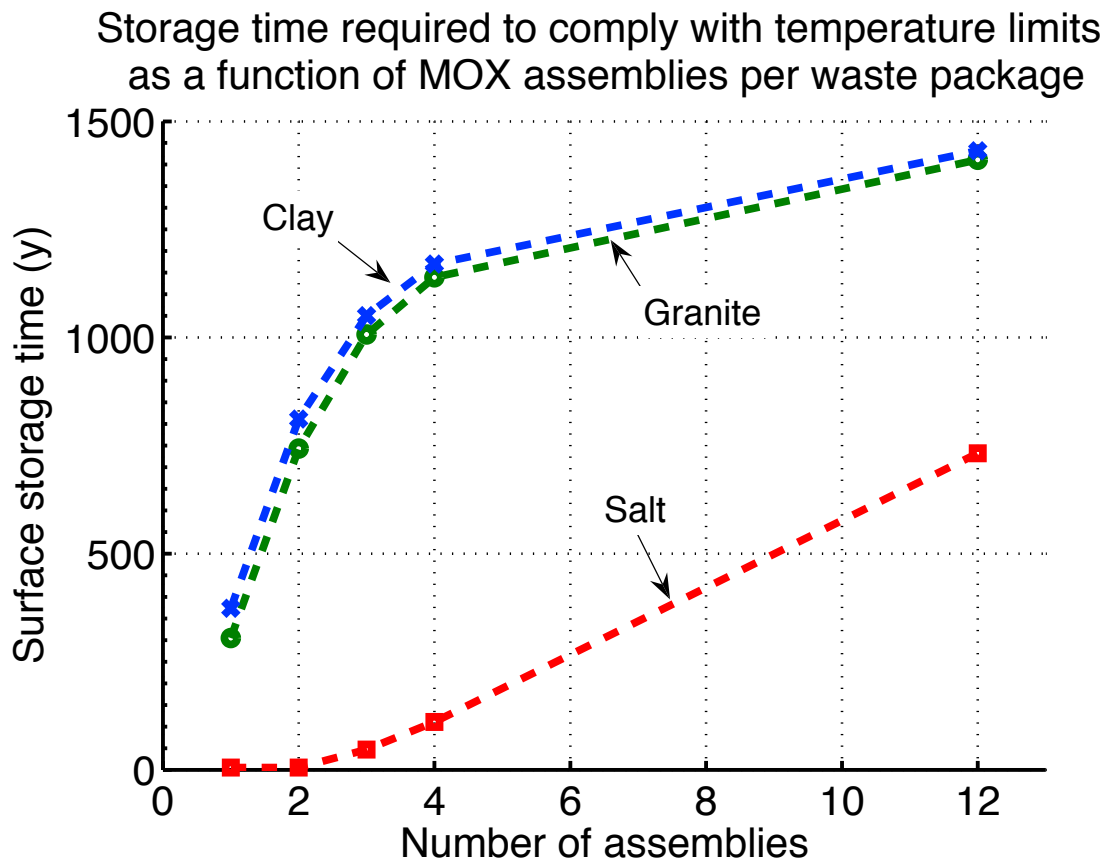
Figure H.6-2 Minimum surface storage time necessary to comply with waste package surface temperature limit as function of MOX assemblies per waste package in a granite, clay, and salt (with 75% of the waste package surface contacting intact salt) repository
