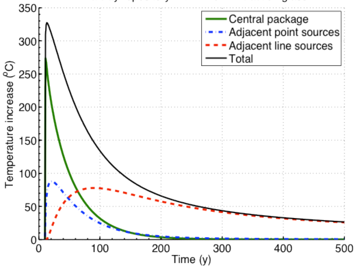
Figure H.2-10 Contributions to the transient rock temperature at the calculation radius from the central package, adjacent point sources and adjacent line sources for new extraction-1 in clay
