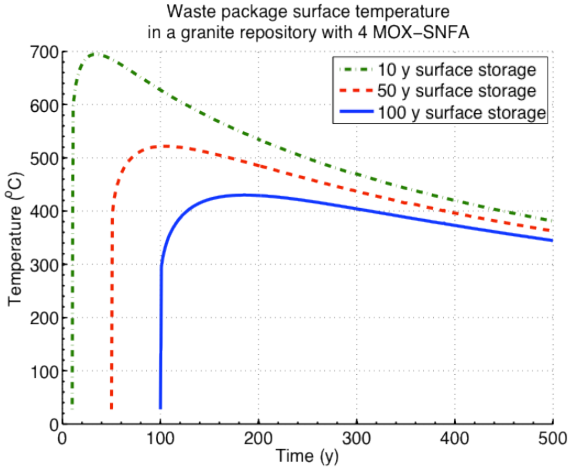
Figure H.4-2 Calculated waste package temperature after storage times of 10, 50 and 100 years for MOX-4 in granite
