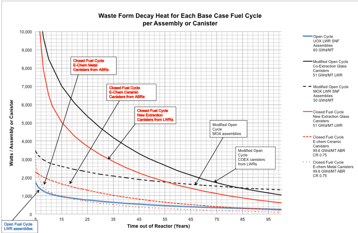
Figure 5.1-7 Decay heat curves for 1 assembly or 1 canister per waste package for UOX, MOX, co-extraction, new extraction, EC-ceramic, and EC-metal
