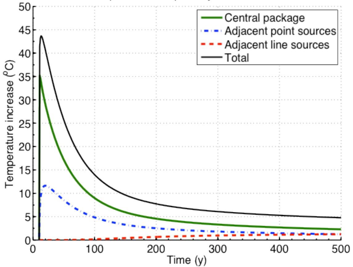
Figure H.2-19 Contributions to the transient rock temperature at the calculation radius from the central package, adjacent point sources and adjacent line sources for UOX-1 in a deep borehole
