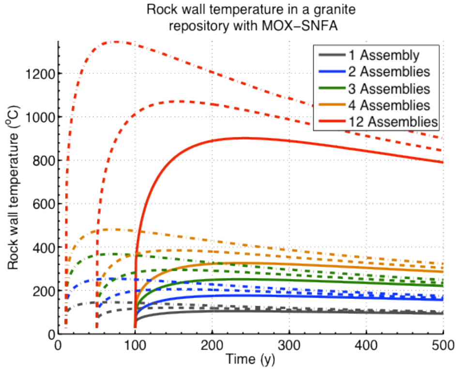
Figure H.3-2 Transient host rock temperature at the calculation radius after storage times of 10, 50 and 100 years for a waste package containing 1, 2, 3, 4 and 12 MOX assemblies in granite
