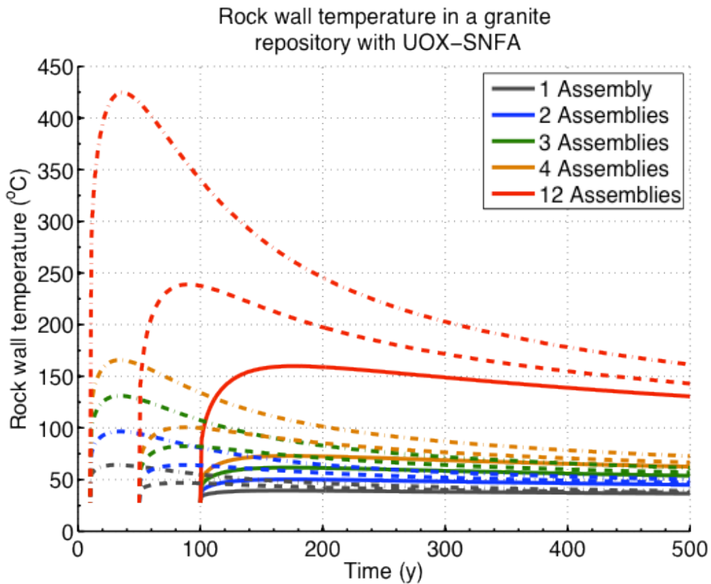
Figure H.3-1 Transient host rock temperature at the calculation radius after storage times of 10, 50 and 100 years for a waste package containing 1, 2, 3, 4 and 12 UOX assemblies in granite
