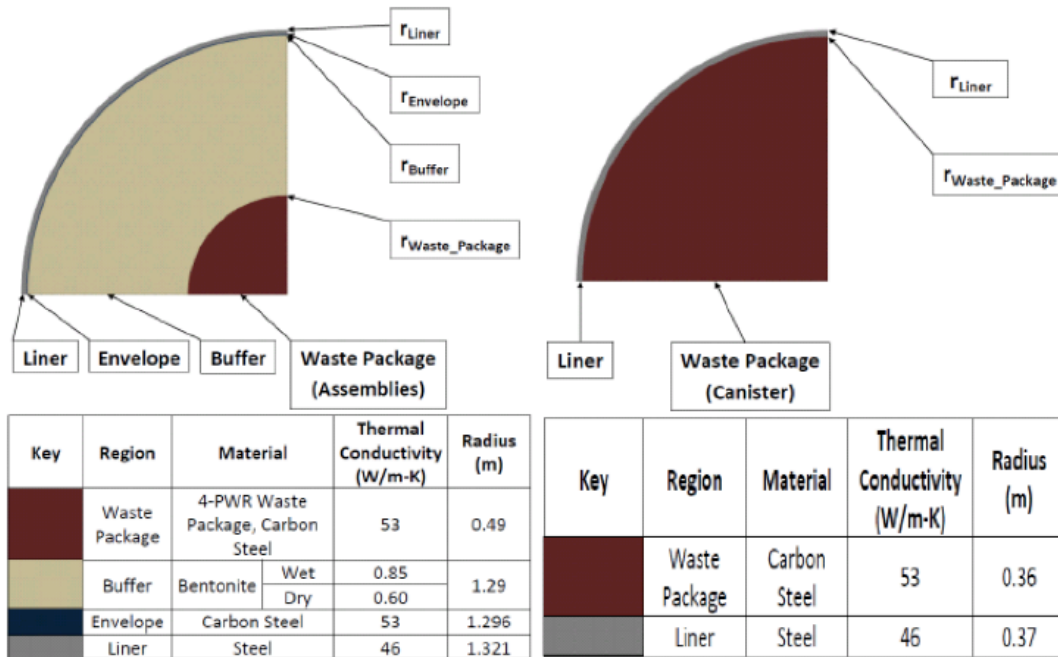
Figure 5.1-4 Graphical representation of a clay design for SNFA (left) and HLW (right), including material properties and dimensions
