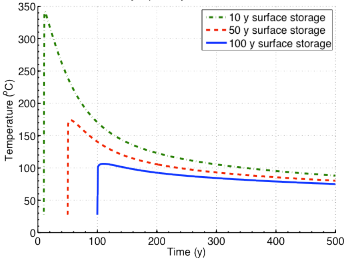
Figure H.4-7 Calculated waste package temperature after storage times of 10, 50 and 100 years for UOX-4 in clay
