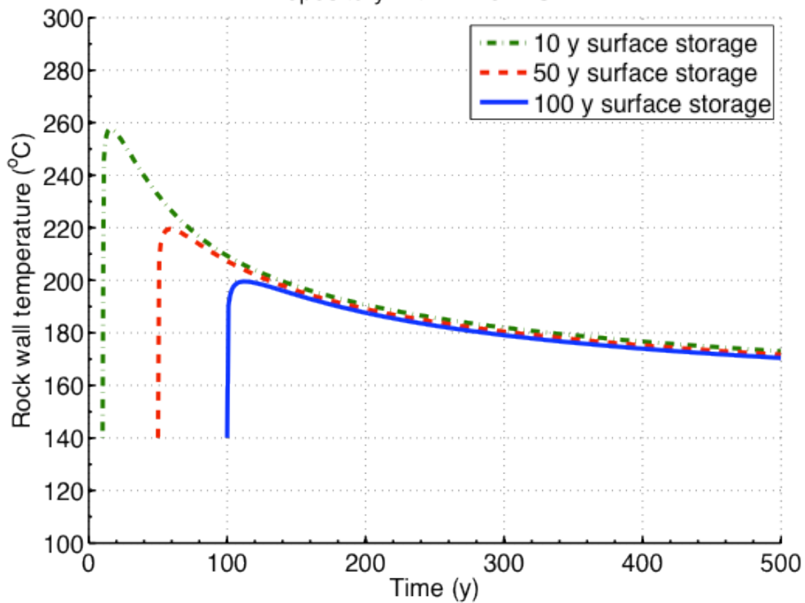
Figure H.3-20 Transient host rock temperature at the calculation radius after storage times of 10, 50 and 100 years for MOX-1 in a deep borehole
