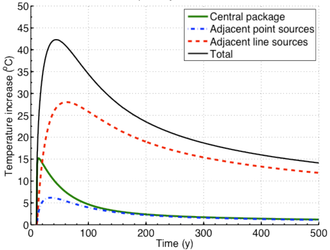
Figure H.2-13 Contributions to the transient rock temperature at the calculation radius from the central package, adjacent point sources and adjacent line sources for UOX-4 in salt
