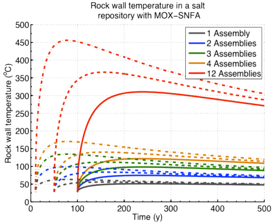
Figure H.3-14 Transient host rock temperature at the calculation radius after storage times of 10, 50 and 100 years for a waste package containing 1, 2, 3, 4 and 12 MOX assemblies in salt
