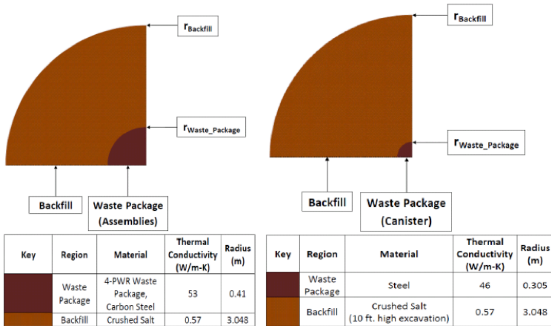
Figure 5.1-5 Graphical representation of a salt design for SNFA (left) and HLW (right), including material properties and dimensions
