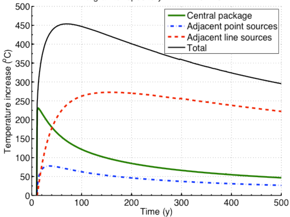
Figure H.2-2 Contributions to the transient rock temperature at the calculation radius from the central package, adjacent point sources and adjacent line sources for 4 MOX assemblies per waste package (MOX-4) in granite
