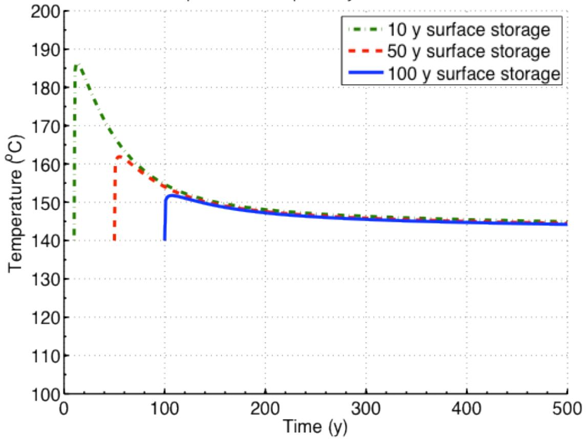
Figure H.4-19 Calculated waste package temperature after storage times of 10, 50 and 100 years for UOX-1 in a deep borehole
