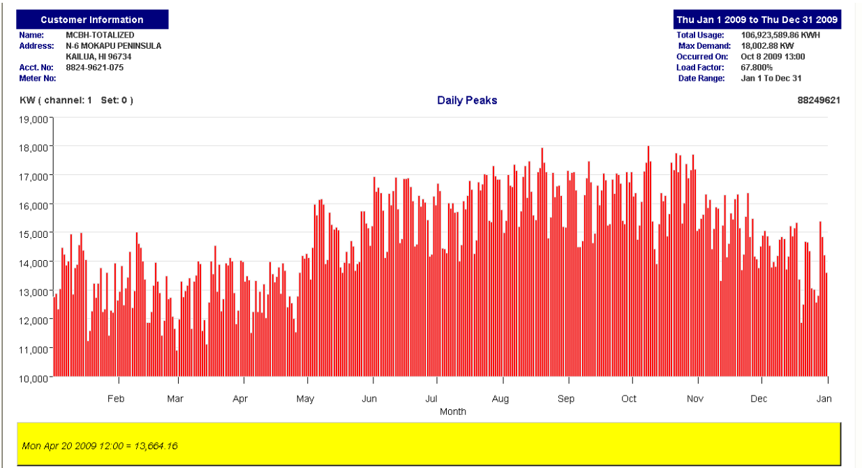
Figure 7: Annual load profile
