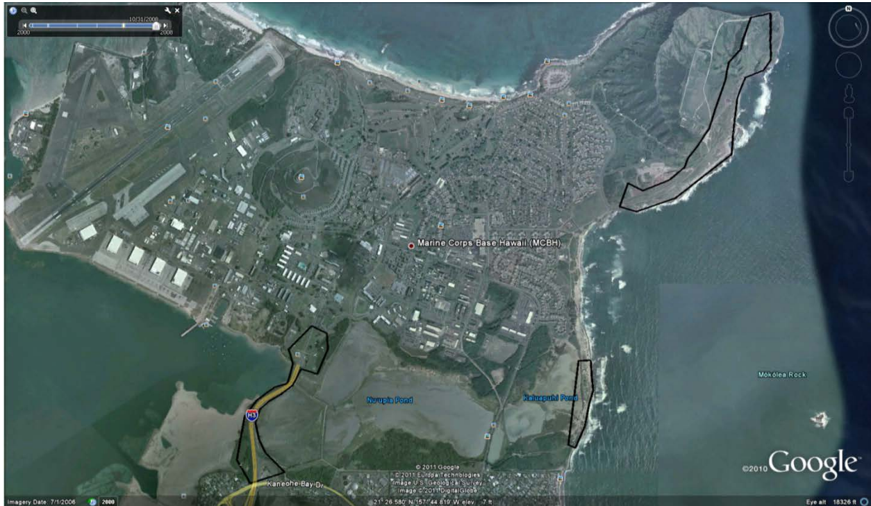
Figure 40. Potential sites for wind turbines
