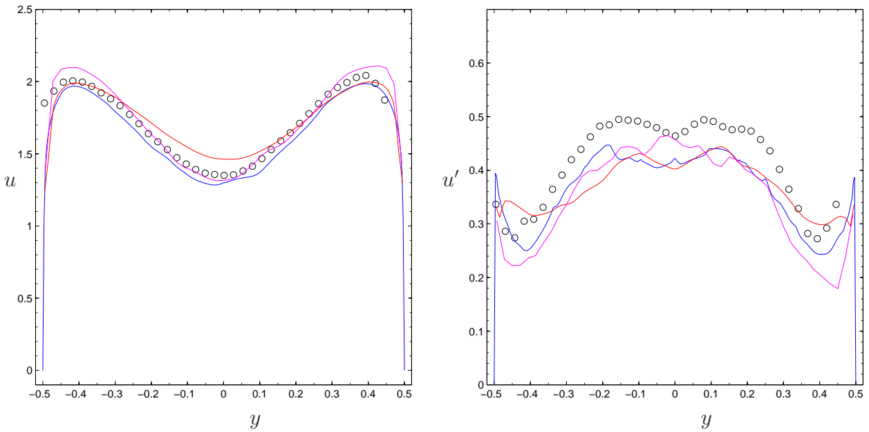
Figure 11. Axial mean velocity (left) and rms (right) horizontal profiles at x=2.6 for experimental data (circles) and simulation with Nek5000 (blue), CABARET (red), and Conv3D (magenta line).
