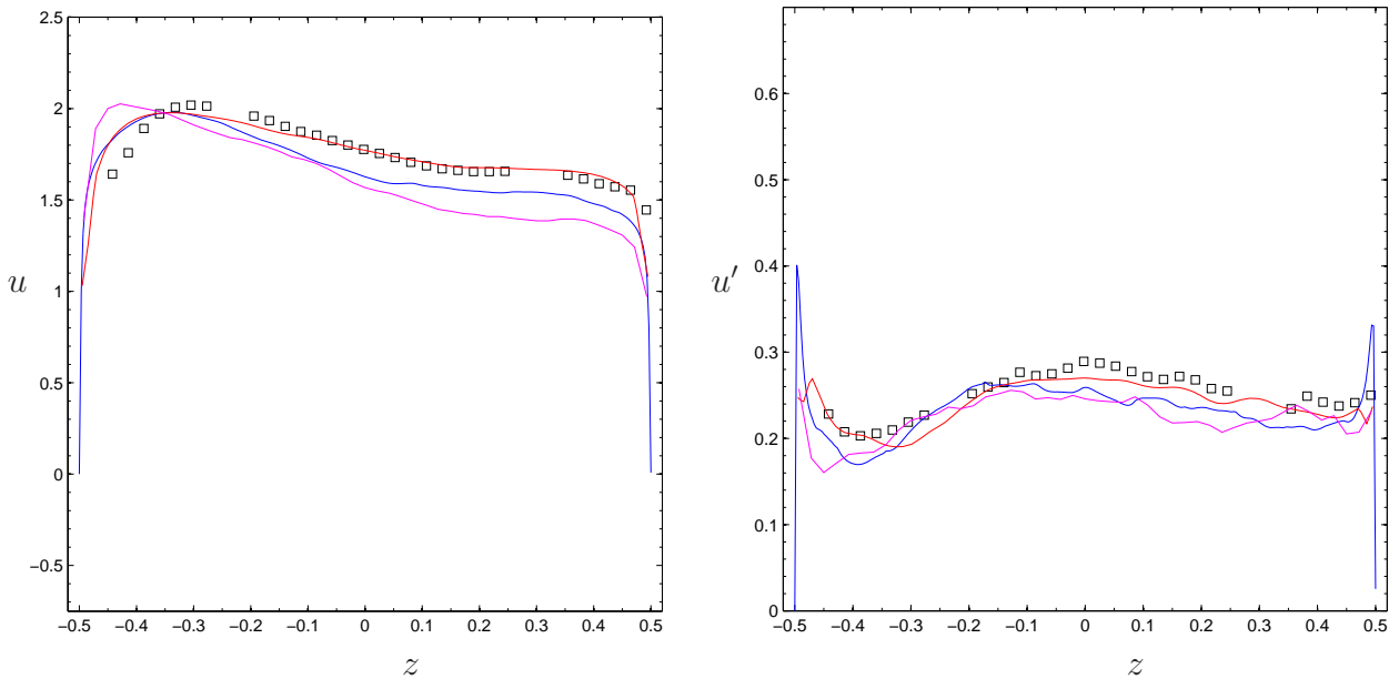
Figure 9. Axial mean velocity (left) and rms (right) vertical profiles at x=4.6 for experimental data (squares) and simulation with Nek5000 (blue), CABARET (red), and Conv3D (magenta line).
