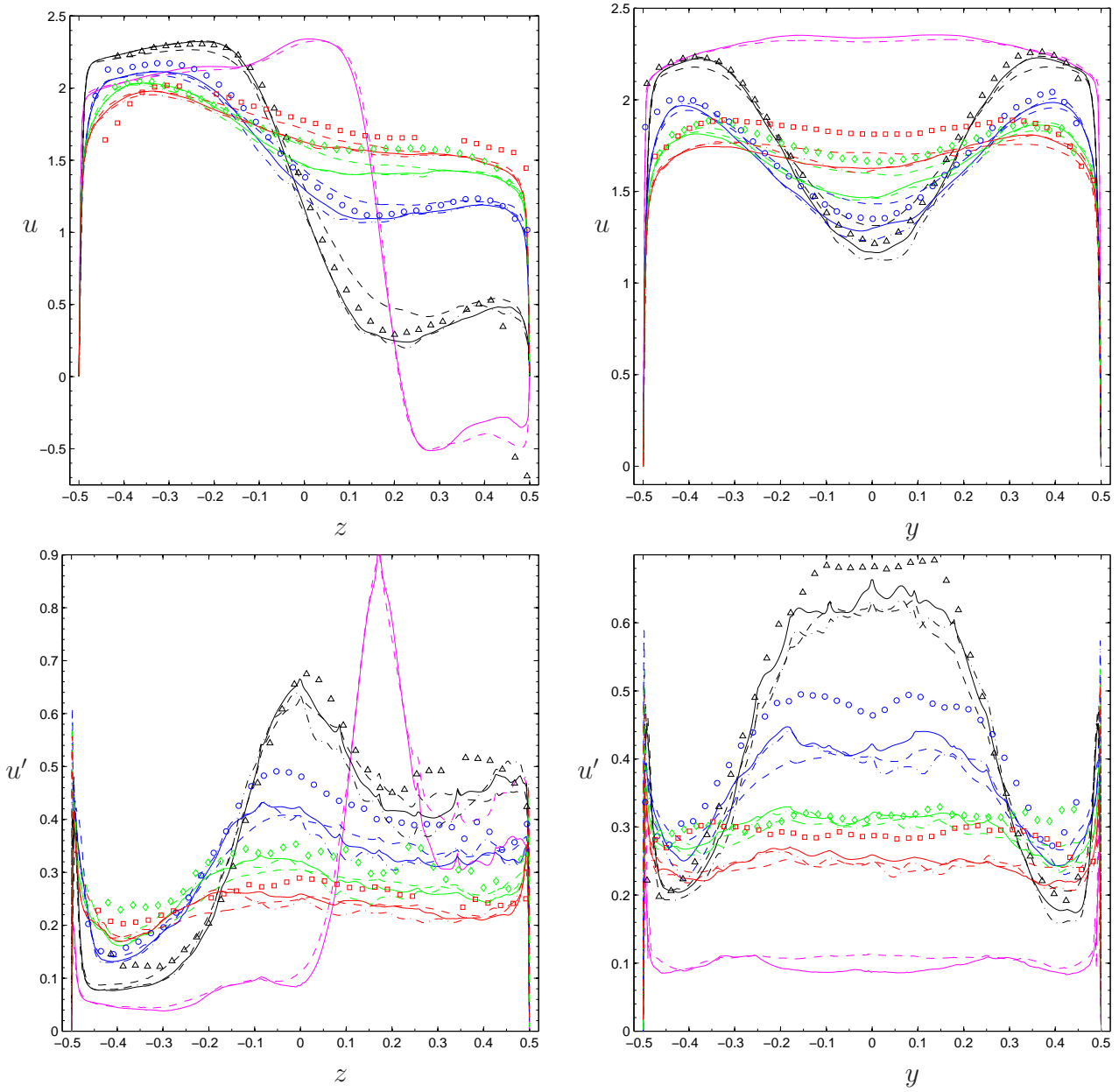
Figure 14. Vertical (left) and horizontal (right) profiles of axial mean velocity (top) and rms (bottom) profiles at x=0.6 (magenta), 1.6 (black), 2.6 (blue), 3.6 (green), and 4.6 (red) for Nek5000 simulation with N = 5 (dashed) and N = 7 (solid) and for Nek5000 benchmark submission results (dash-dot).
