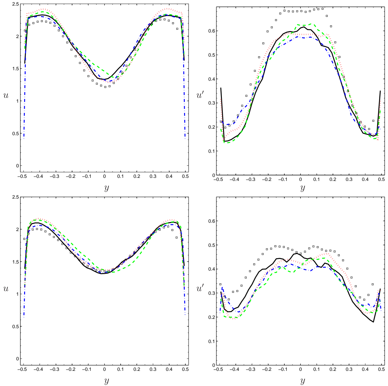
Figure 21. Horizontal profiles of axial mean (left) and rms velocity (right) at x=1.6 (top) and x = 2.6 (bottom) for the experiment data (symbols) and Conv3D simulation on 40 million node uniform (black solid) and nonuniform (blue dash-dotted) mesh, on 12 million node uniform mesh (green dashed) and on 3 million node nonuniform mesh (red dotted line).
