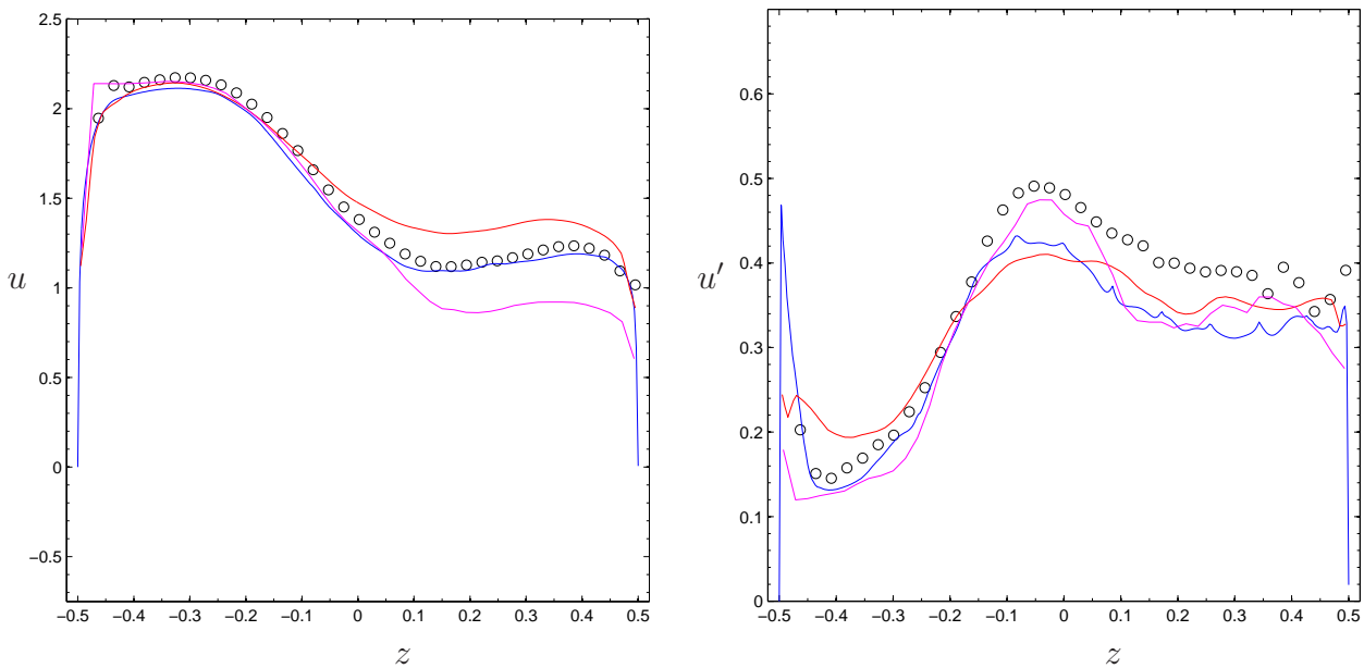
Figure 7. Axial mean velocity (left) and rms (right) vertical profiles at x=2.6 for experimental data (circles) and simulation with Nek5000 (blue), CABARET (red), and Conv3D (magenta line).
