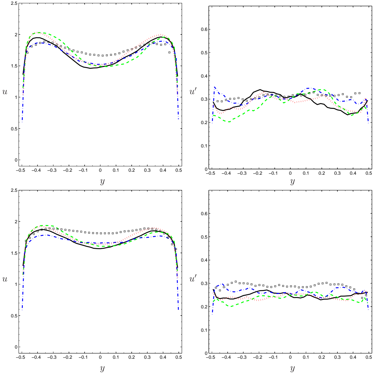
Figure 22. Horizontal profiles of axial mean (left) and rms velocity (right) at x=3.6 (top) and x=4.6 (bottom) for the experiment data (symbols) and Conv3D simulation on 40 million node uniform (black solid) and nonuniform (blue dash-dotted) mesh, on 12 million node uniform mesh (green dashed) and on 3 million node nonuniform mesh (red dotted line).
