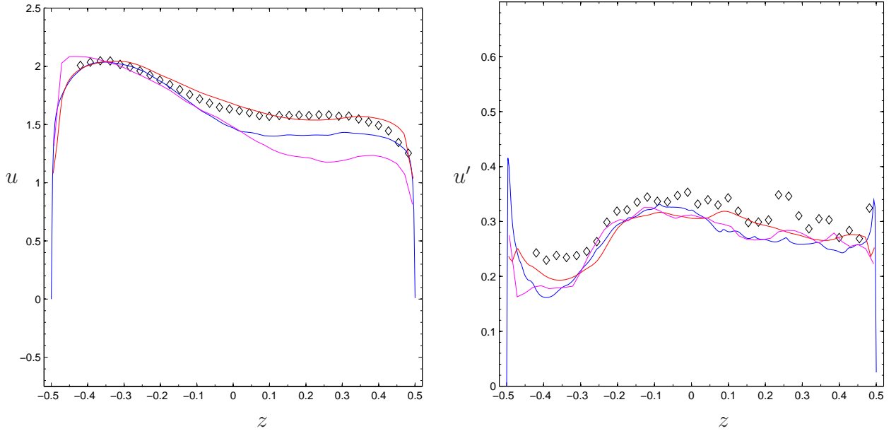
Figure 8. Axial mean velocity (left) and rms (right) vertical profiles at x=3.6 for experimental data (diamonds) and simulation with Nek5000 (blue), CABARET (red), and Conv3D (magenta line).
