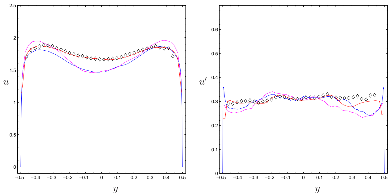
Figure 12. Axial mean velocity (left) and rms (right) horizontal profiles at x=3.6 for experimental data (diamonds) and simulation with Nek5000 (blue), CABARET (red), and Conv3D (magenta line).
