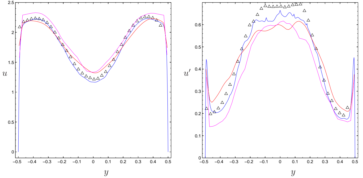
Figure 10. Axial mean velocity (left) and rms (right) horizontal profiles at x=1.6 for experimental data (triangles) and simulation with Nek5000 (blue), CABARET (red), and Conv3D (magenta line).
