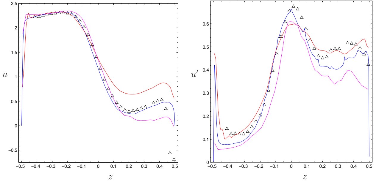
Figure 6. Axial mean velocity (left) and rms (right) vertical profiles at x=1.6 for experimental data (triangles) and simulation with Nek5000 (blue), CABARET (red), and Conv3D (magenta line).
