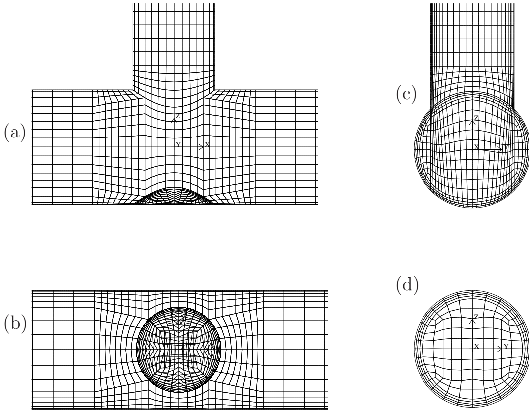
Figure 2. Computational mesh for Nek5000 T-junction simulation comprising E=62176 elements: (a) side view of surface mesh, (b) top view, (c) slice at x=0 , and (d) slice at x=4 .
