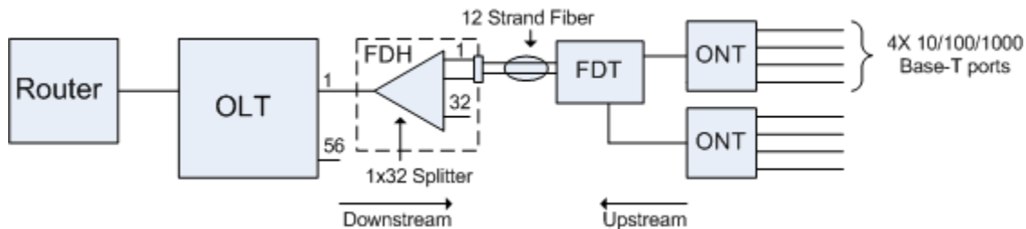
Figure 1. GPON Components
