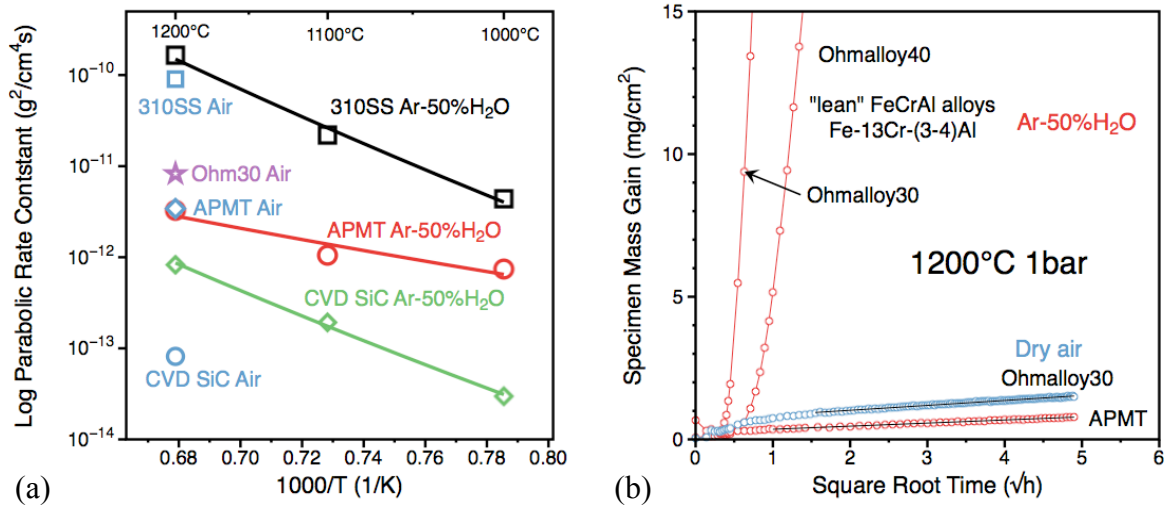
Fig. 13. (a) Arrhenius plot of the parabolic reaction rates for several materials and (b) comparison of mass gain for FeCrAl alloys at 1200°C in Ar-50%H 2 O and dry air.
