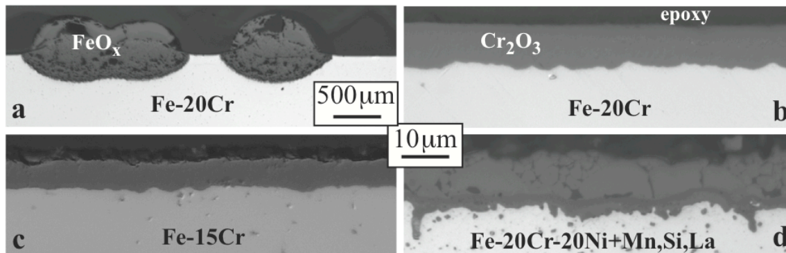
Fig. 16. Light microscopy of polished cross-sections of after exposure for 2h at 1200°C in 3.4bar steam (a) and (b) Fe-20Cr, (c) Fe-15Cr and (d) Fe-20Cr-20Ni+Mn,Si,La.
