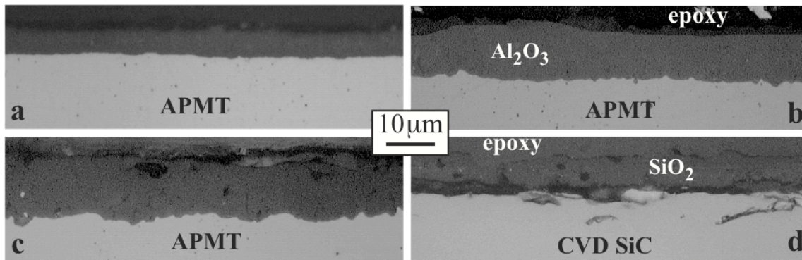
Fig. 4. Light microscopy of polished cross-sections of APMT after exposure in 3.4 bar steam for (a) 48h at 1200°C, (b) 8h at 1300°C and (c) 8h at 1350°C and (d) CVD SiC after 8h at 1350°C.
