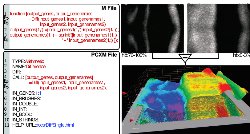
Fig. 3. M-file (top left) and PCXM header file (bottom left) of an example function for the computation of the cell-by-cell difference between two expression patterns. Color of text is used to illustrate which parts are mandatory (red), optional (blue), or provided in a template file (black). Right: Example showing the use of the function to compute the difference between late- and early-stage hunchback expression.
